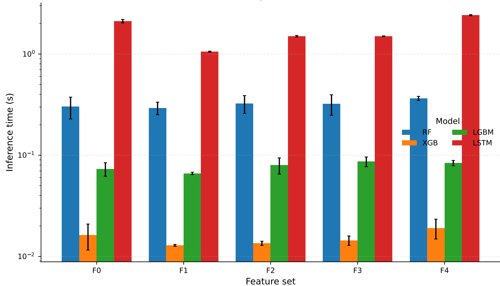
Inference time (s) by model and feature set
