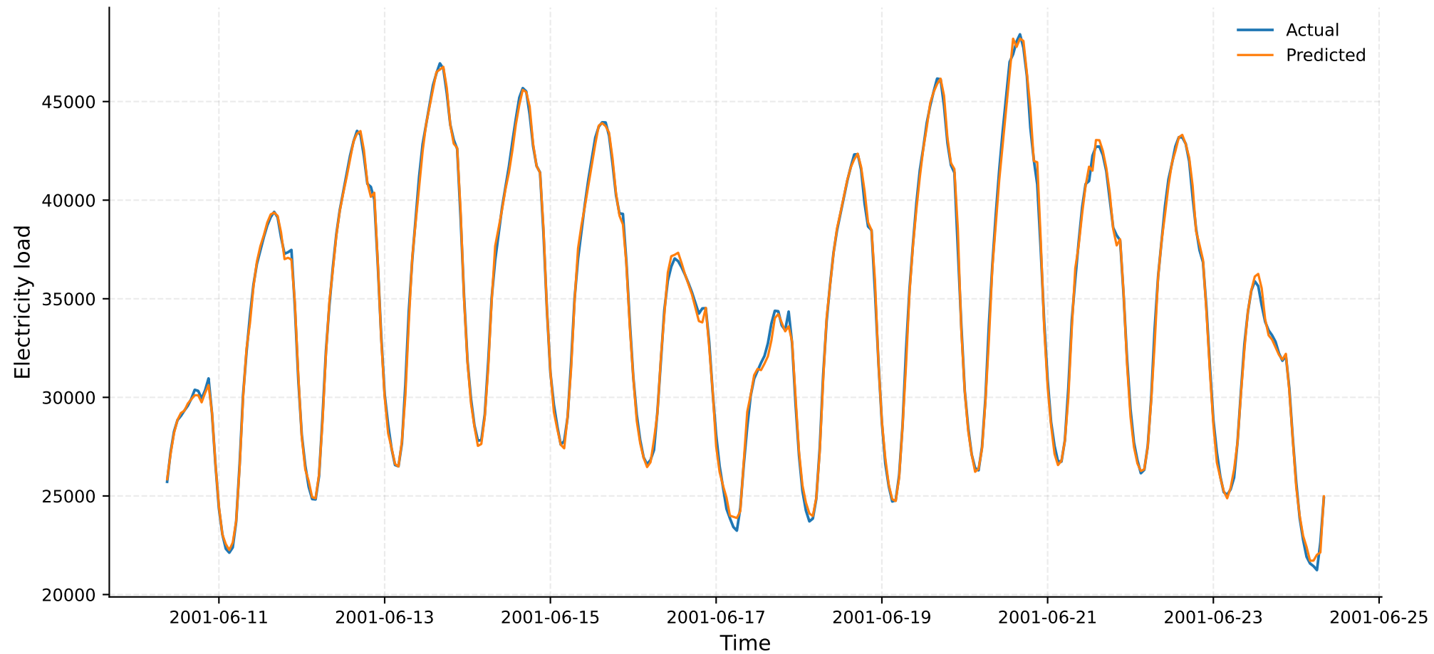
Best run: LSTM-F3, seed 168 (RMSE=326.18)
