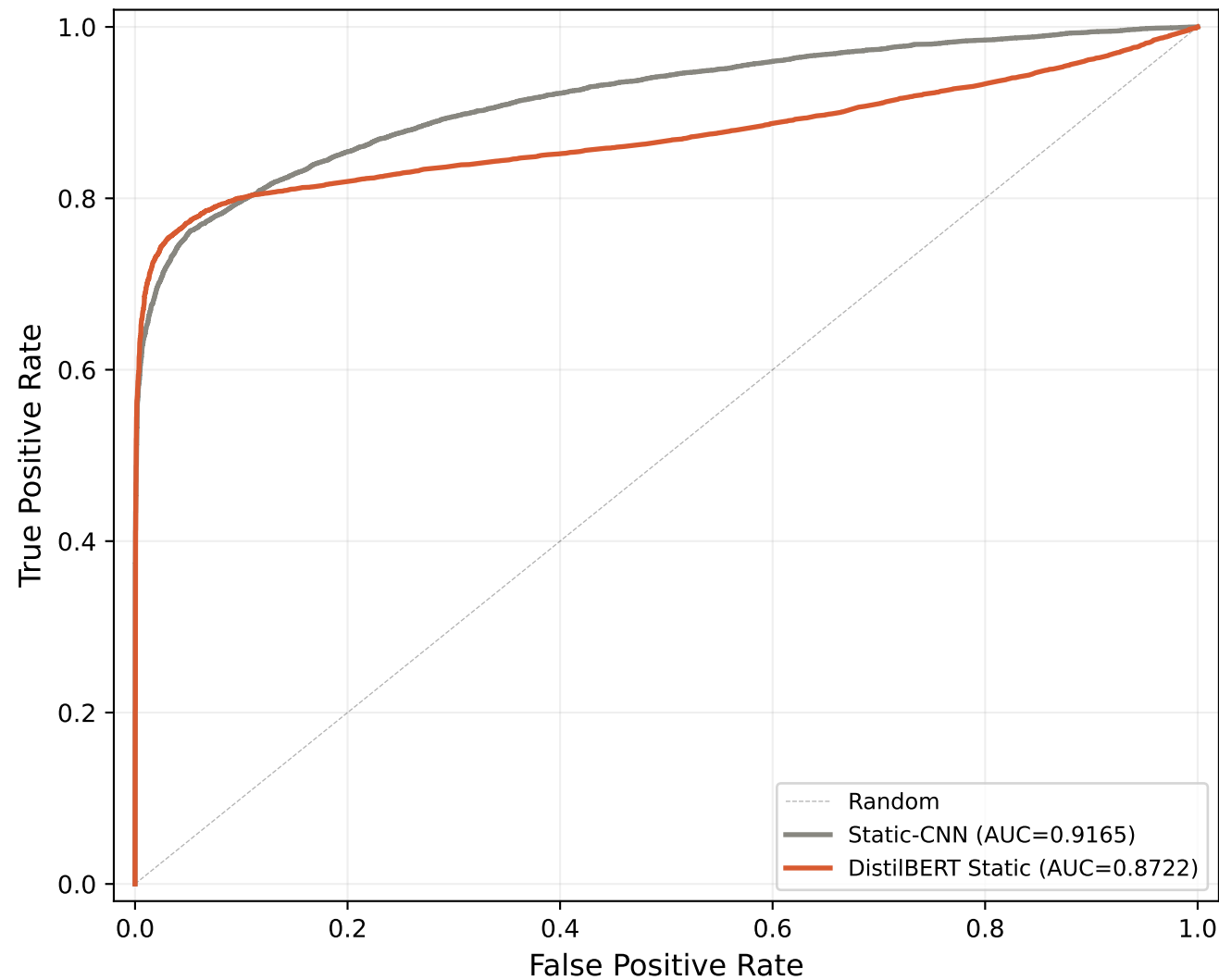
(a) ROC Curve (D24 test)
