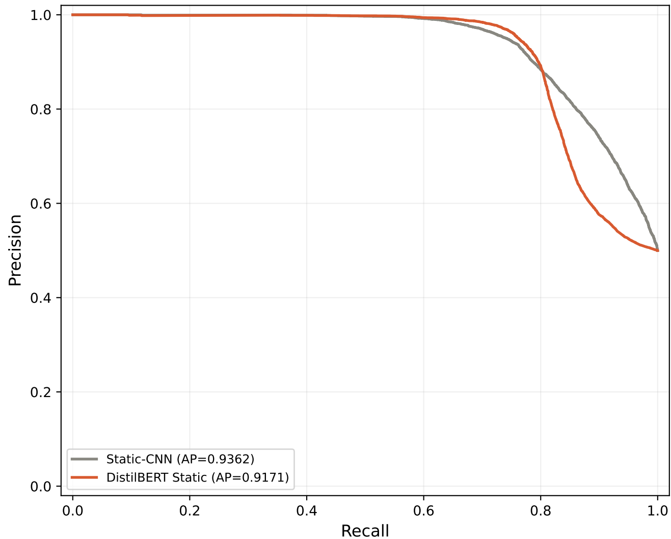
(b) Precision-Recall Curve (D24 test)
