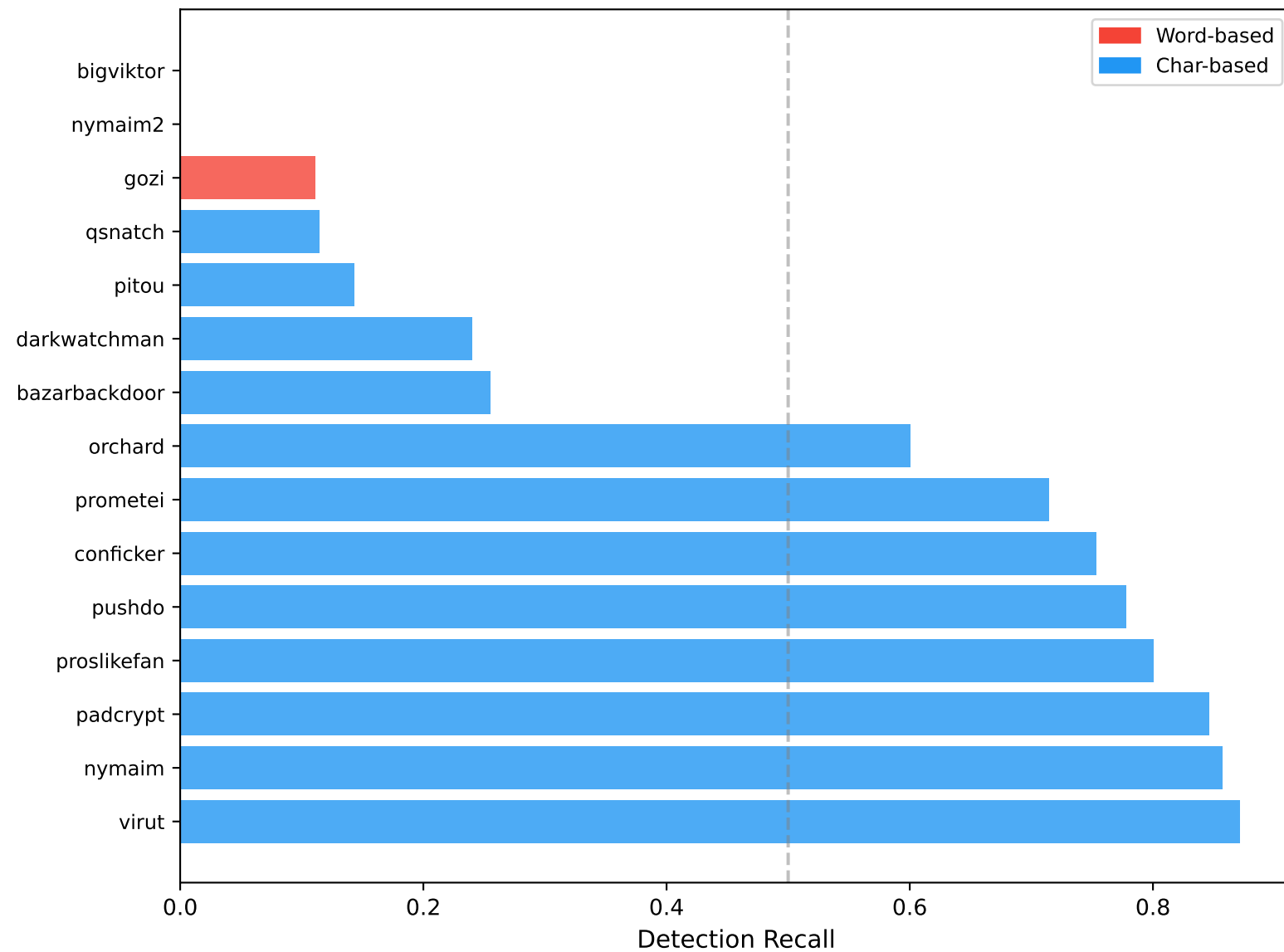
(a) 15 Worst-Detected Families (Static-CNN on D24)
