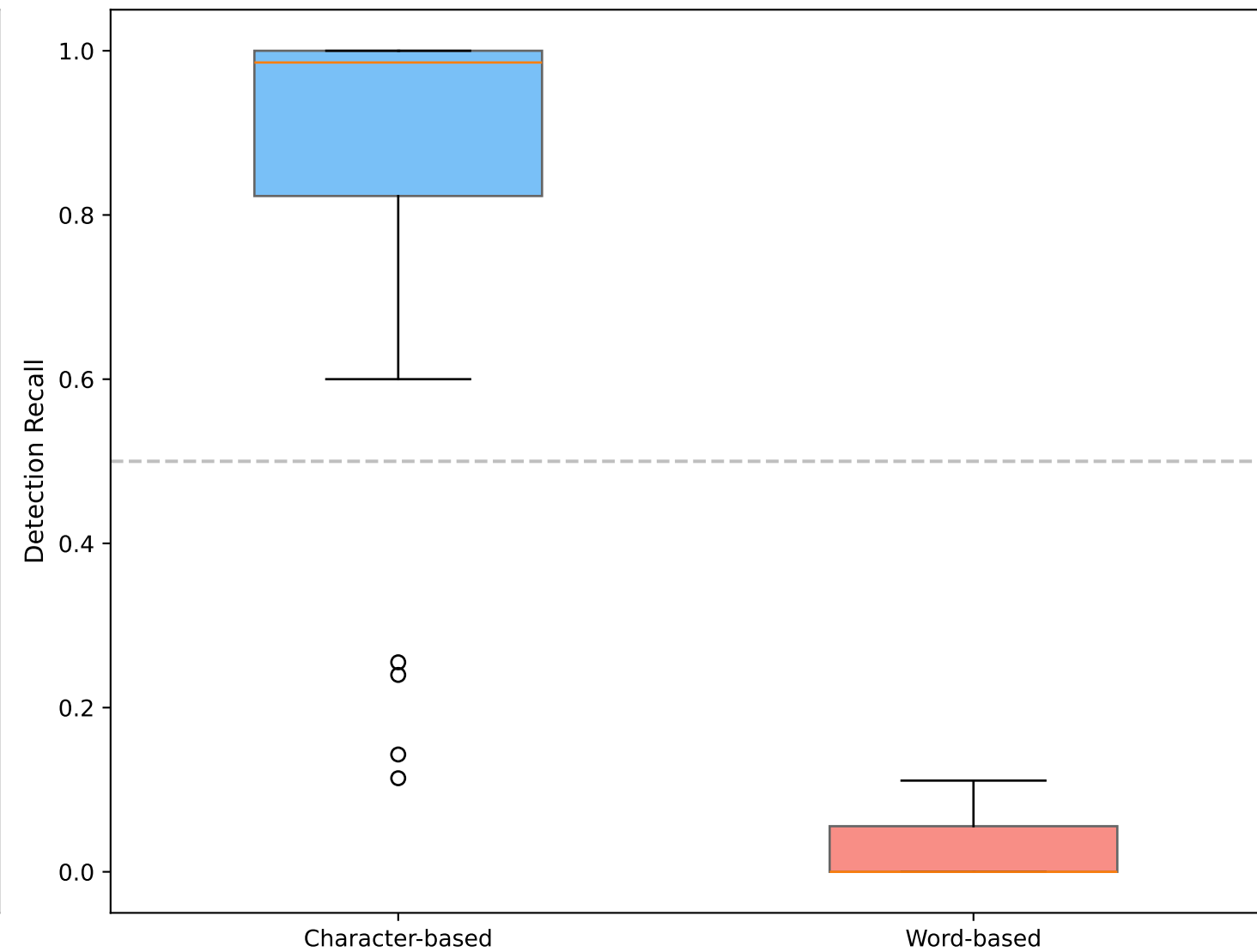
(b) Recall Distribution by DGA Type (Static-CNN on D24)
