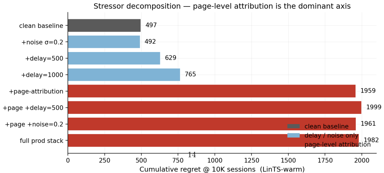
Figure 5: Figure 2: Stressor decomposition. LinTS-warm cumulative regret at 10K sessions under each
