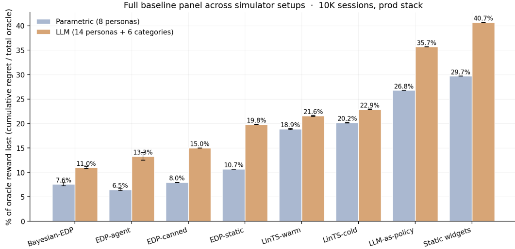
Figure 7: Full baseline panel across simulators. Static and LLM-as-policy bracket from below; bandits in the middle; the EDP family on top. Bayesian-EDP is best on LLM-persona (11.0%); EDP-agent is best on parametric (6.5%). Error bars are \pm 1 SE across replicates.
