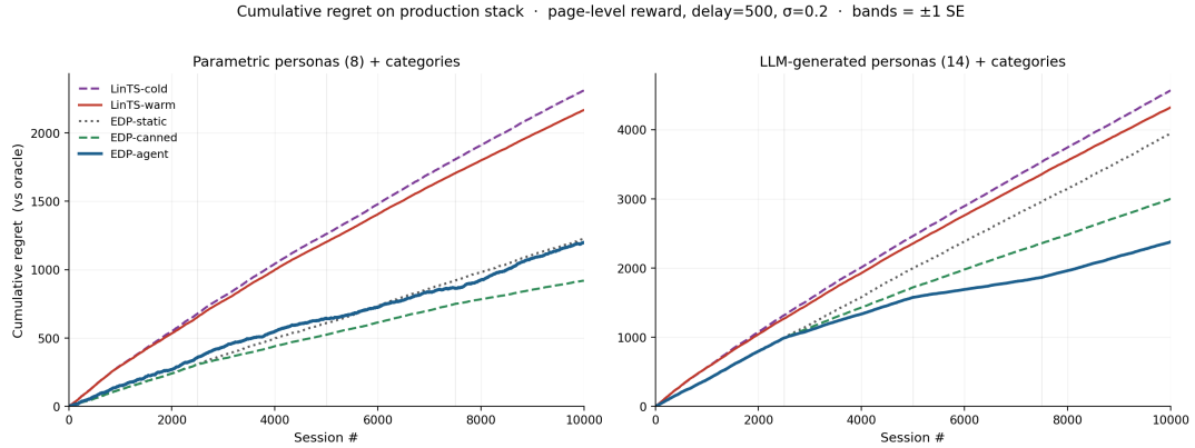
Figure 6: Cumulative regret over 10K sessions on each simulator. Left: parametric (8 personas). Right: LLM (14 personas + categories). EDP-agent stays low across both; EDP-static / EDP-canned degrade visibly from left to right; LinTS is high in both.
