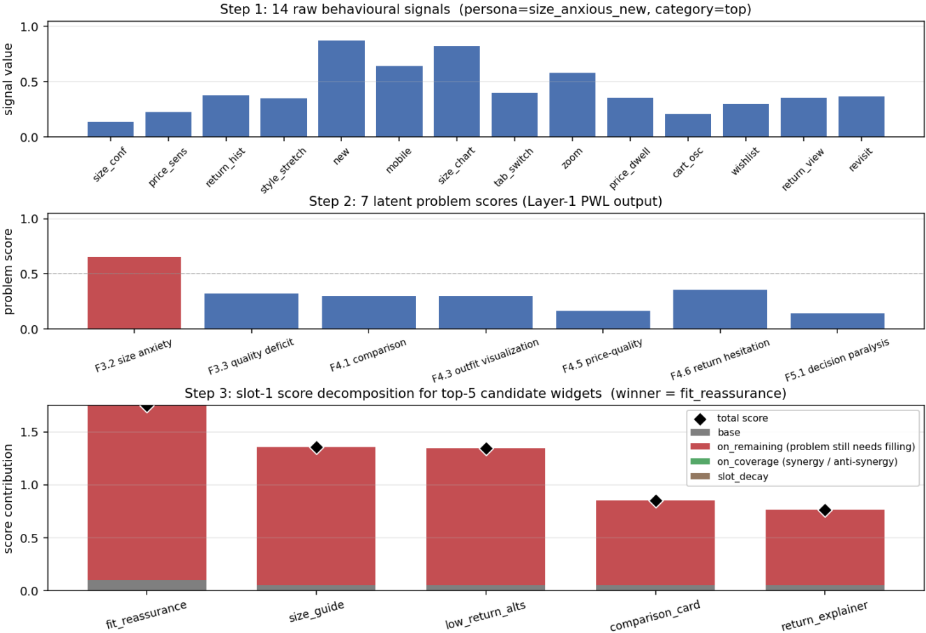
Figure 2. Figure 9: Open-box decision trace for one size-anxious session. Top: the 14 raw behavioural signals. Middle: the 7 Layer-1 problem scores. Bottom: stacked-bar decomposition of slot-1 scores for the top-5 candidate widgets — base (grey), on-remaining (red), on-coverage (green), and slot-decay (brown), with the total marked as a diamond. The winner wins for readable reasons.
