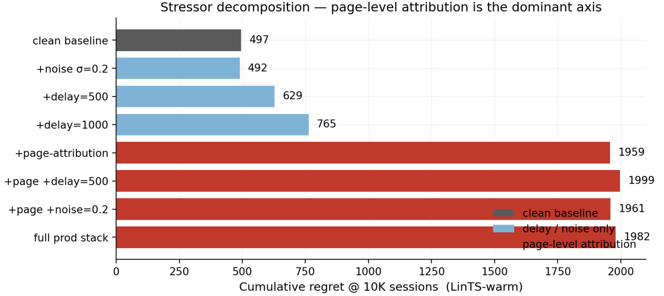
Figure 6. Figure 2: Stressor decomposition. LinTS-warm cumulative regret at 10K sessions under each combination of (per-slot vs page-level attribution) \times (delay \in \{0, 500, 1000\} ) \times (noise \sigma \in \{0, 0.2\} ).
