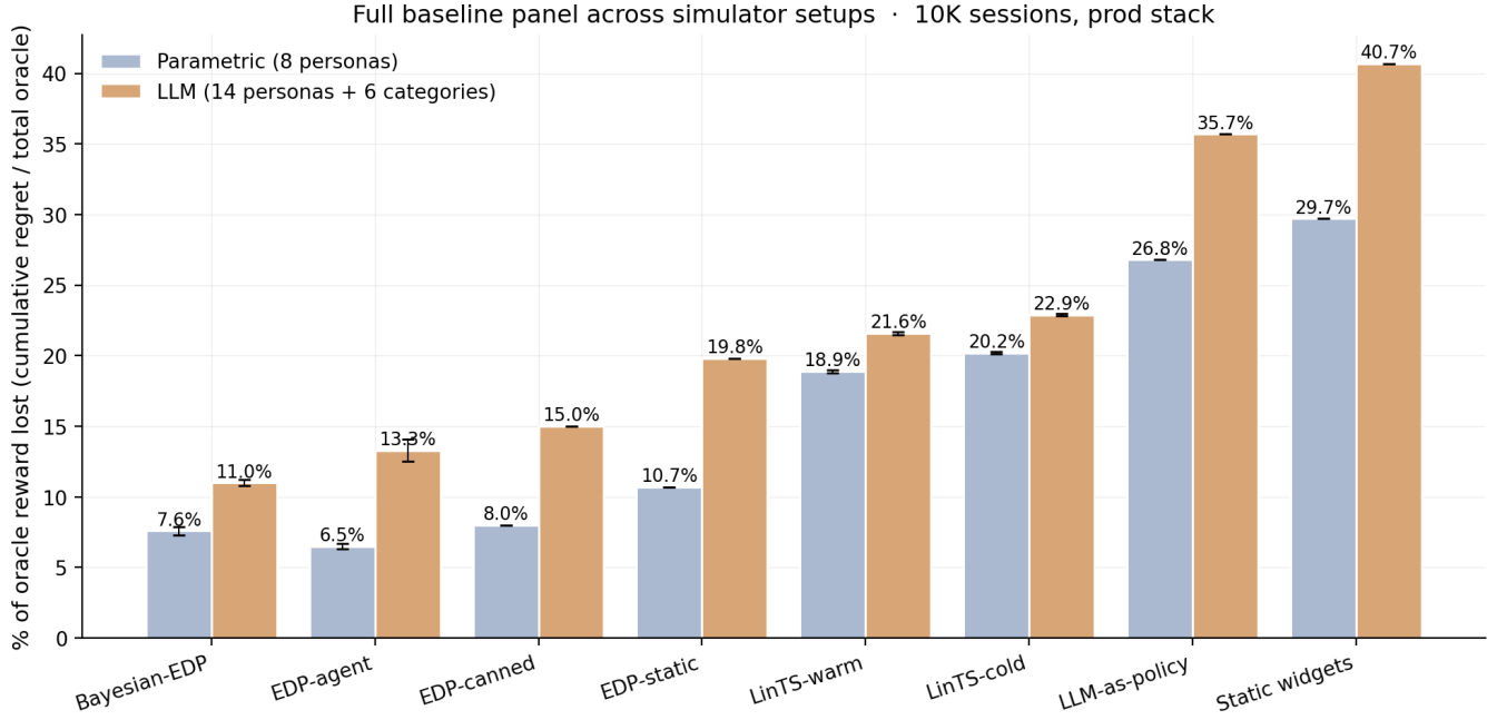
Figure 7. Figure 7: Full baseline panel across simulators. Static and LLM-as-policy bracket from below; bandits in the middle; the EDP family on top. Bayesian-EDP is best on LLM-persona (11.0%); EDP-agent is best on parametric (6.5%). Error bars are \pm 1 SE across replicates.
