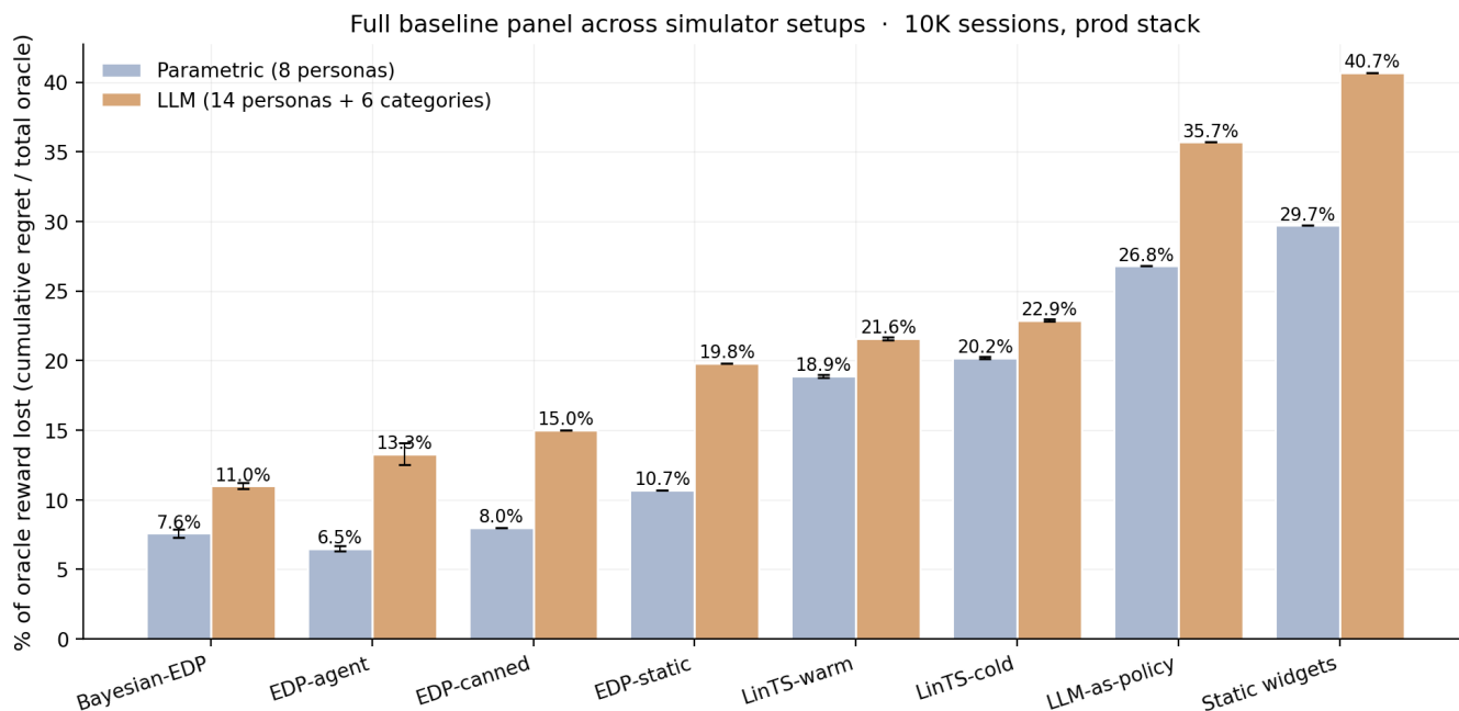
Figure 11. Figure 7: Full baseline panel across simulators. Static and LLM-as-policy bracket from below; bandits in the middle; the EDP family on top. Bayesian-EDP is best on LLM-persona (11.0%); EDP-agent is best on parametric (6.5%). Error bars are \pm 1 SE across replicates.
