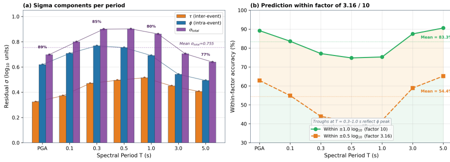
Fig. 8. Residual sigma decomposition. (a) Inter-event ( \tau , orange), intra-event ( \phi , blue), and total sigma ( \sigma_{total} , purple) per spectral period, with the mean \sigma_{total} = 0.755 line shown. Percentages annotate the intra-event dominance ratio \phi/\sigma_{total} which ranges 77–89%. (b) Within-factor accuracy: fraction of predictions within factor 10 ( \pm 1.0 \log_{10} , green) and within factor 3.16 ( \pm 0.5 \log_{10} , orange), averaging 83.3% and 54.4% respectively across periods.
