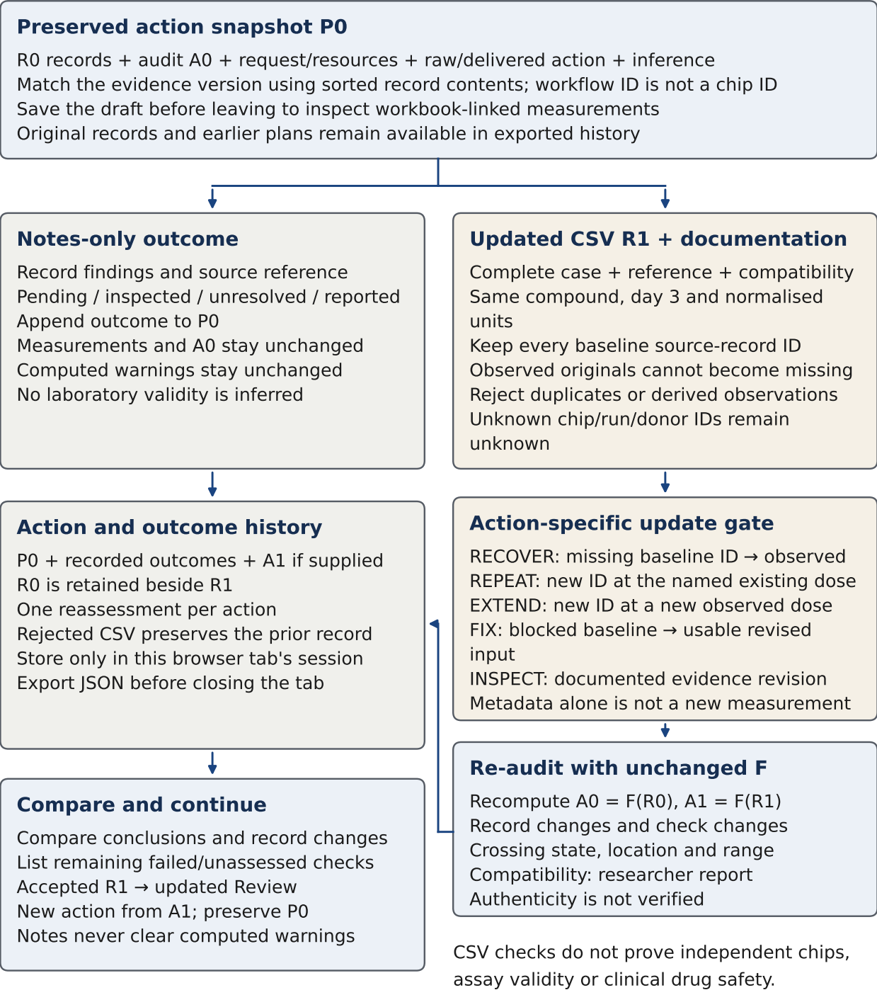
Figure 3. Notes document a decision; a compatible CSV starts a separate evidence version
