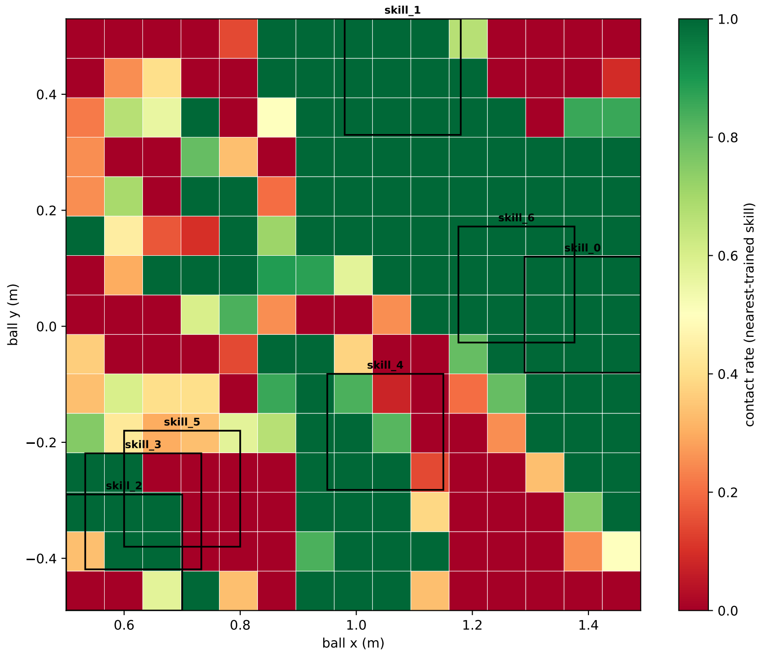
Ball-placement contact-rate heatmap (15x15 bins, 1500 placements, nearest-trained skill of 7, overall 56.1%)
