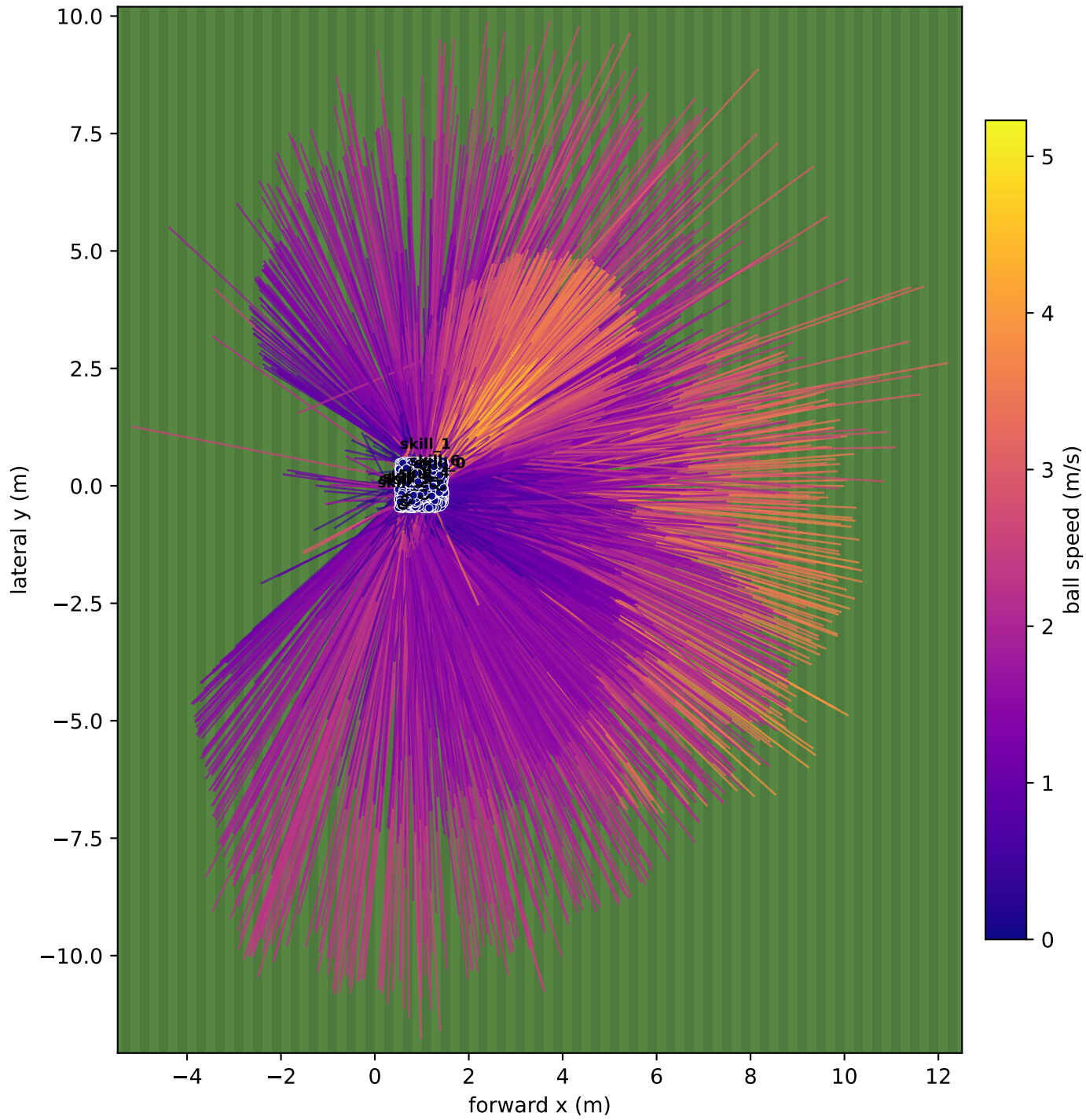
Shot trajectories across swept ball placements (ALL contacts, incl. non-directed touches, 4549 drawn)
