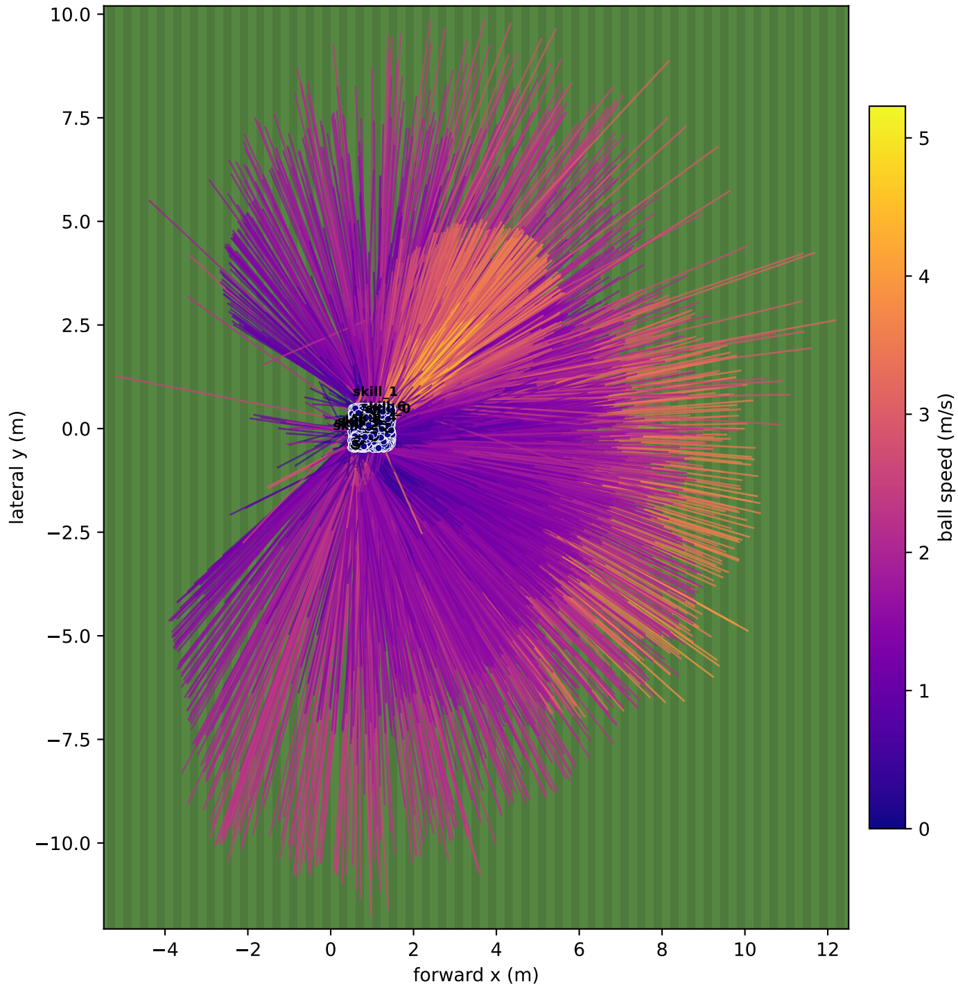
Shot trajectories across swept ball placements (ALL contacts, incl. non-directed touches, 5641 drawn)
