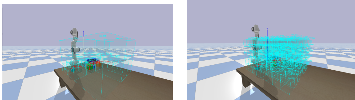
(a) Semantic partition: cyan Free Space Boxels where the scene is empty, plus object and shadow Boxels at the cube cluster.
