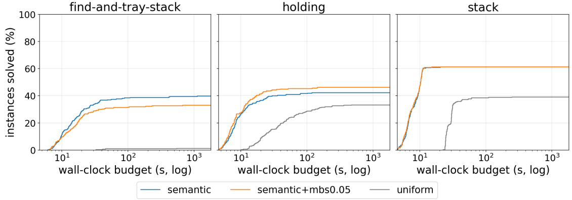
Figure 5.4: Cumulative solve rate vs wall-clock budget (log axis) per (goal, variant). Almost all solves happen within \sim 200 s; uniform starts later and plateaus lower on every goal.
