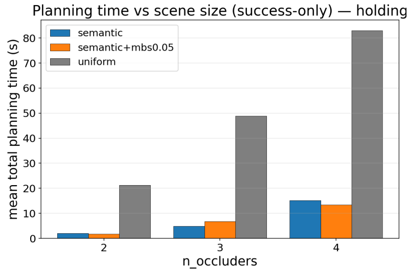
Figure 5.8: Mean success-only planning time vs n_{\text{occ}} on the holding goal. Adaptive variants scale gracefully; uniform’s cost grows much faster.
