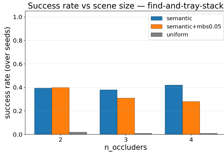
Figure 5.7: Success rate vs n_{\text{occ}} on the find-and-tray-stack goal. Uniform fails almost entirely; semantic+mbs0.05 visibly degrades with n_{\text{occ}} , contrary to its intent.
