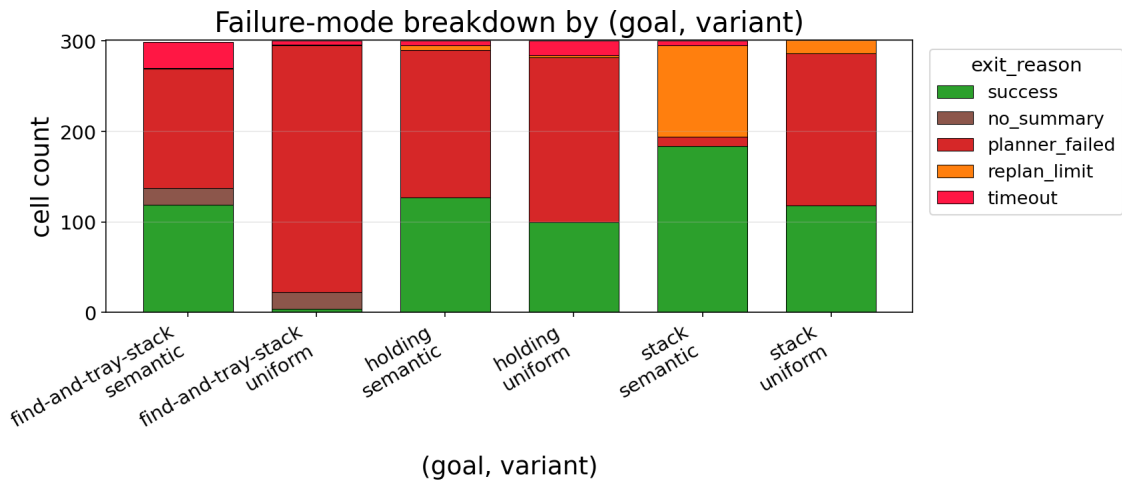
Figure 5.12: Stacked exit-reason breakdown per (goal, variant). planner_failed here also absorbs the physics_mismatch , drop_failed and all_searched exits (all cases where the planned solution ultimately failed); it is the dominant failure mode on holding and find-and-tray-stack, while on stack the semantic variant instead fails mainly via replan_limit (the second-largest slice after success).
