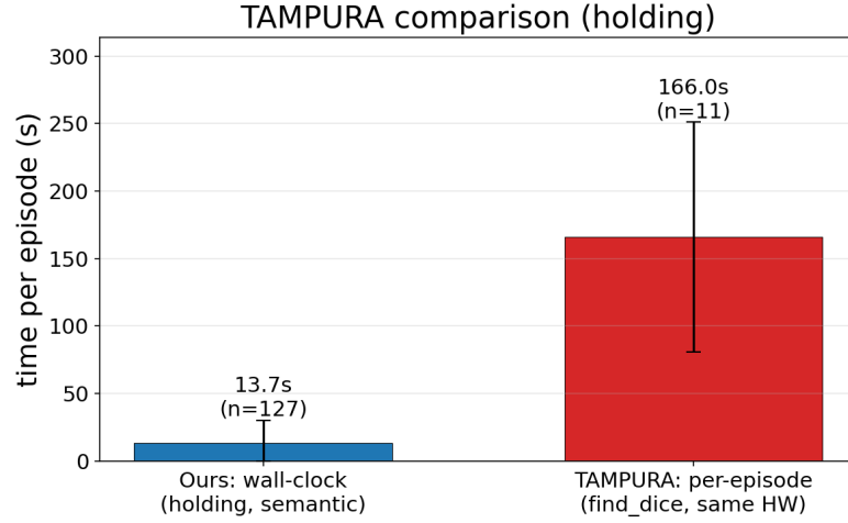
Figure 5.11: Per-episode time on holding (same hardware): our wall-clock (semantic variant; mean \pm std, success-only; right-skewed, median 8.5 s) and real TAMPURA Find Die re-run locally (mean \pm std over successful episodes; 20 seeds, 55 % success). Both are per-episode times including simulated execution. TAMPURA’s published 57 s (Table II) is a per-step figure and is not plotted; see the text for the per-step reconciliation. On reliability the order reverses, holding-semantic succeeding on 42 % of episodes against TAMPURA’s local 55 %.
