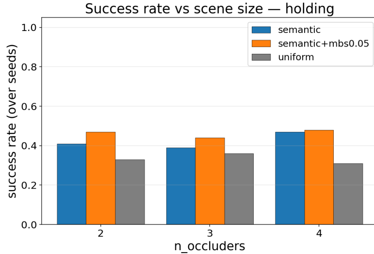
Figure 5.5: Success rate vs n_{\text{occ}} on the holding goal. Adaptive variants (semantic, semantic+mbs0.05) are within seed noise of each other; uniform sits \sim 10 pp lower. Each bar is the mean success rate over the \sim 80 – 100 seeds at that difficulty (here and in Figures 5.6 and 5.7).
