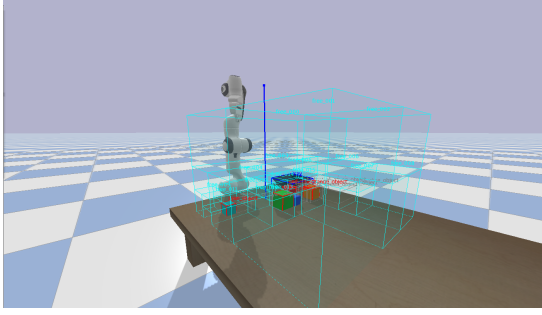
(a) Semantic partition: cyan Free Space Boxes where the scene is empty, plus object and shadow Boxels at the cube cluster.
