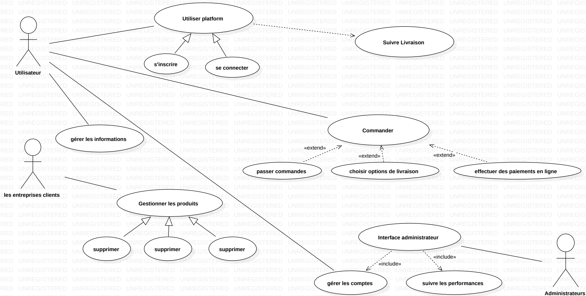
Model1::UseCaseDiagram1
