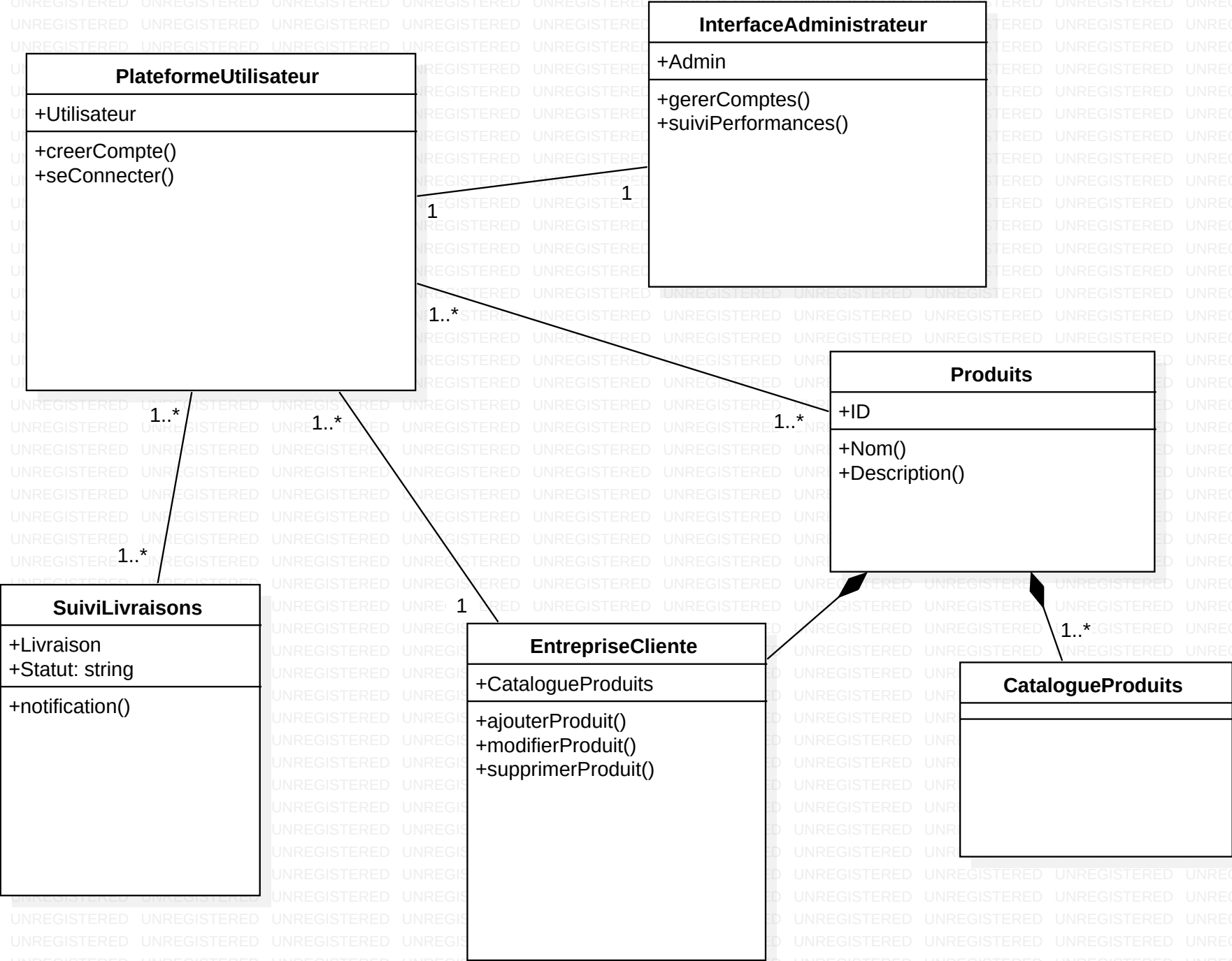
Model2::ClassDiagram1
