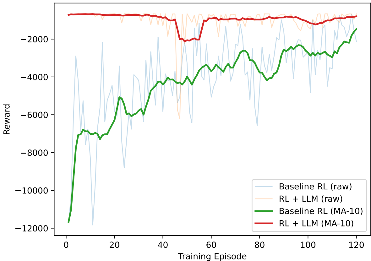
TRAIN Episode Reward
