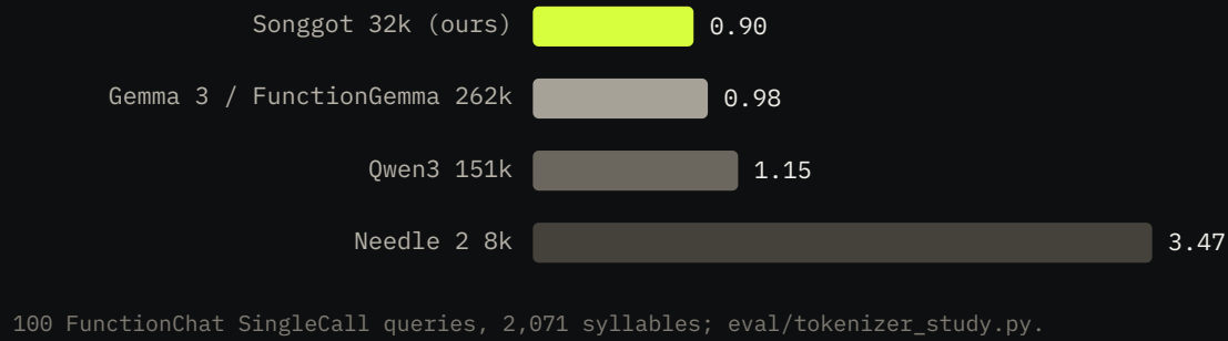
Figure 1. Tokens per Hangul syllable on the FunctionChat queries, lower is better
