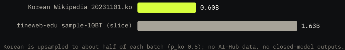
Figure 4. Pretraining corpus in tokens under the Songgot tokenizer
