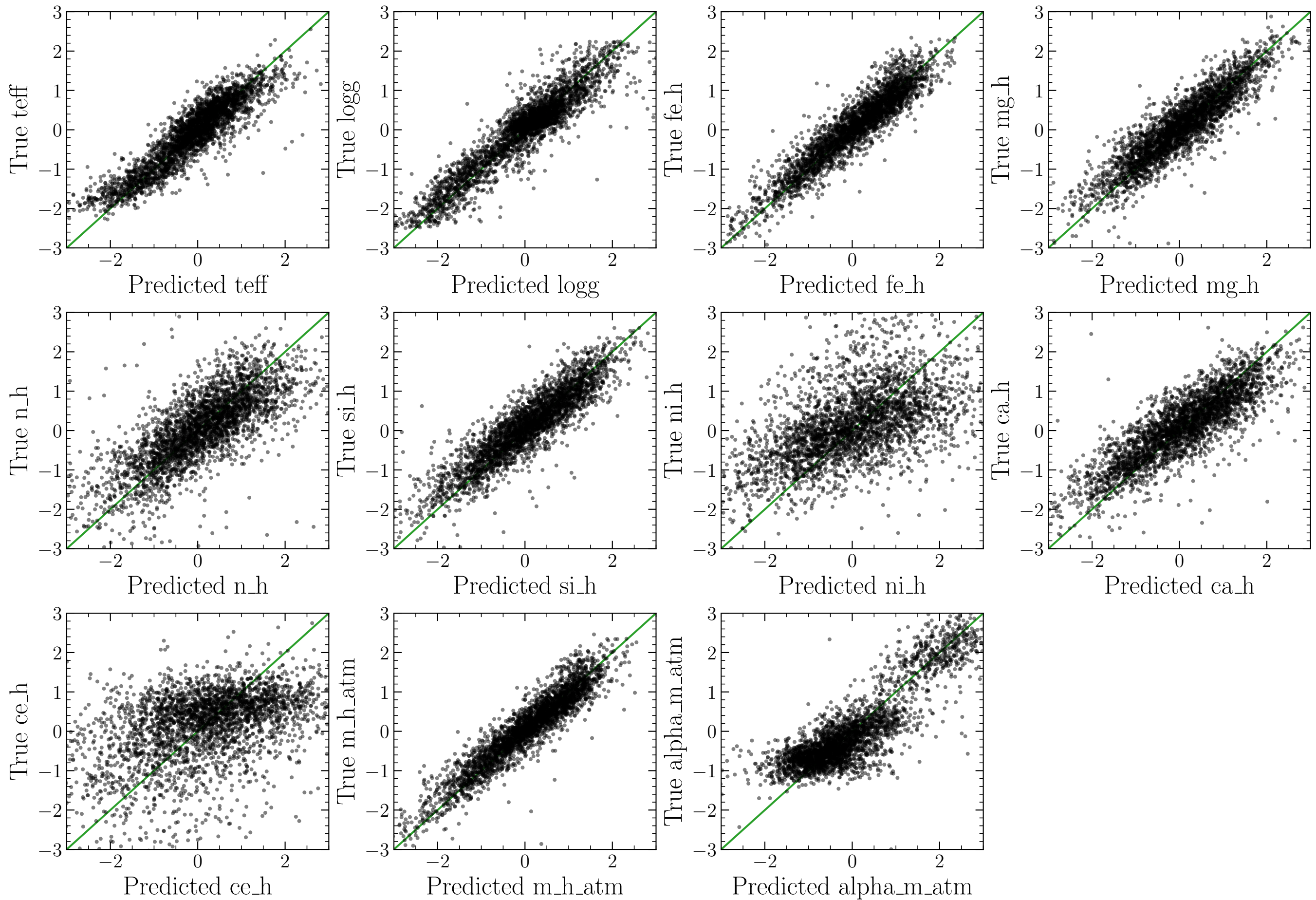
Flux only: predicted vs. true labels, giants, no mask, n_latents = 11
