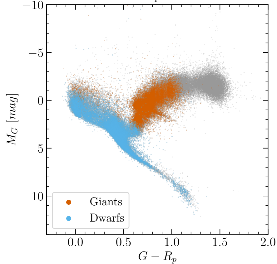
Gaia stars with RVS spectra and SNR > 100
