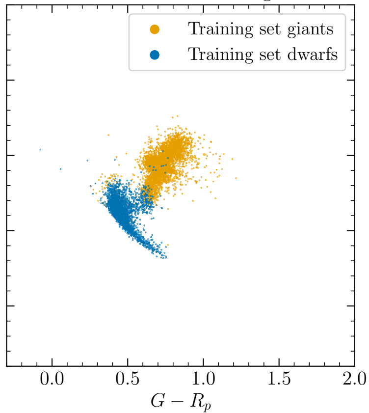
Gaia stars in the training set
