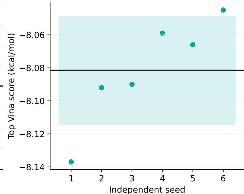
PDE9A canonical
