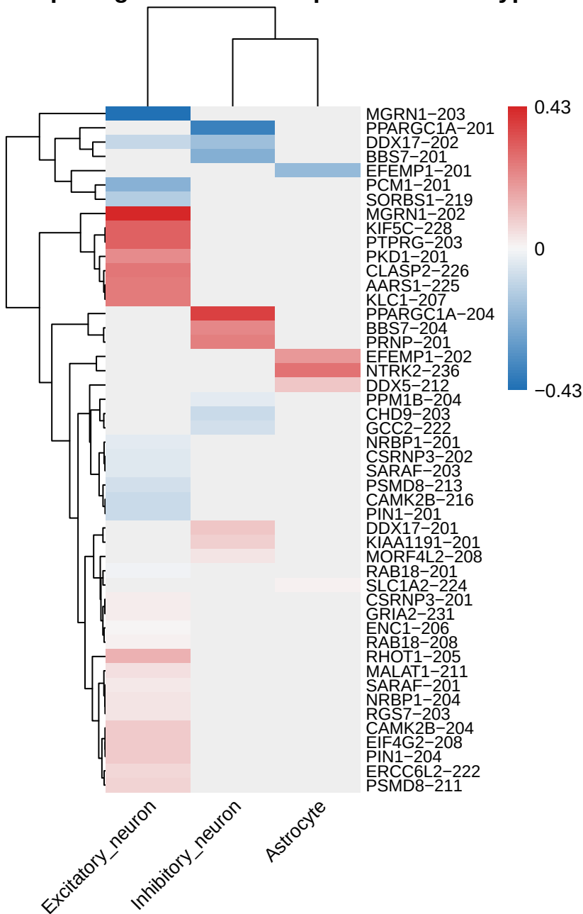
.PSI heatmap - significant transcripts across cell types
