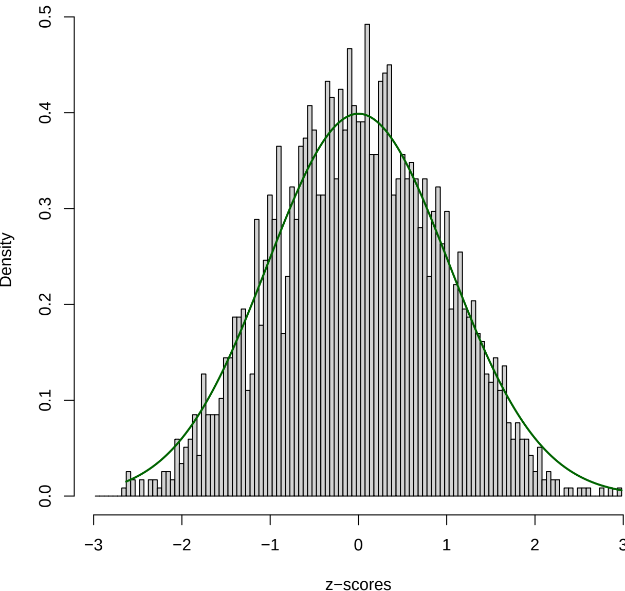
diagplot 2: AD_vs_Control
