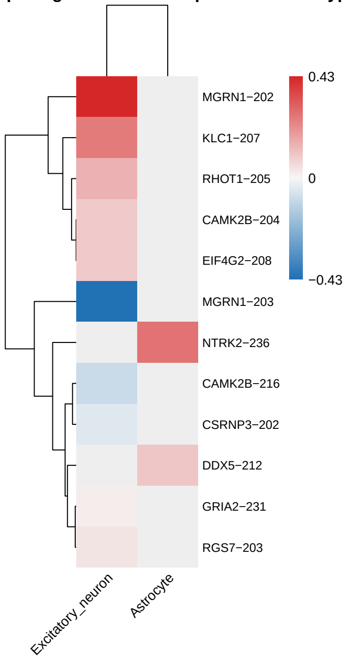
.PSI heatmap – significant transcripts across cell types
