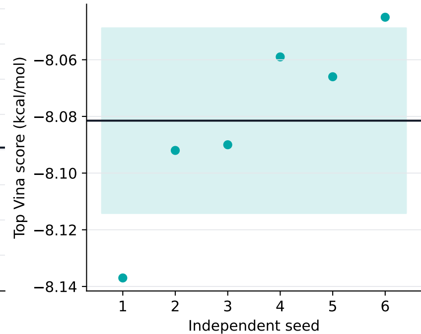
PDE9A canonical
