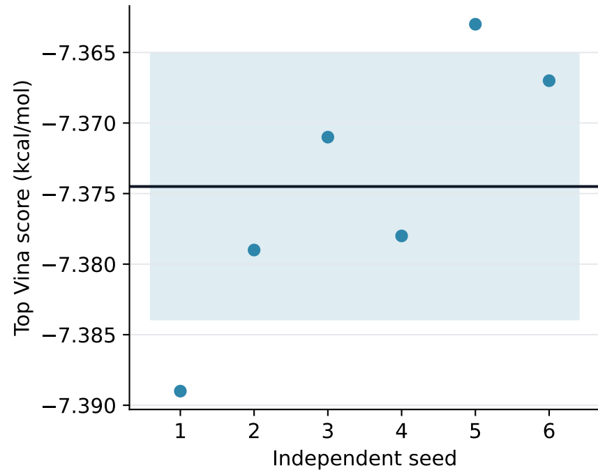
GABRA2 canonical
