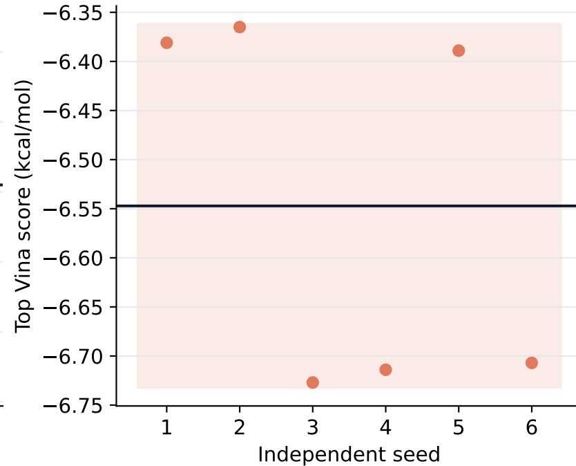
CACNA1D shared pocket
