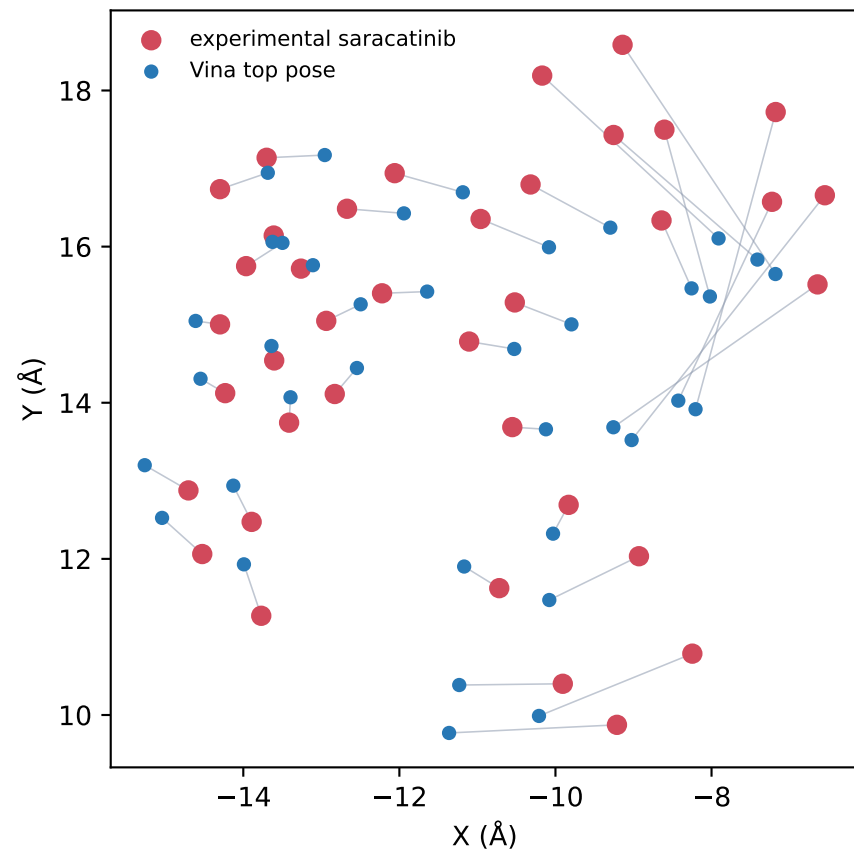
10Dj ligand overlay RMSD = 1.75 Å
