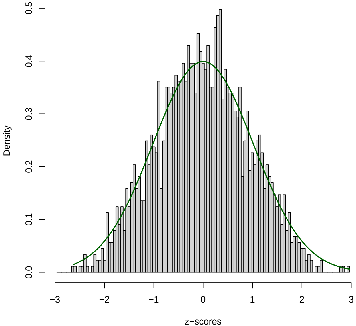
diagplot 2: AD_vs_Control
