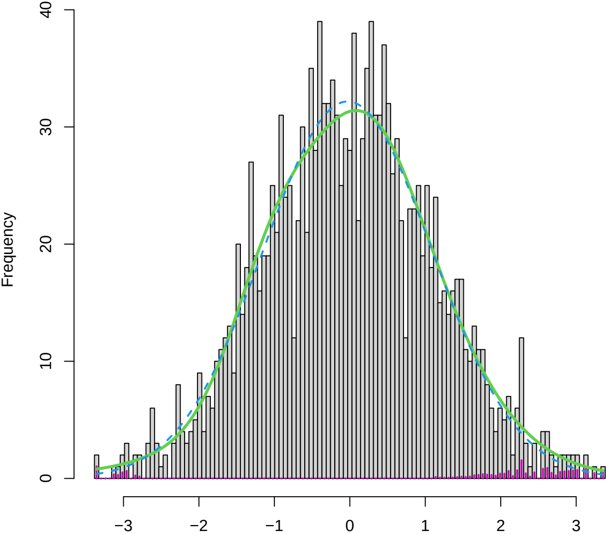
diagplot 1: AD_vs_Control
