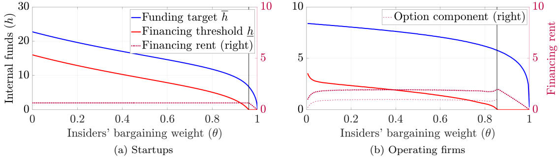
Figure 6: Comparative statics in bargaining power \theta
