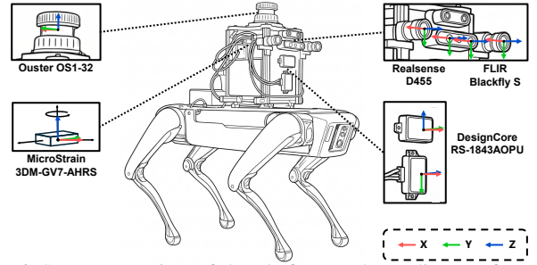
Fig. 6: System overview of the platform and coordinates of sensors.
