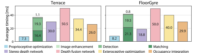
Fig. 11: Average runtime of RAGNAROK-SLAM in ms per frame.
