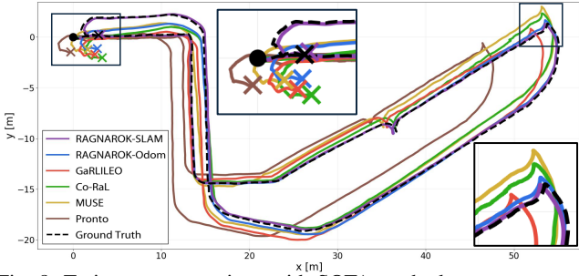
Fig. 8: Trajectory comparison with SOTA methods on Overpass.
