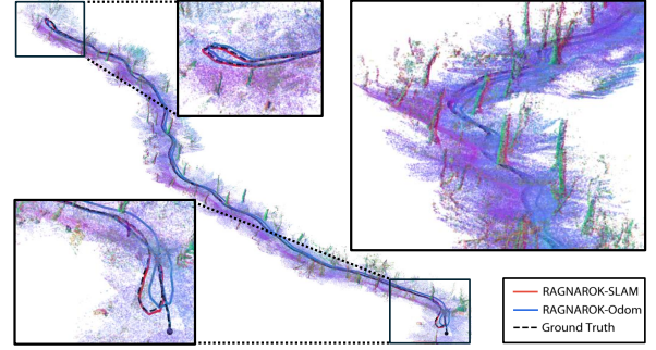
Fig. 7: Reconstructed map of Mountain-Long with trajectories.
