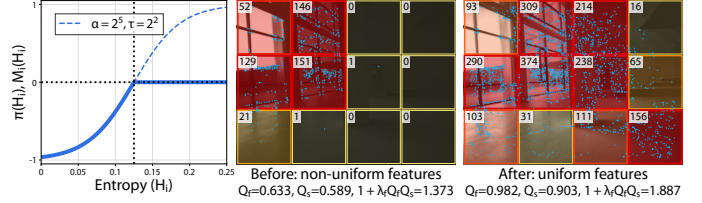
Fig. 4: Left: Plot of \pi(H_i) M_i(H_i) . Middle: Before enhancement, features are non-uniformly distributed. Right: After enhancement, more features are extracted and more uniformly distributed.
