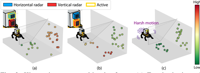
Fig. 3: Kinematics-aware multi-radar factor. (a) For the horizontal radar, wall points aligned with the azimuth are weighted higher. (b) For the vertical radar, floor and ceiling points aligned with the azimuth are weighted higher. (c) Under harsh motion, increased positional uncertainty lowers the radar Doppler residual weights.
