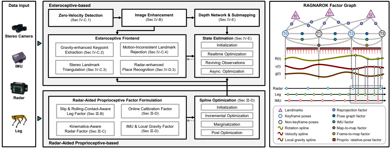
Fig. 2: Overview of RAGNAROK: The radar-aided proprioceptive estimator optimizes the splines of velocity, rotation, and local gravity. The exteroceptive estimator performs image enhancement, keypoint matching, landmark triangulation, place recognition, and submapping.
