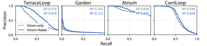
Fig. 10: Precision-recall curves for sequences with multiple loops.
