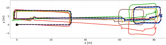
Fig. 9: Trajectory comparison with SOTA methods on Downstair.
