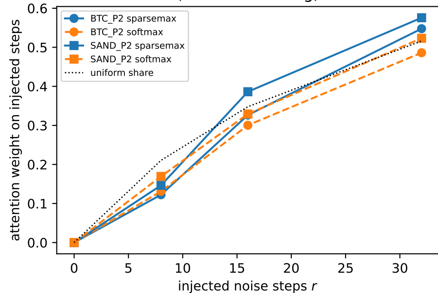
(a) Sparsemax does not exclude injected noise (after full training)
