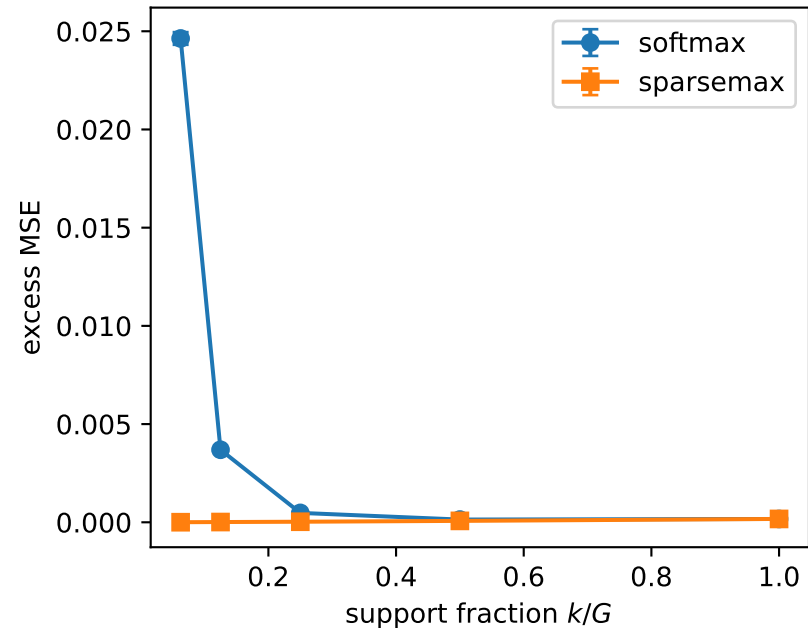
(a) n = 512, \sigma_z = 1
