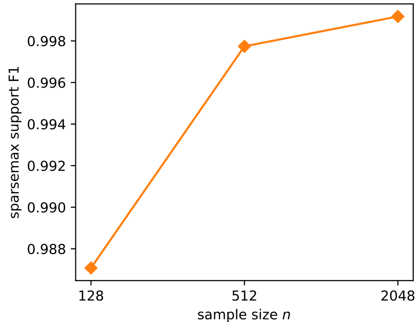
(c) support recovery
