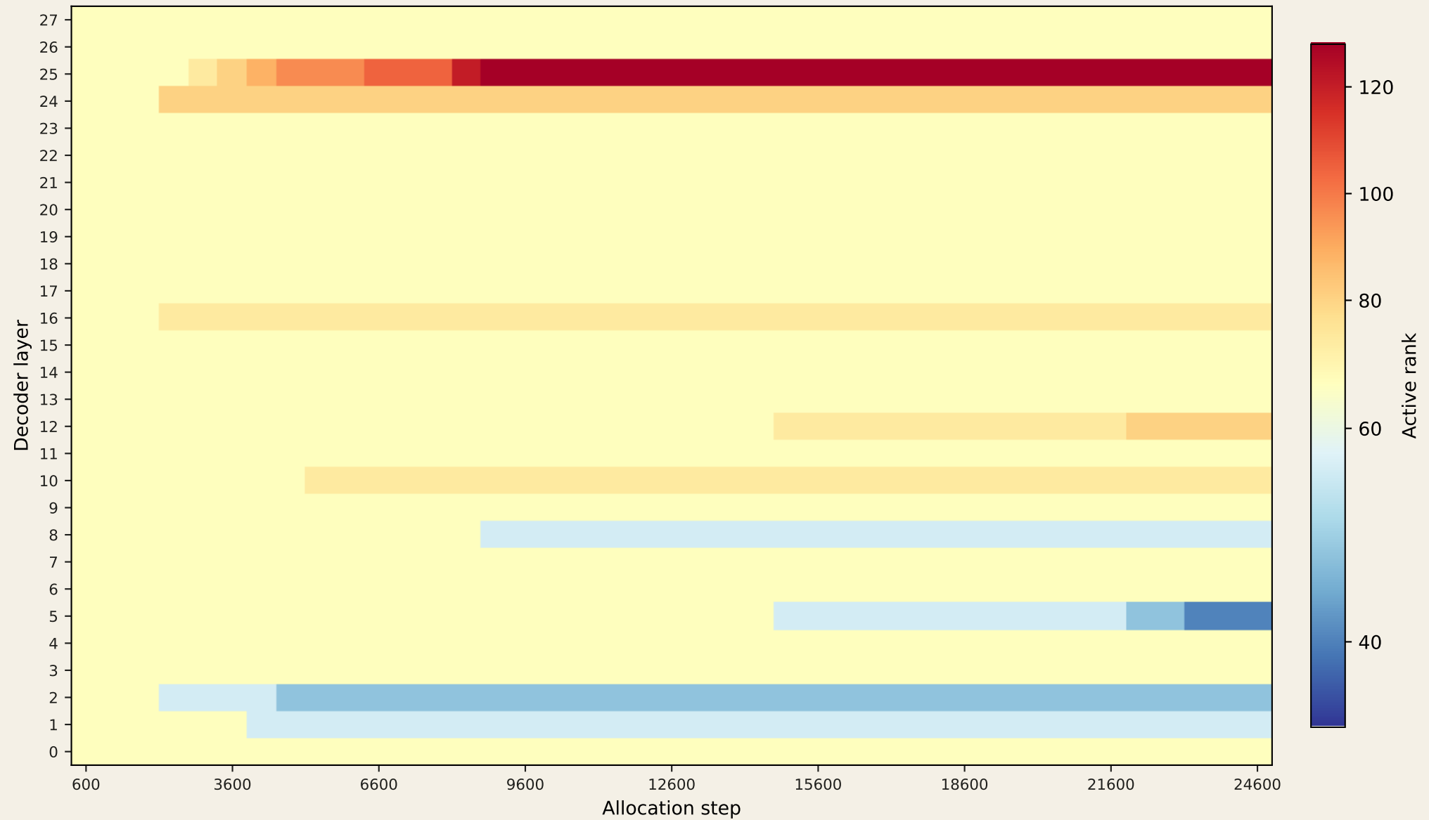
MLP Branch-Rank Trajectory
