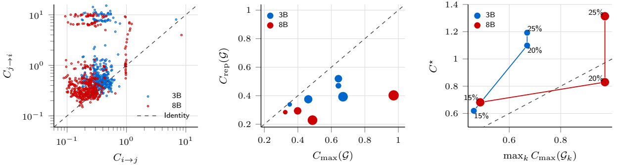
Fig. 2. Structural validation. (a) Directed replacement costs exhibit clear source–target asymmetry. (b) The best representation cost satisfies C_{rep}(G) \leq C_{max}(G) for every observed group. (c) C^* is compared directly with \max_k C_{max}(G_k) ; the dashed line marks equality.
