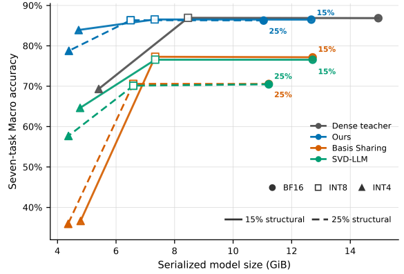
Fig. 3. Quantized Llama-3.1-8B storage–accuracy trade-off. BF16, INT8, and INT4 are shown at 15% and 25% structural compression; upper-left points are preferable.
