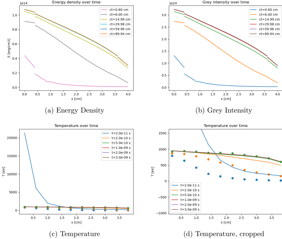
Figure 3: Modified FC Test results with T_b = 100 eV
