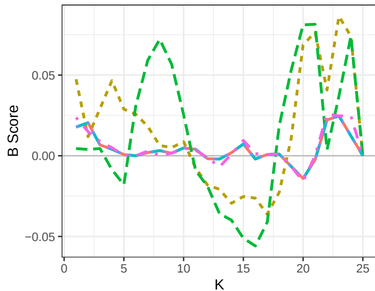
Behavior (T&C)
