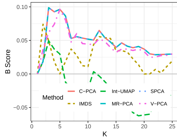
Behavior (LCMC)
