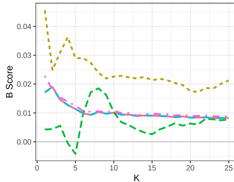
Behavior (MRRE)
