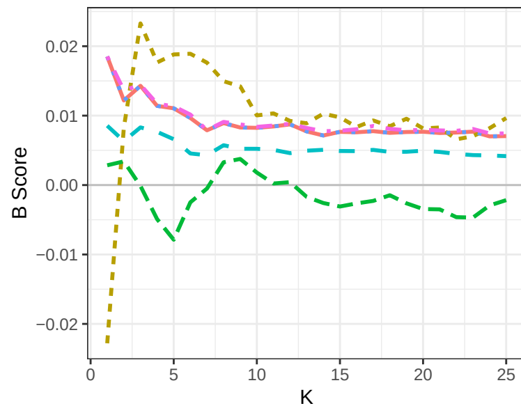
Behavior (MRRE)
