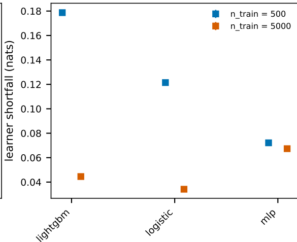
(b) learner shortfall
