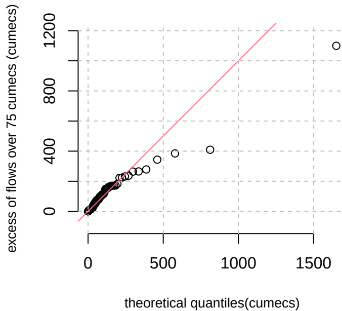
Figure 2: q-q plot for observed quantiles against the quantiles for the proposed distribution
