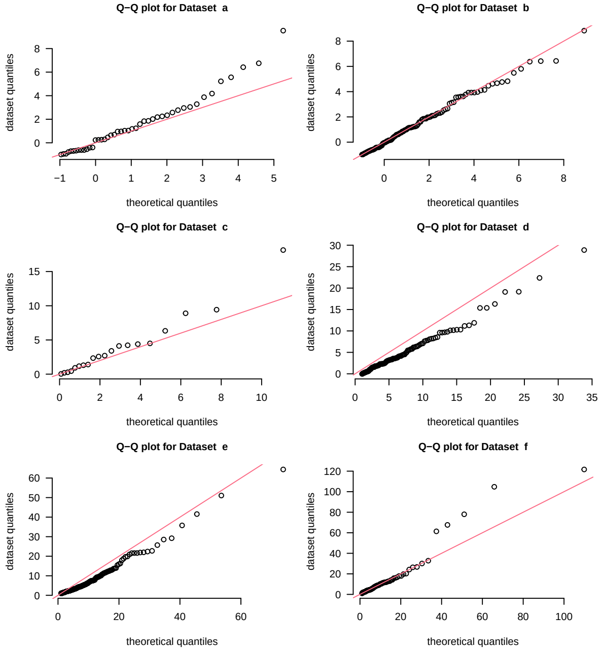
Figure 1: Quantile-quantile plots of each dataset against the quantiles of its stated generalised Pareto distribution.
