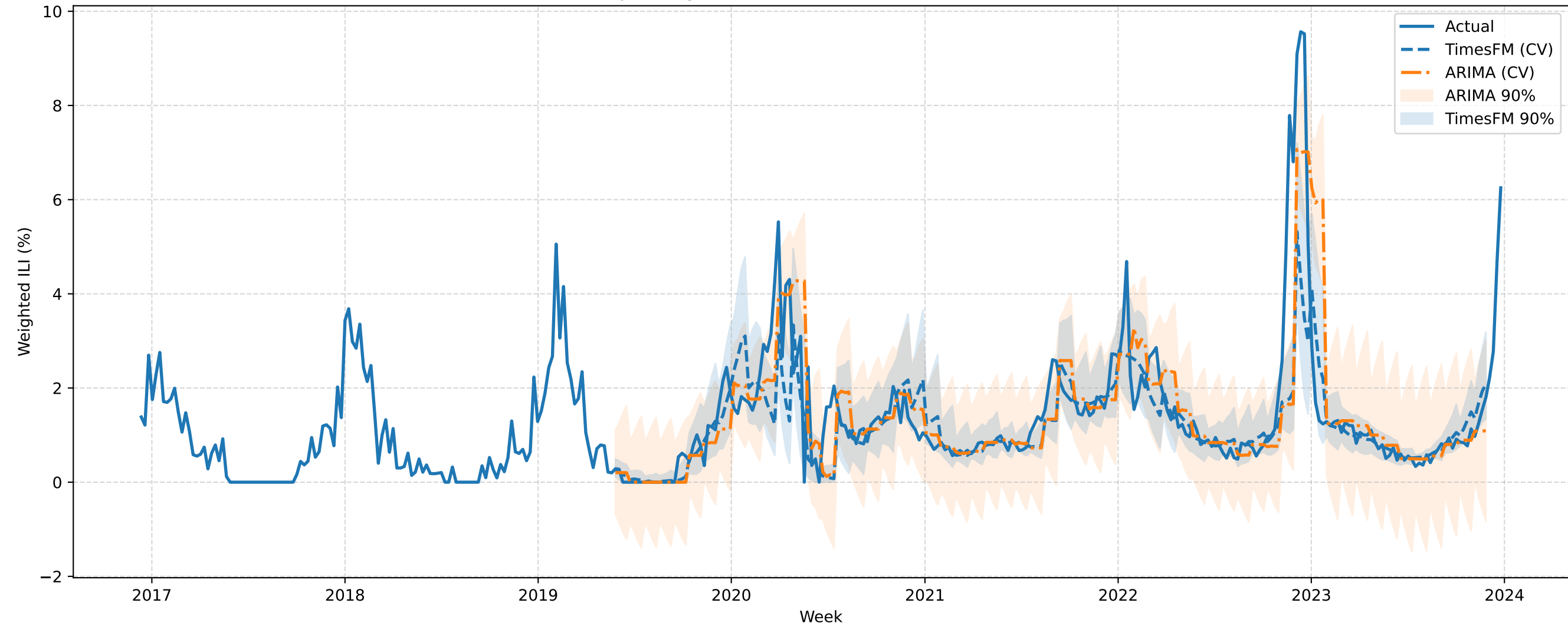
FINALIZED ID Expanding-Window CV (h=4): TimesFM vs ARIMA (best order)
