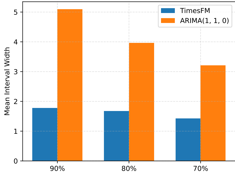
VERSIONED TX Width
