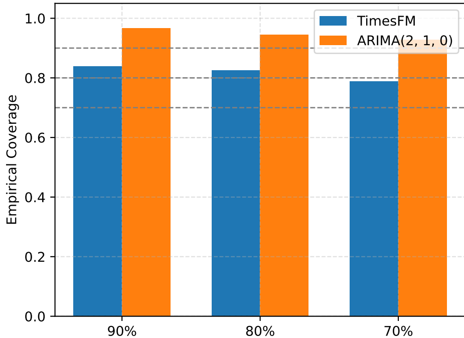
VERSIONED VA Coverage
