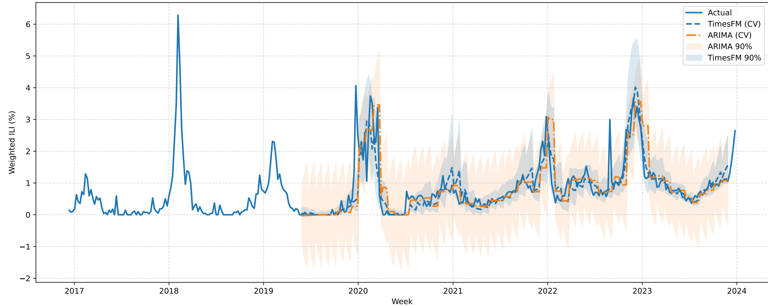
FINALIZED DE Expanding-Window CV (h=4): TimesFM vs ARIMA (best order)
