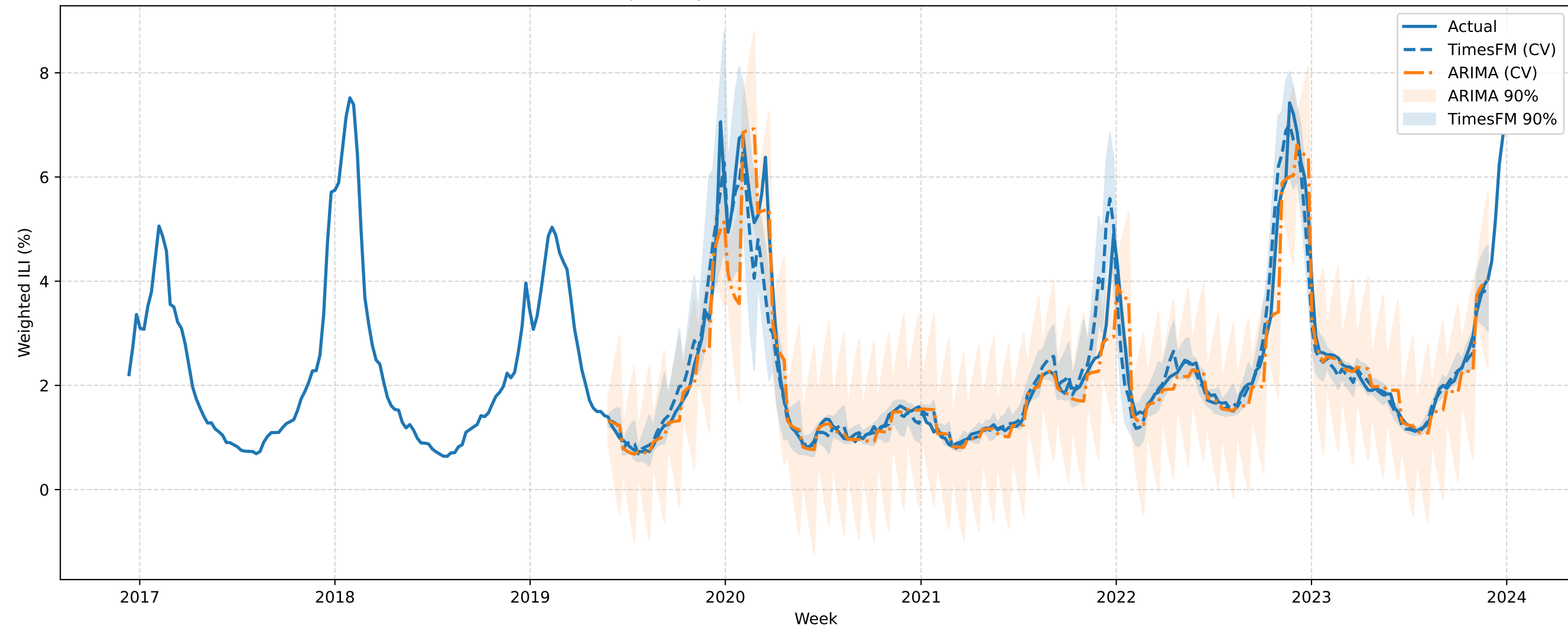
VERSIONED NAT Expanding-Window CV (h=4): TimesFM vs ARIMA (best order)
