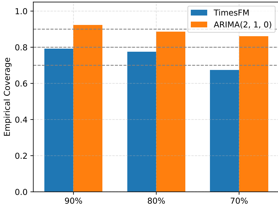
FINALIZED CA Coverage
