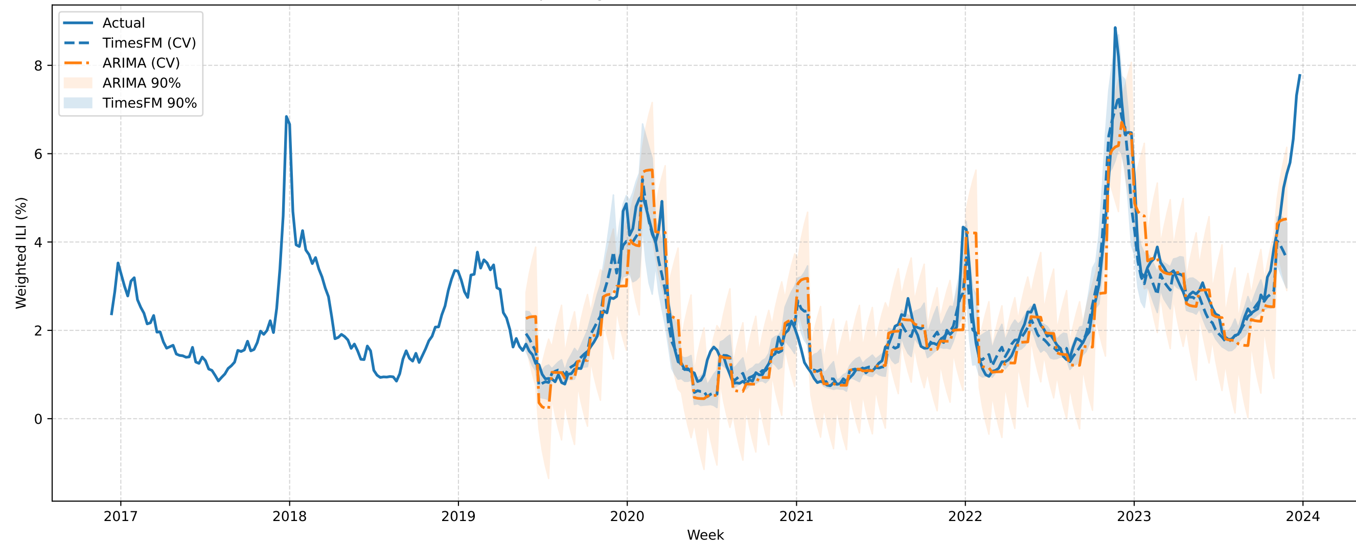
VERSIONED CA Expanding-Window CV (h=4): TimesFM vs ARIMA (best order)
