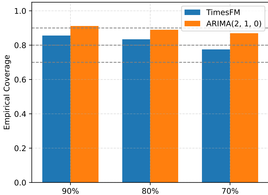
FINALIZED NAT Coverage
