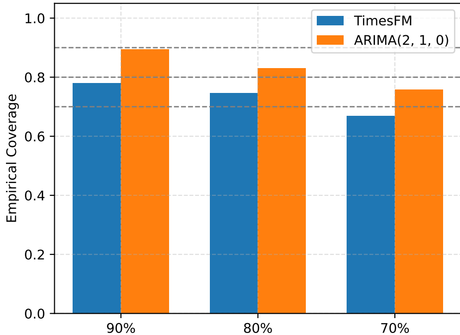
FINALIZED NV Coverage
