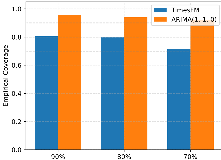
VERSIONED NJ Coverage
