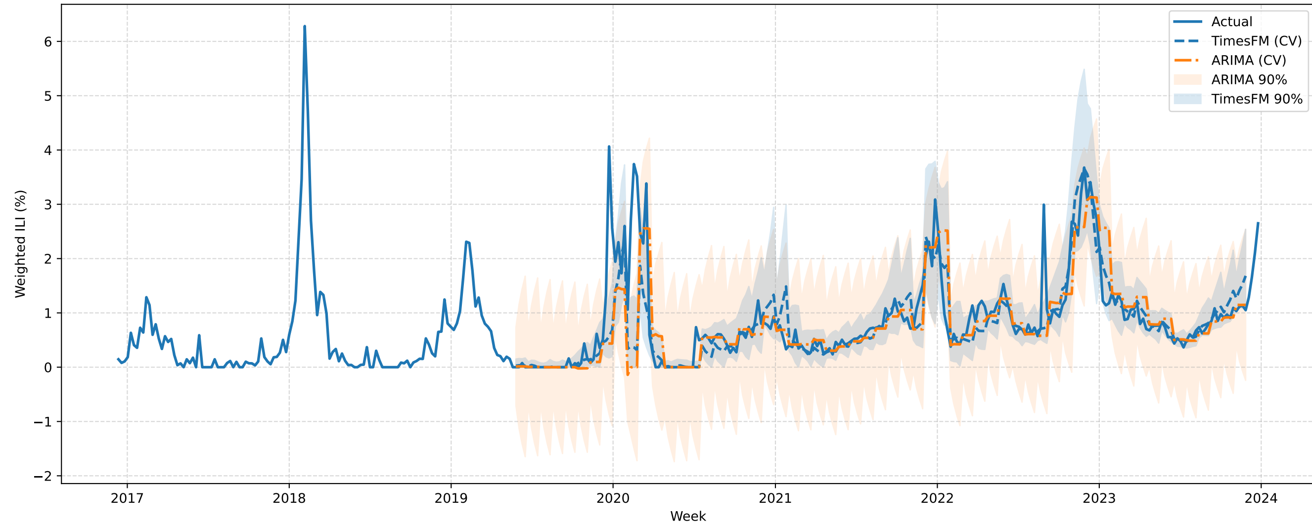
VERSIONED DE Expanding-Window CV (h=4): TimesFM vs ARIMA (best order)
