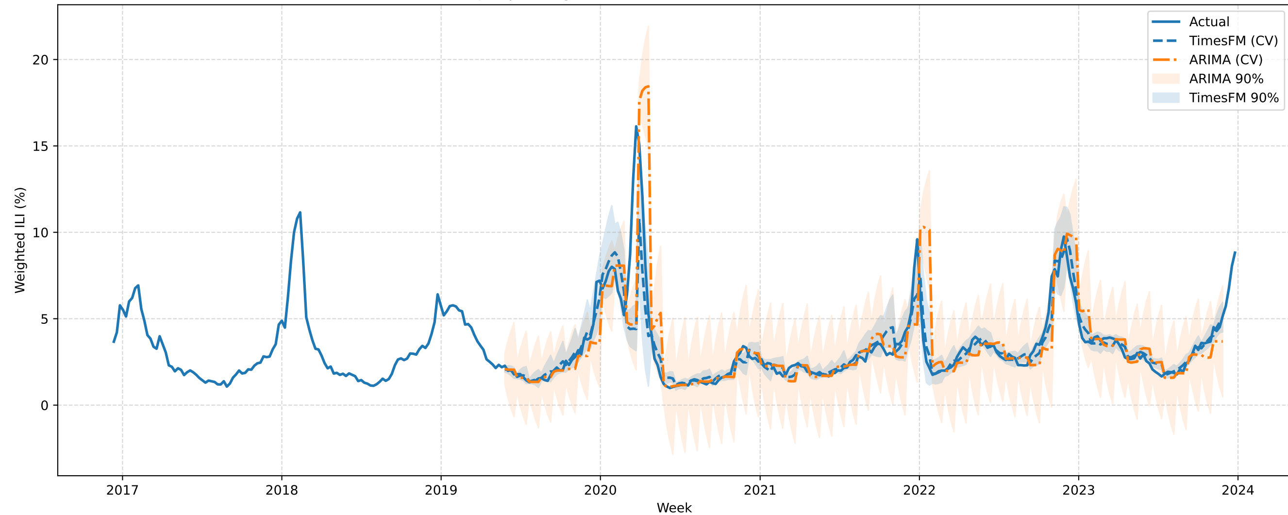
FINALIZED NJ Expanding-Window CV (h=4): TimesFM vs ARIMA (best order)
