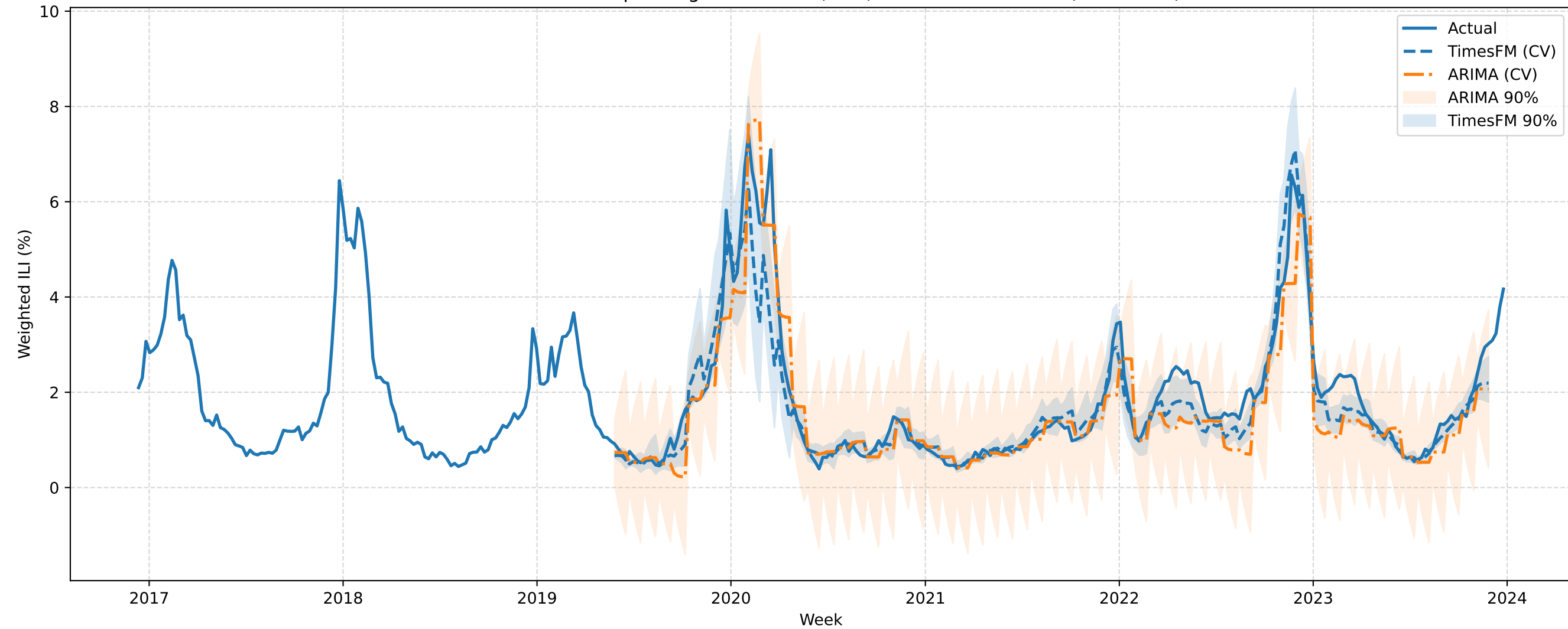
VERSIONED IL Expanding-Window CV (h=4): TimesFM vs ARIMA (best order)
