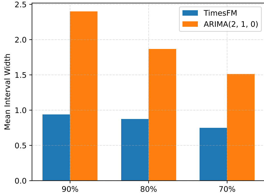
FINALIZED DE Width
