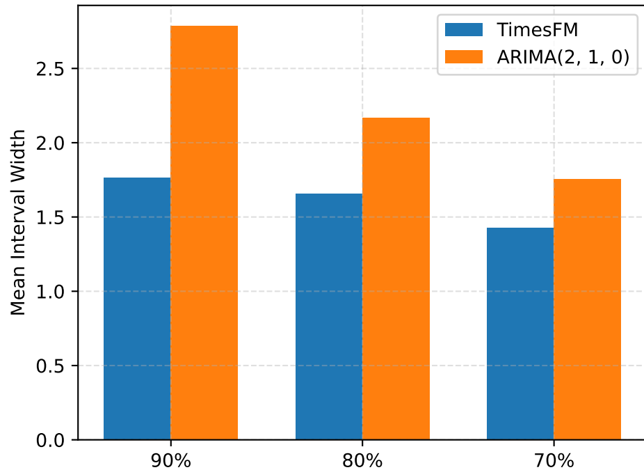
VERSIONED HI Width
