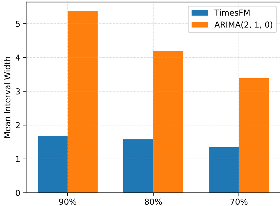
VERSIONED SC Width
