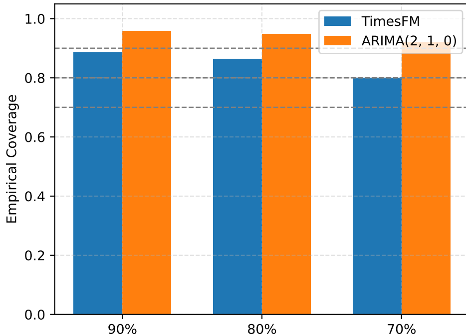
VERSIONED LA Coverage
