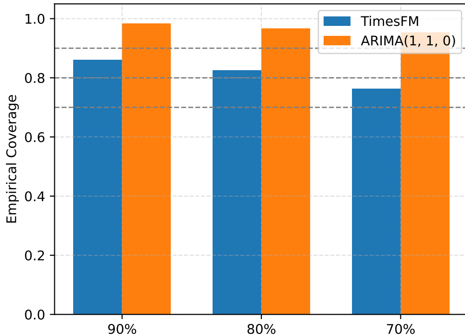
VERSIONED AL Coverage
