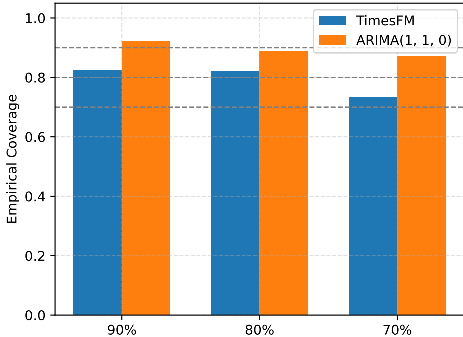
FINALIZED PA Coverage
