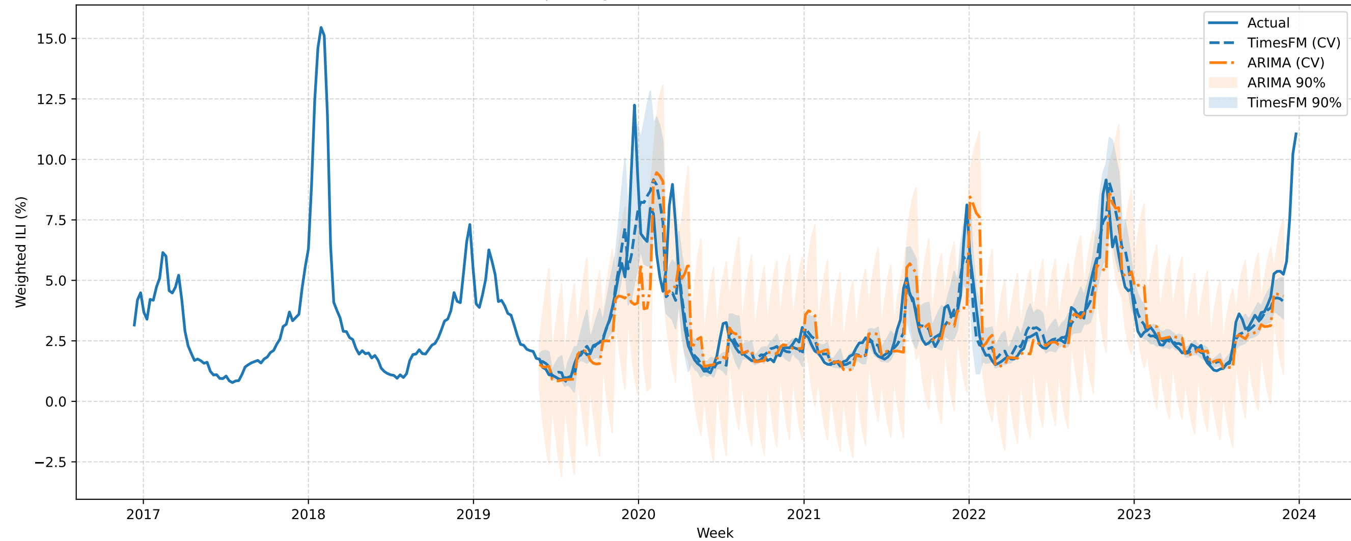
FINALIZED GA Expanding-Window CV (h=4): TimesFM vs ARIMA (best order)
