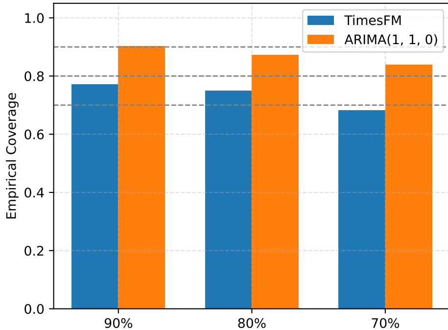
VERSIONED OH Coverage
