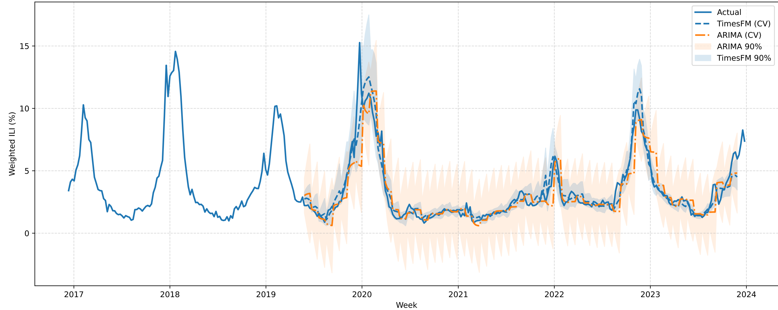
FINALIZED TX Expanding-Window CV (h=4): TimesFM vs ARIMA (best order)
