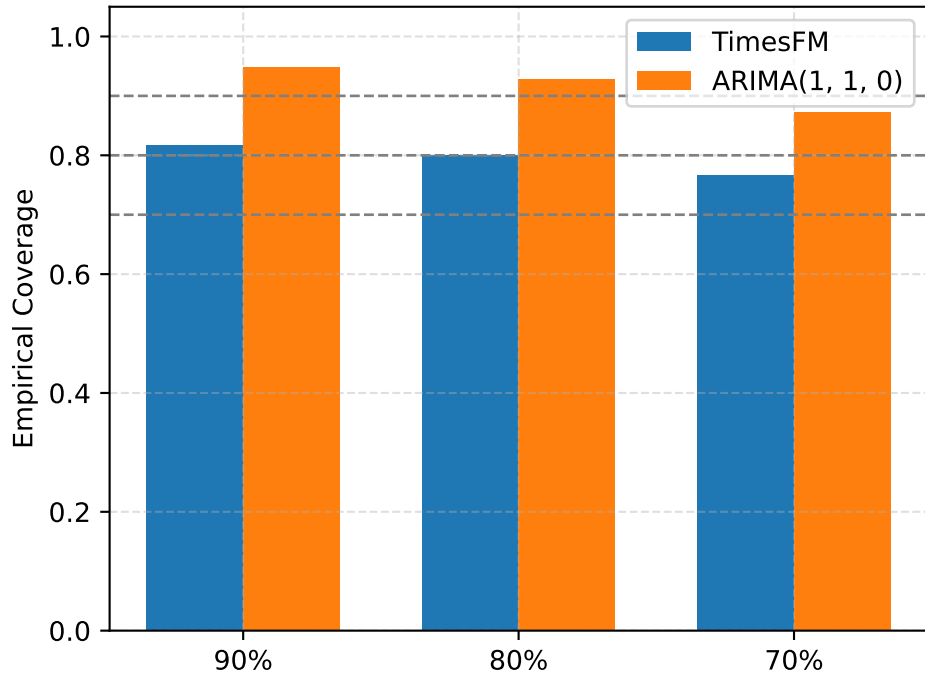
VERSIONED WV Coverage
