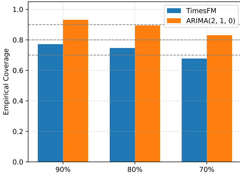
FINALIZED LA Coverage
