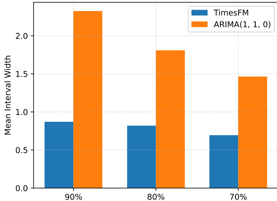
VERSIONED NAT Width
