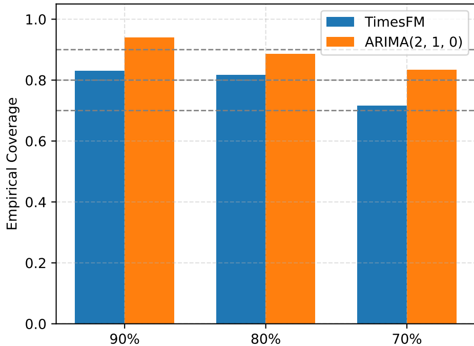
VERSIONED HI Coverage
