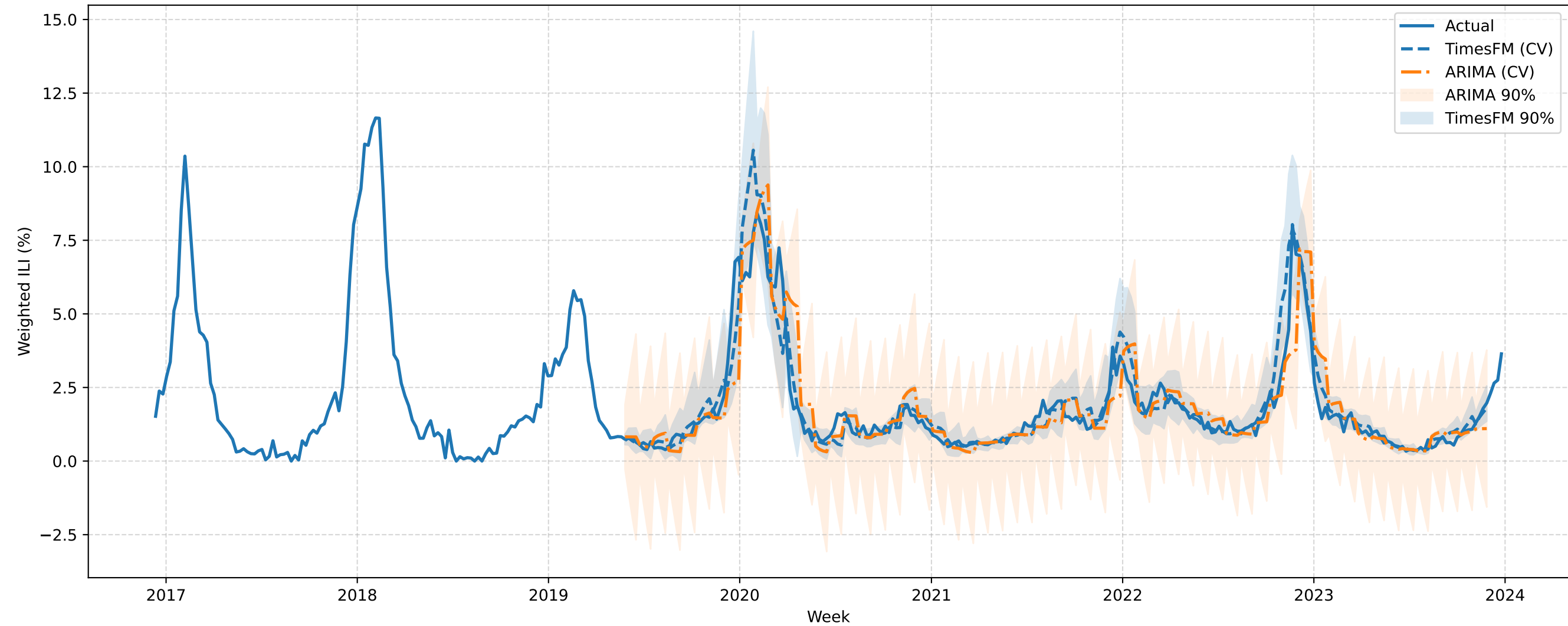
FINALIZED KS Expanding-Window CV (h=4): TimesFM vs ARIMA (best order)
