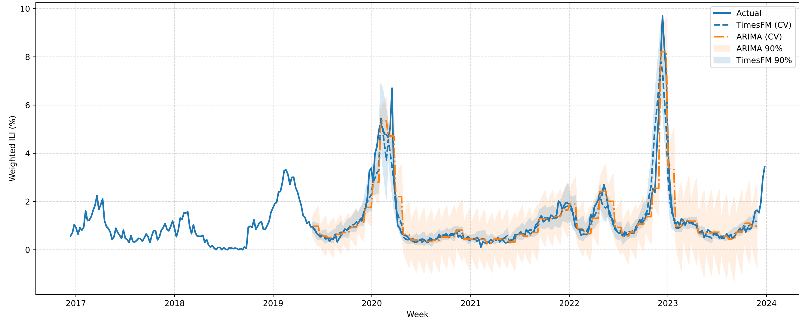
VERSIONED ME Expanding-Window CV (h=4): TimesFM vs ARIMA (best order)
