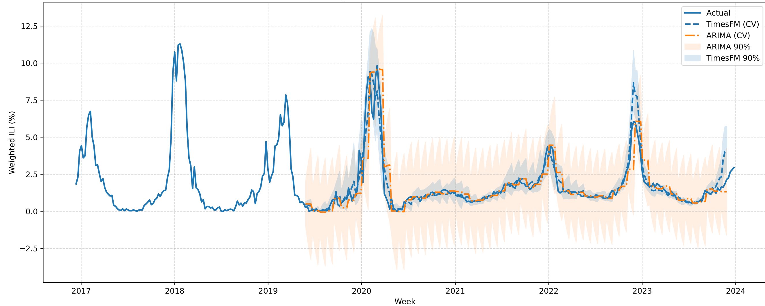
FINALIZED MO Expanding-Window CV (h=4): TimesFM vs ARIMA (best order)
