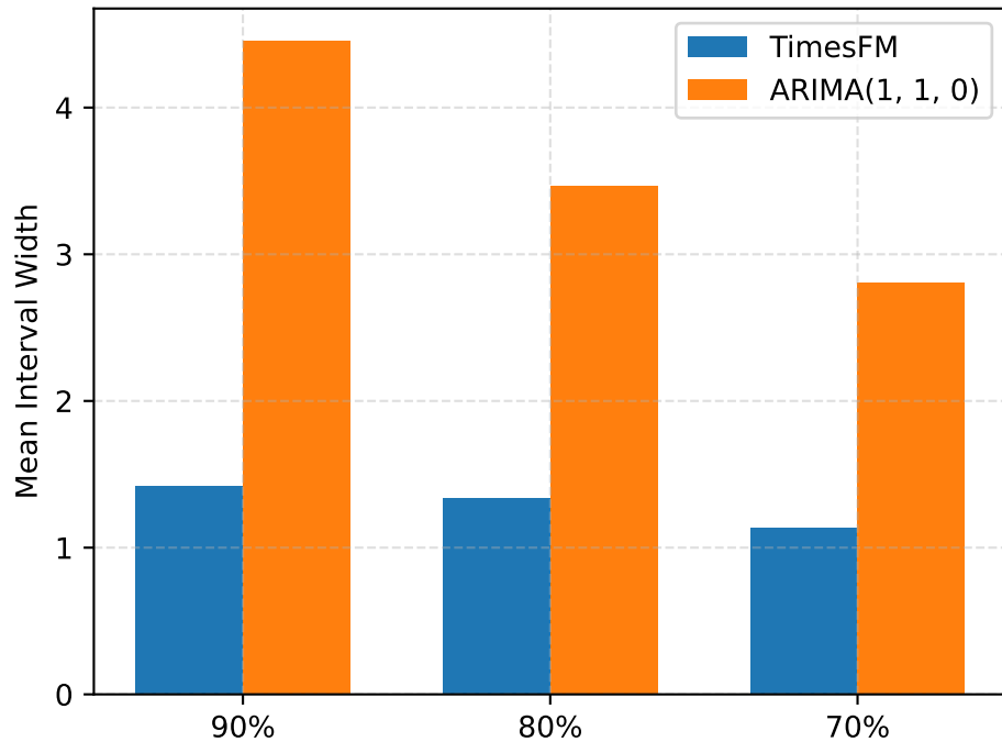
VERSIONED NJ Width
