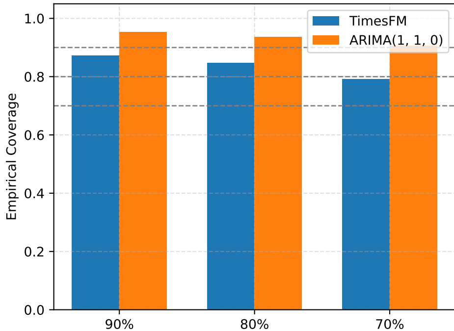
VERSIONED NAT Coverage
