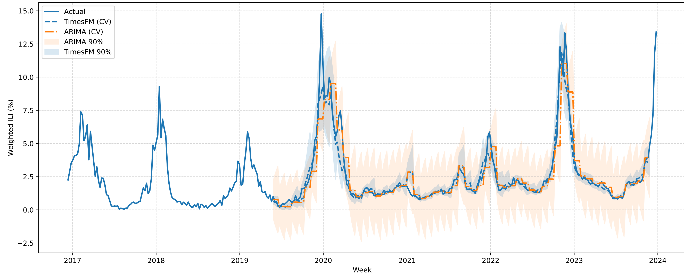
VERSIONED TN Expanding-Window CV (h=4): TimesFM vs ARIMA (best order)
