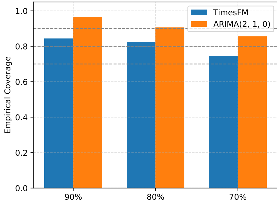
FINALIZED HI Coverage
