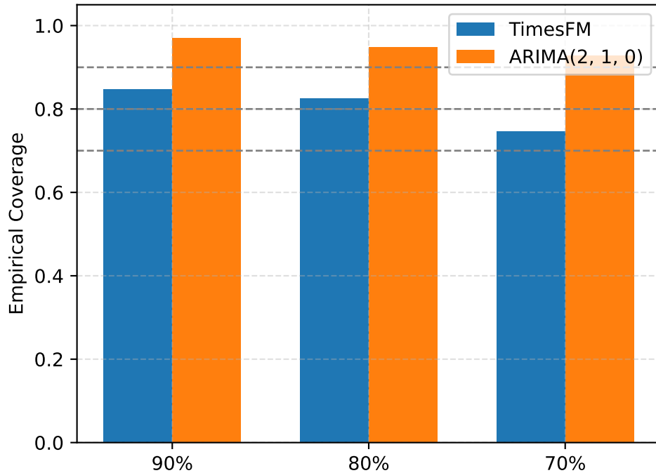
VERSIONED MO Coverage
