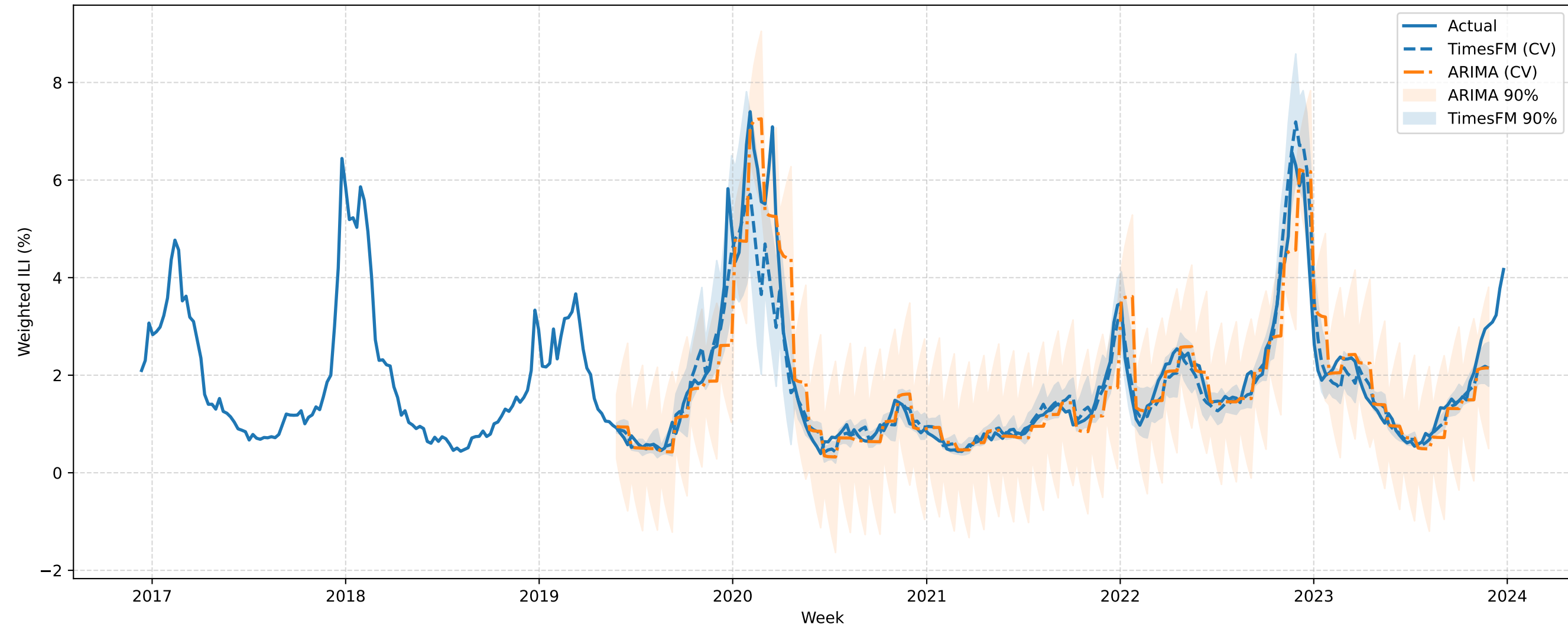
FINALIZED IL Expanding-Window CV (h=4): TimesFM vs ARIMA (best order)
