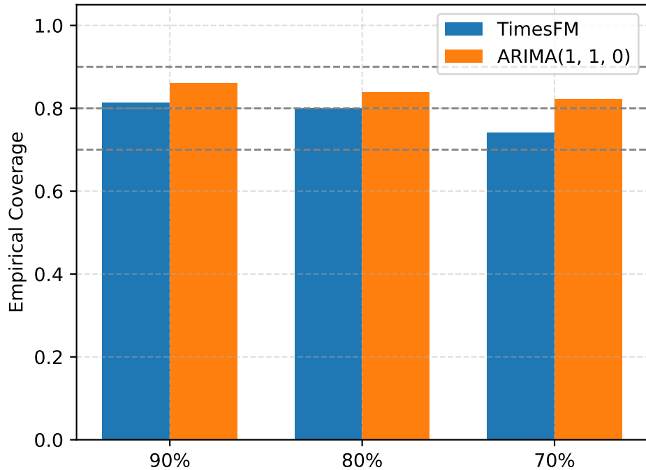
VERSIONED MN Coverage
