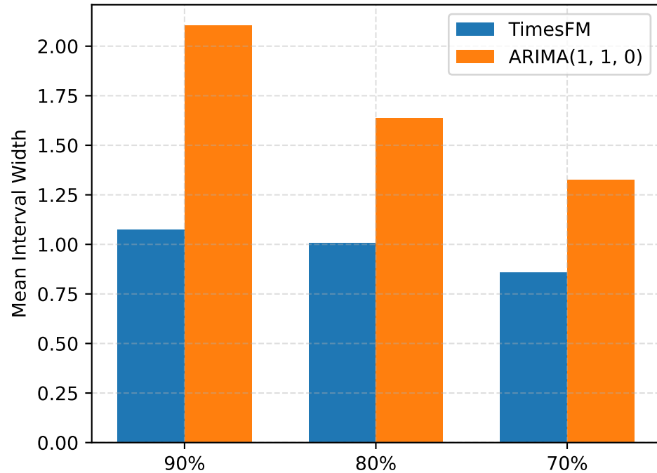
VERSIONED OH Width
