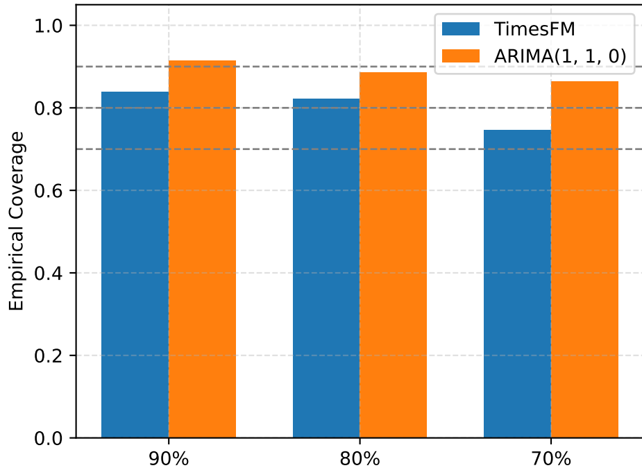
FINALIZED VA Coverage
