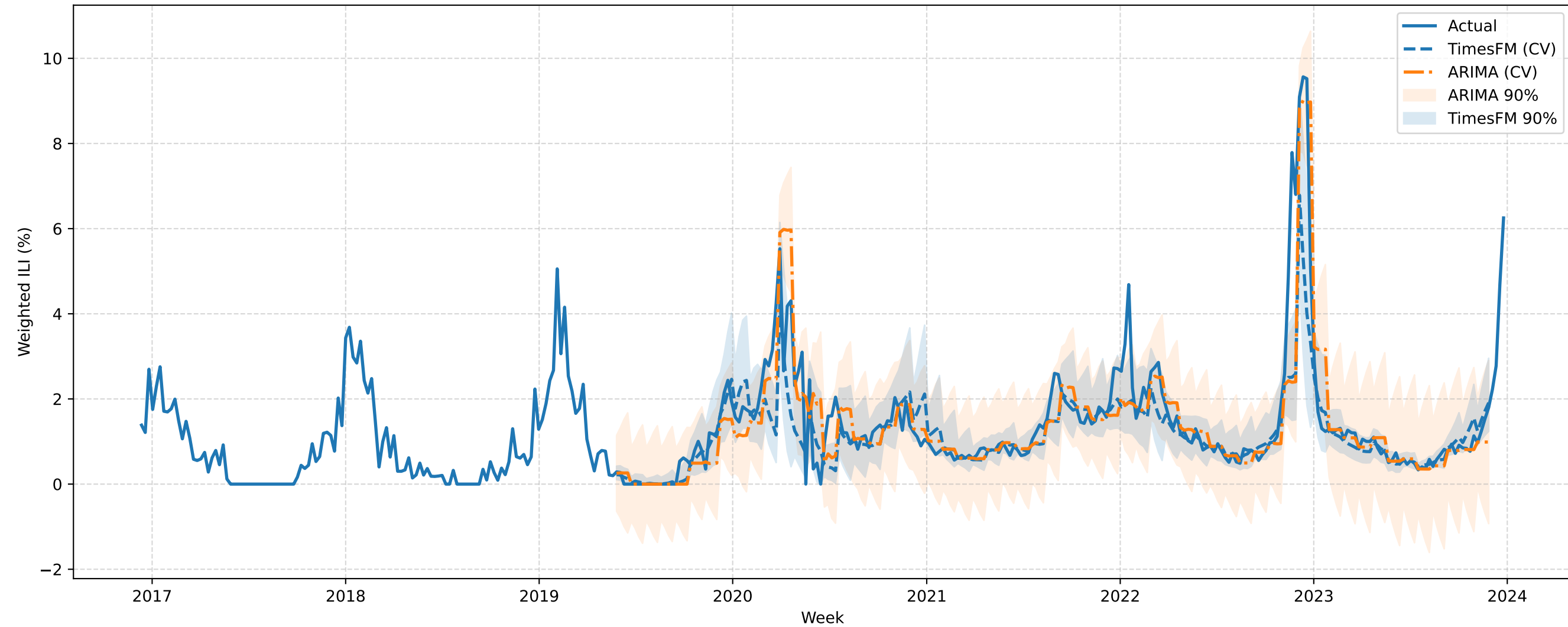
VERSIONED ID Expanding-Window CV (h=4): TimesFM vs ARIMA (best order)
