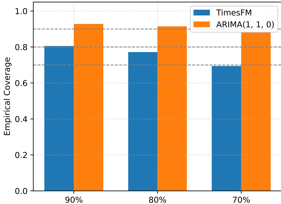
FINALIZED WV Coverage
