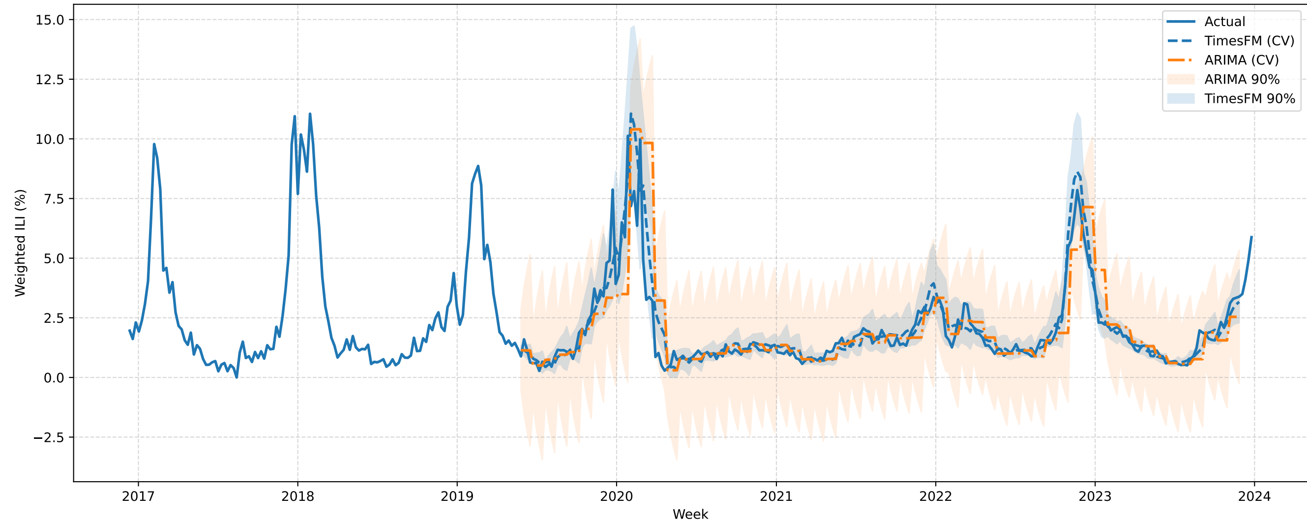
FINALIZED AR Expanding-Window CV (h=4): TimesFM vs ARIMA (best order)
