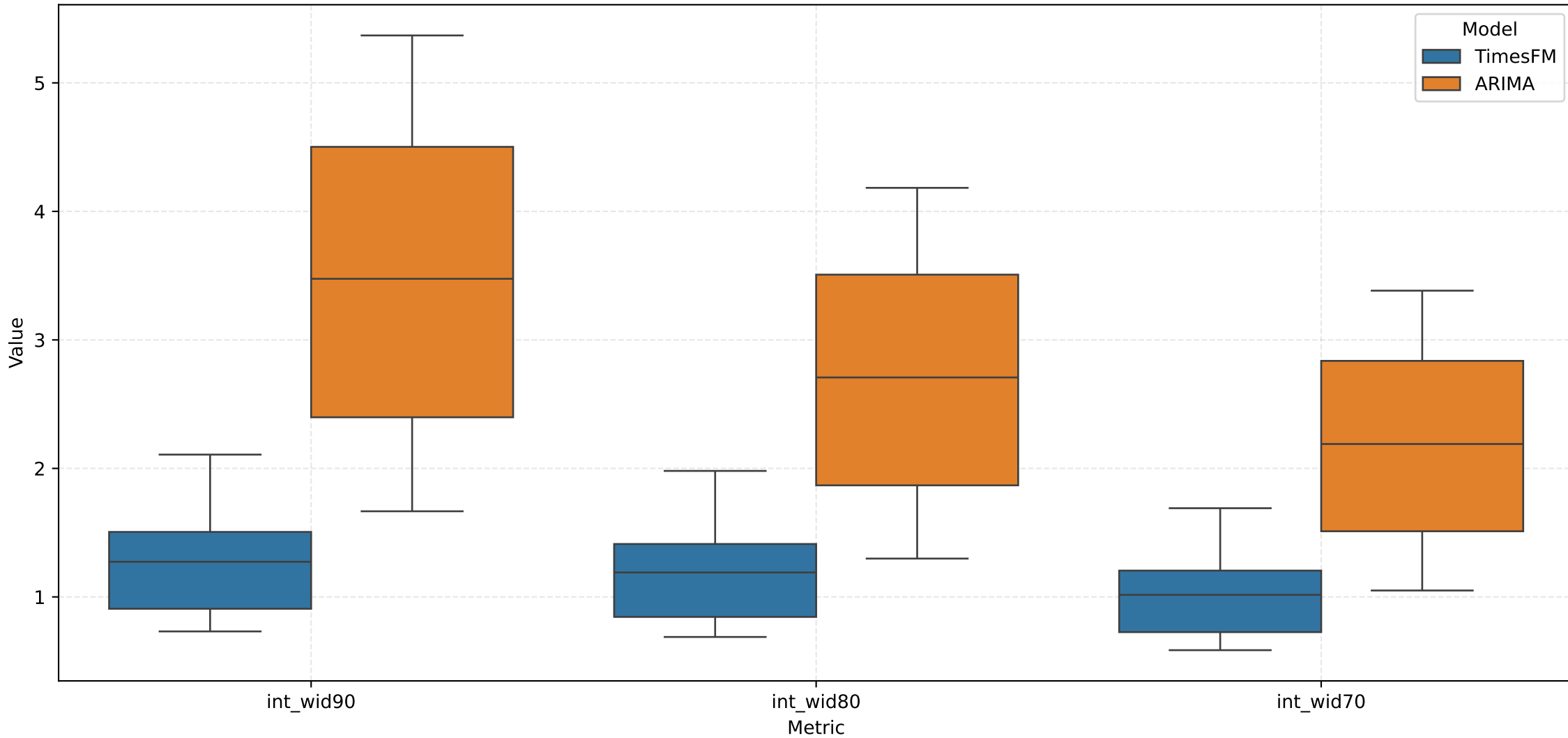
Prediction Interval Widths Across Regions - VERSIONED
