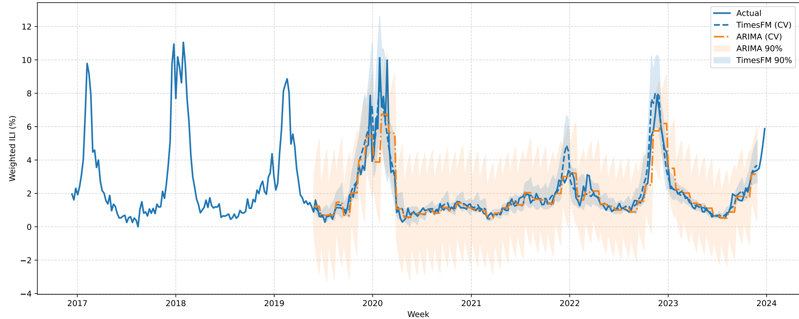
VERSIONED AR Expanding-Window CV (h=4): TimesFM vs ARIMA (best order)
