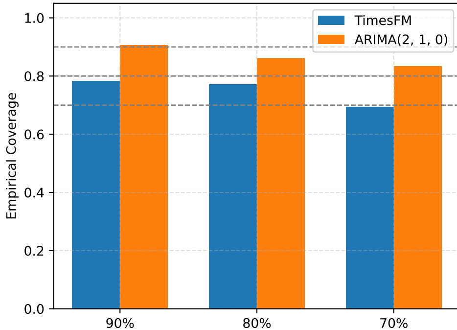
FINALIZED NJ Coverage
