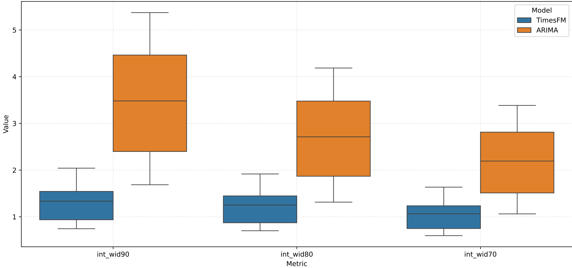
Prediction Interval Widths Across Regions - FINALIZED
