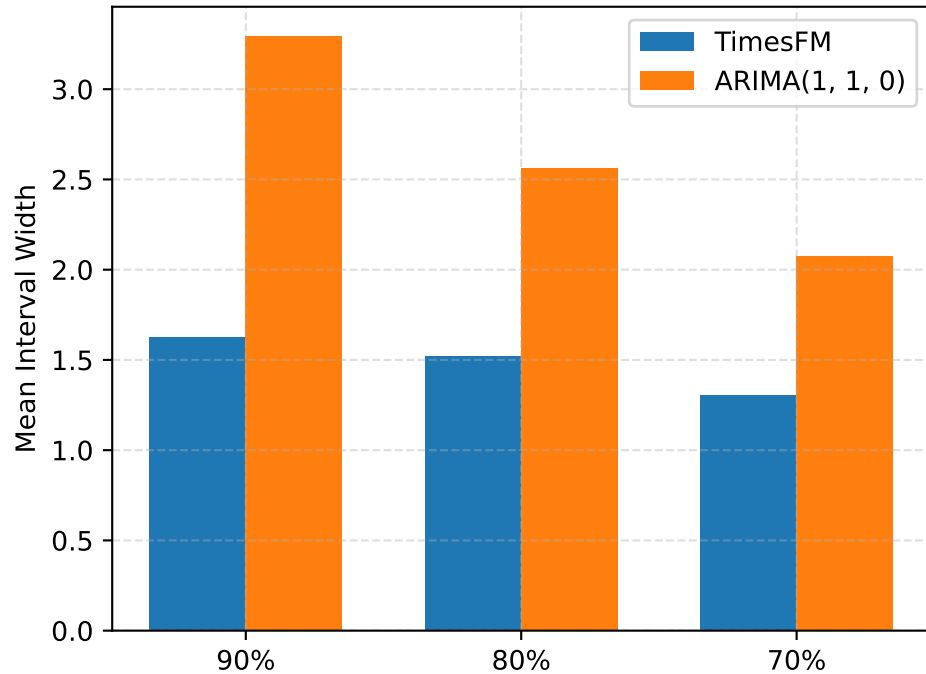
FINALIZED WY Width
