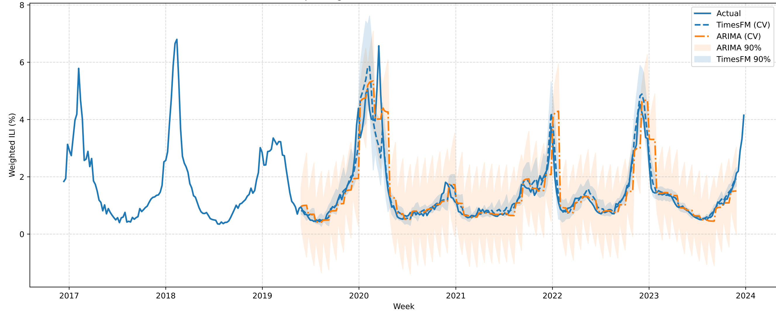
FINALIZED PA Expanding-Window CV (h=4): TimesFM vs ARIMA (best order)
