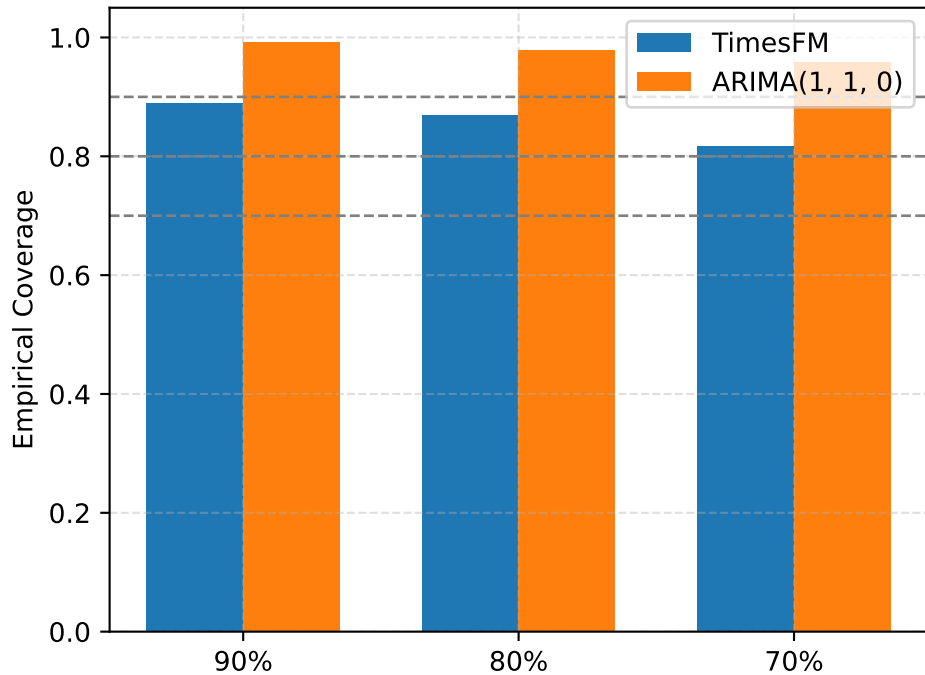
VERSIONED NC Coverage
