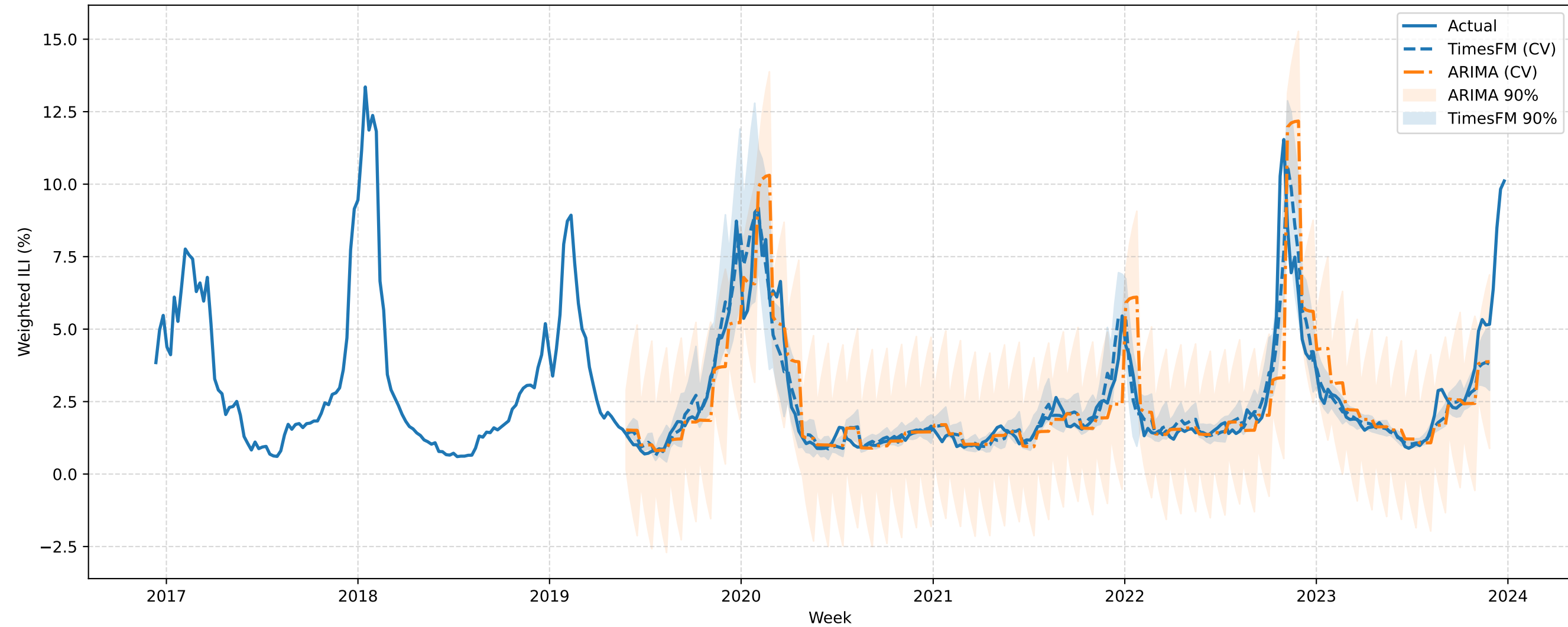
FINALIZED AL Expanding-Window CV (h=4): TimesFM vs ARIMA (best order)
