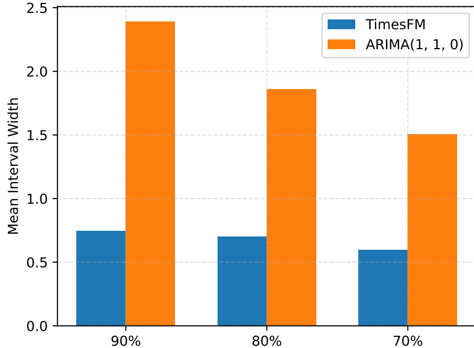
FINALIZED PA Width
