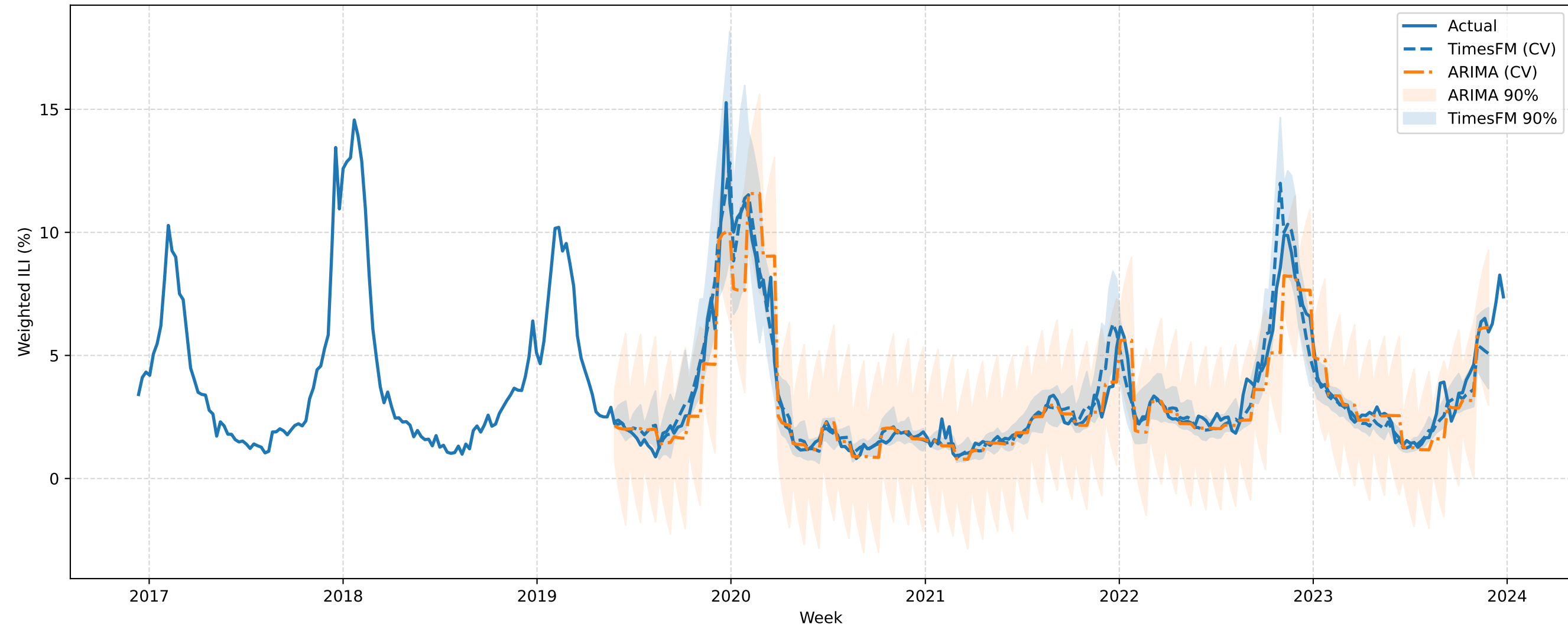
VERSIONED TX Expanding-Window CV (h=4): TimesFM vs ARIMA (best order)
