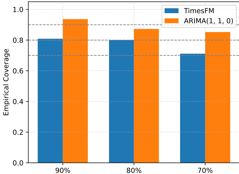
FINALIZED AZ Coverage
