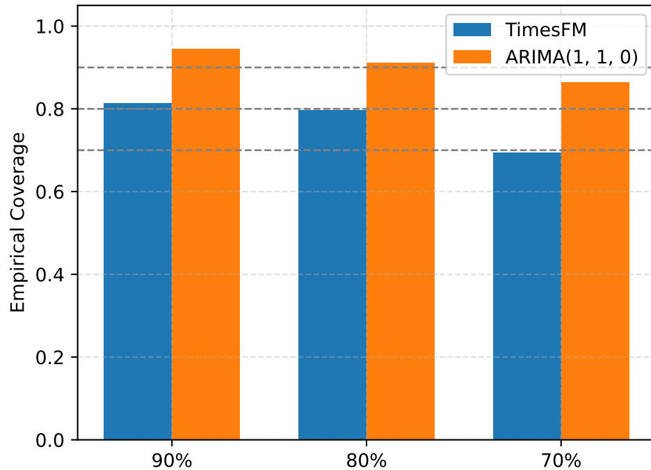
FINALIZED OK Coverage
