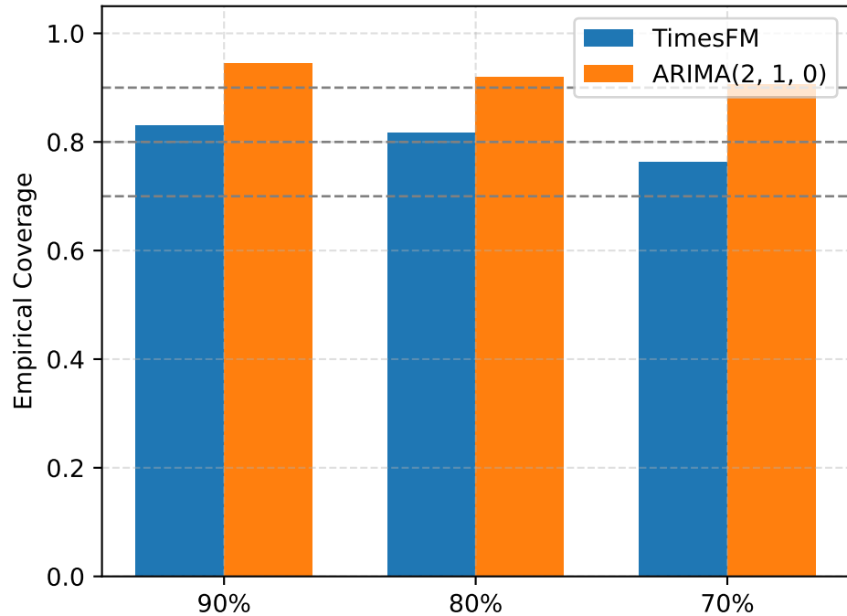
FINALIZED KS Coverage
