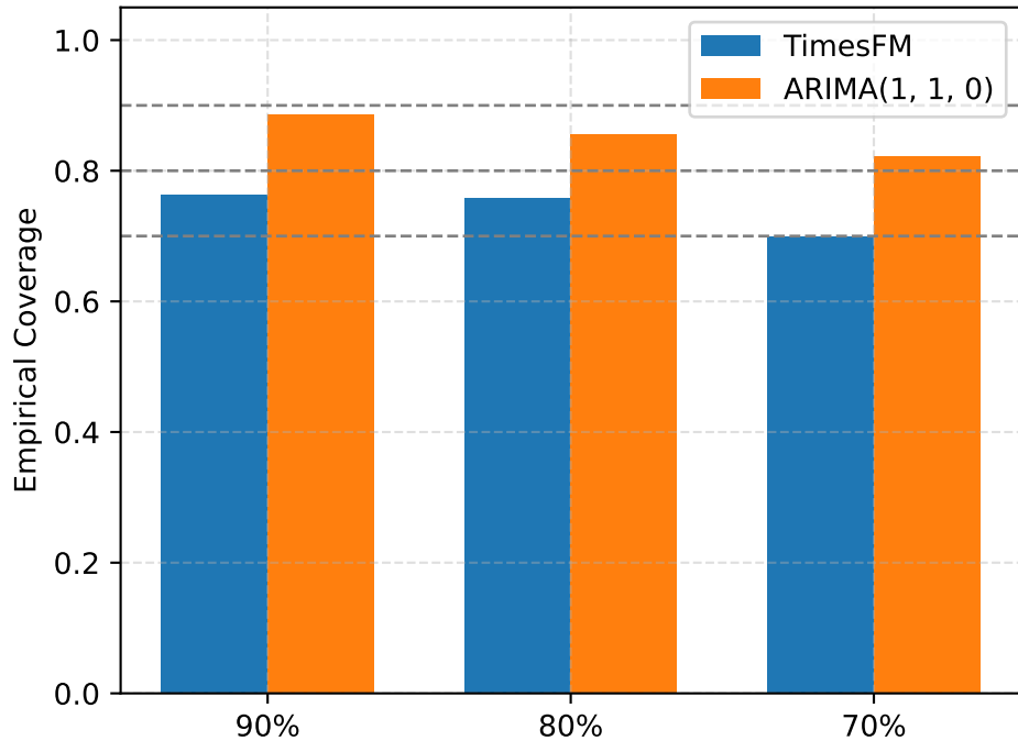
FINALIZED ID Coverage
