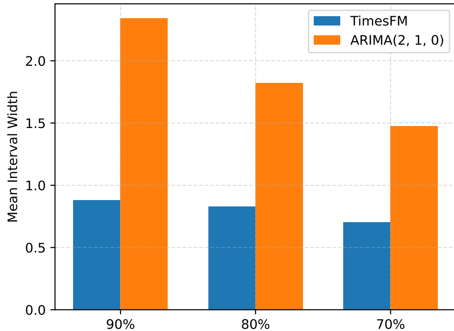
FINALIZED NAT Width
