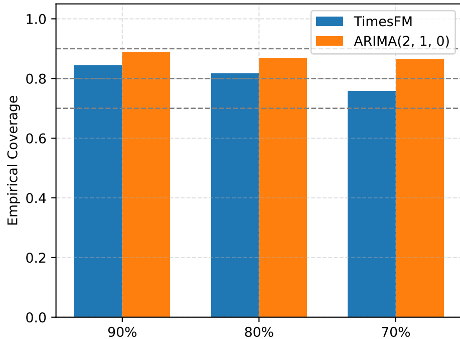
FINALIZED ME Coverage
