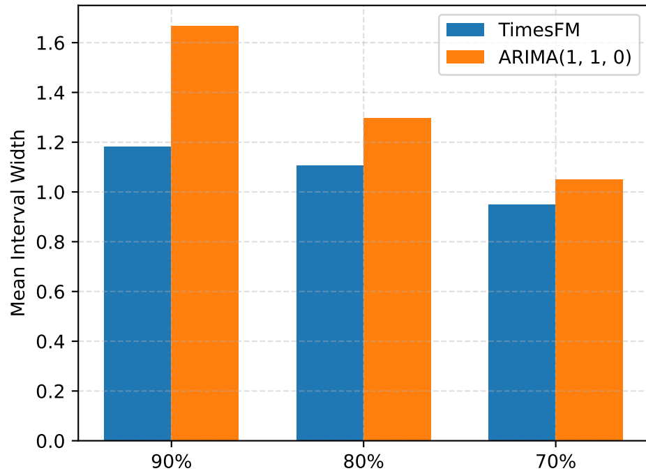
VERSIONED NV Width
