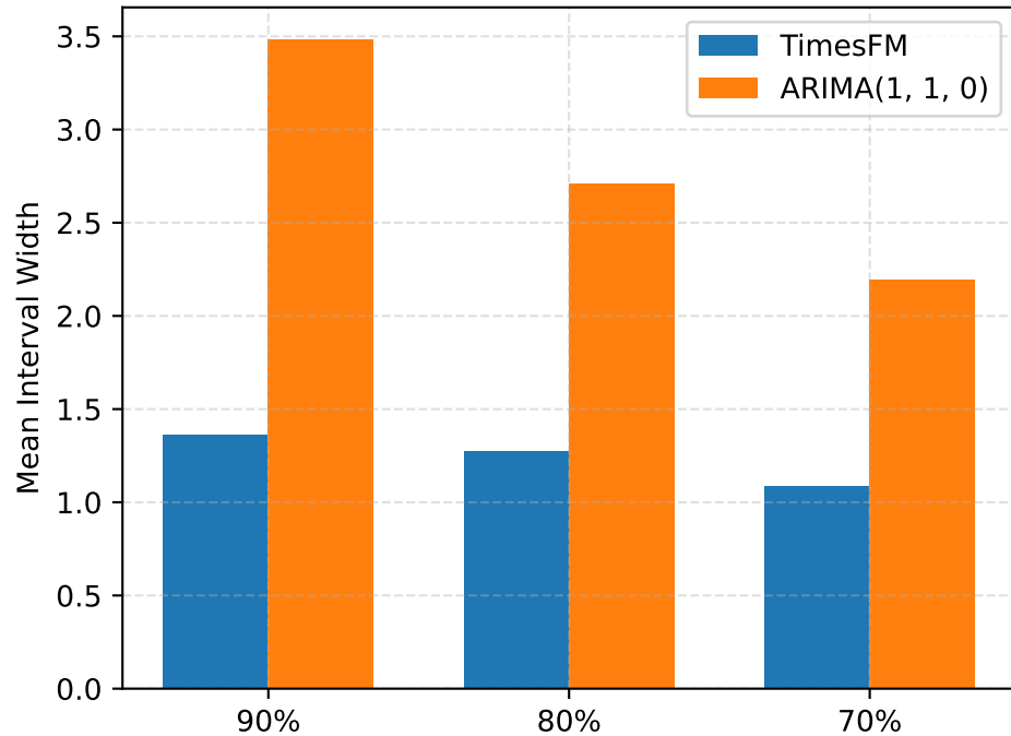
FINALIZED WV Width
