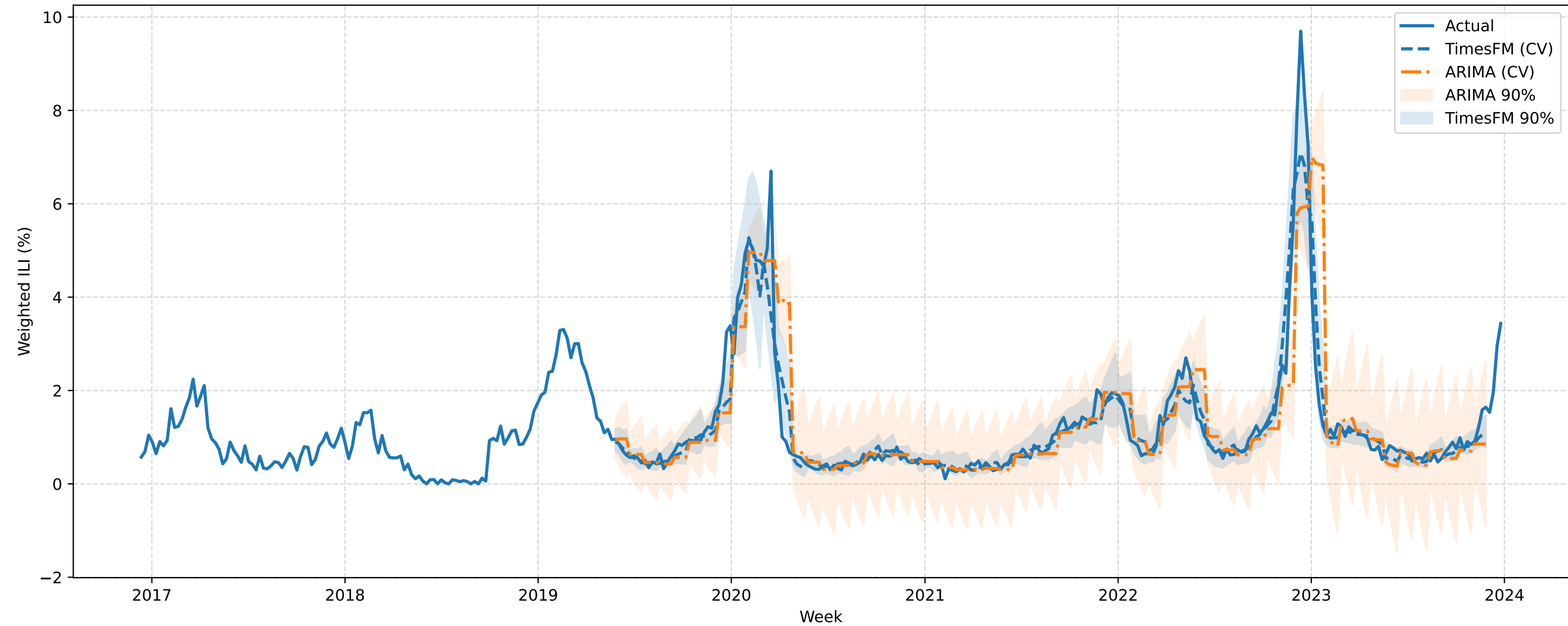
FINALIZED ME Expanding-Window CV (h=4): TimesFM vs ARIMA (best order)
