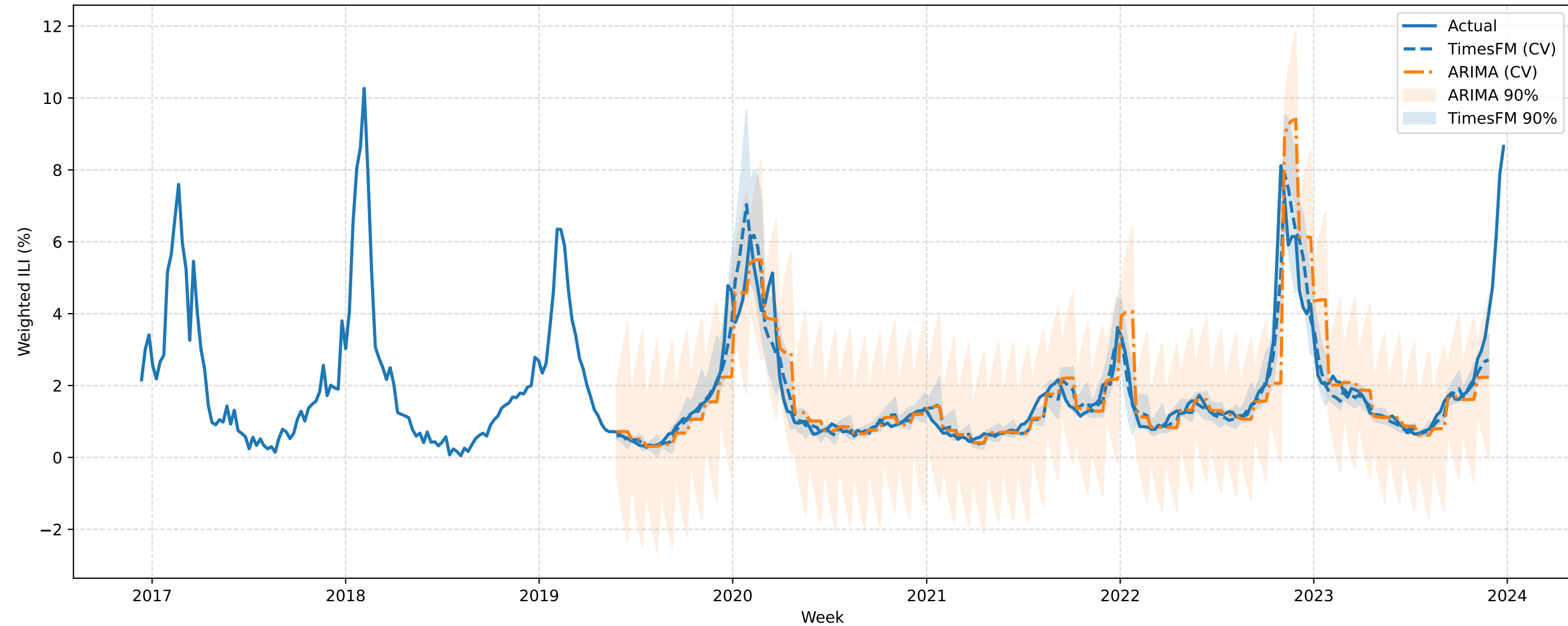
FINALIZED NC Expanding-Window CV (h=4): TimesFM vs ARIMA (best order)
