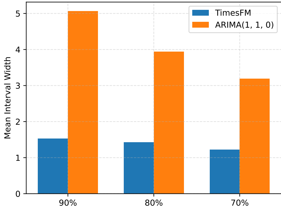
FINALIZED AR Width
