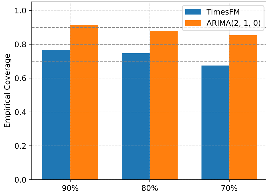
FINALIZED GA Coverage
