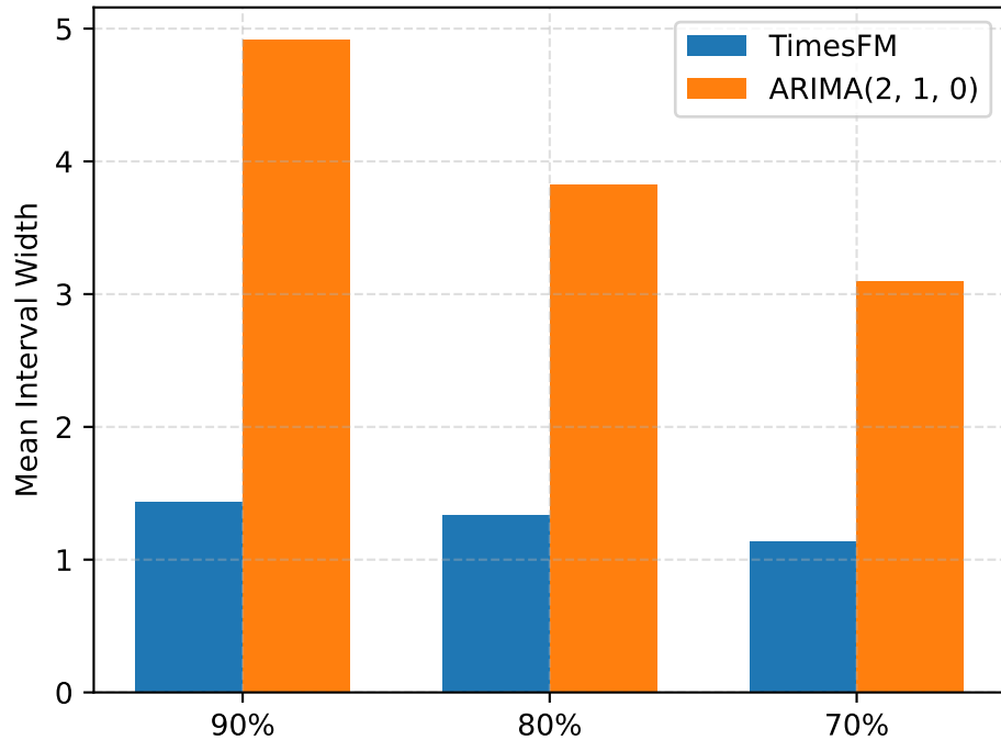
VERSIONED MO Width
