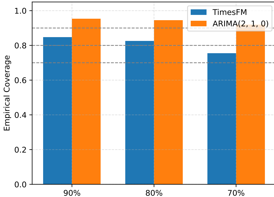
FINALIZED MO Coverage
