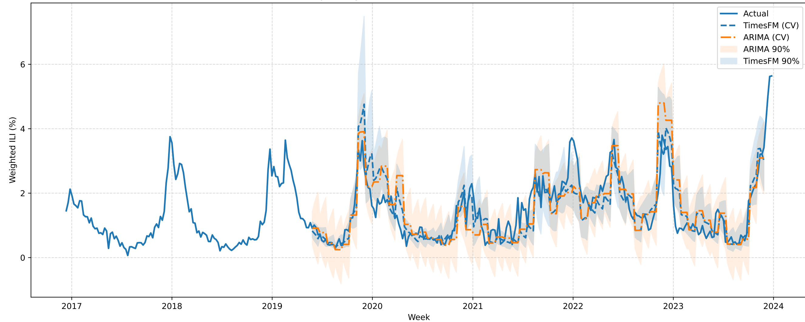
VERSIONED NV Expanding-Window CV (h=4): TimesFM vs ARIMA (best order)
