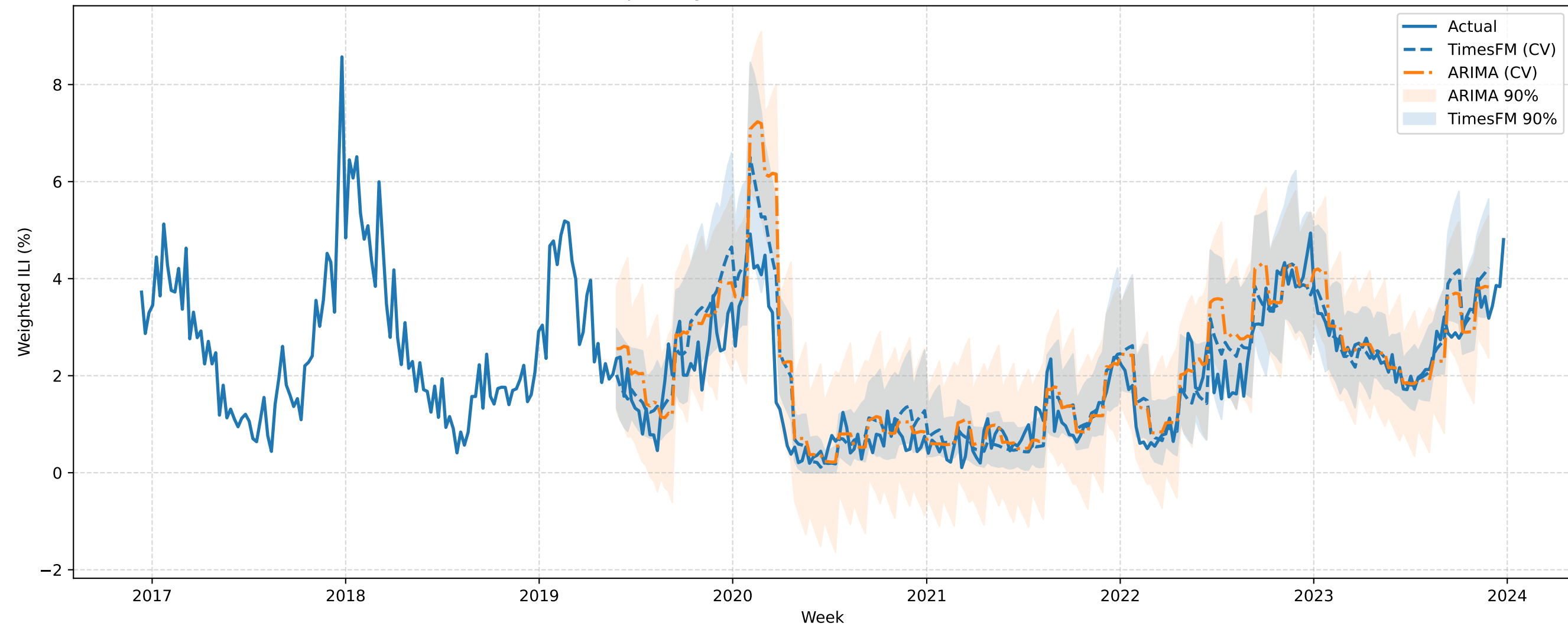
VERSIONED HI Expanding-Window CV (h=4): TimesFM vs ARIMA (best order)
