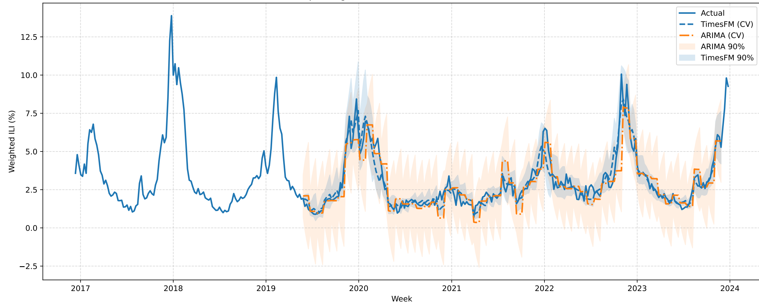
VERSIONED MS Expanding-Window CV (h=4): TimesFM vs ARIMA (best order)
