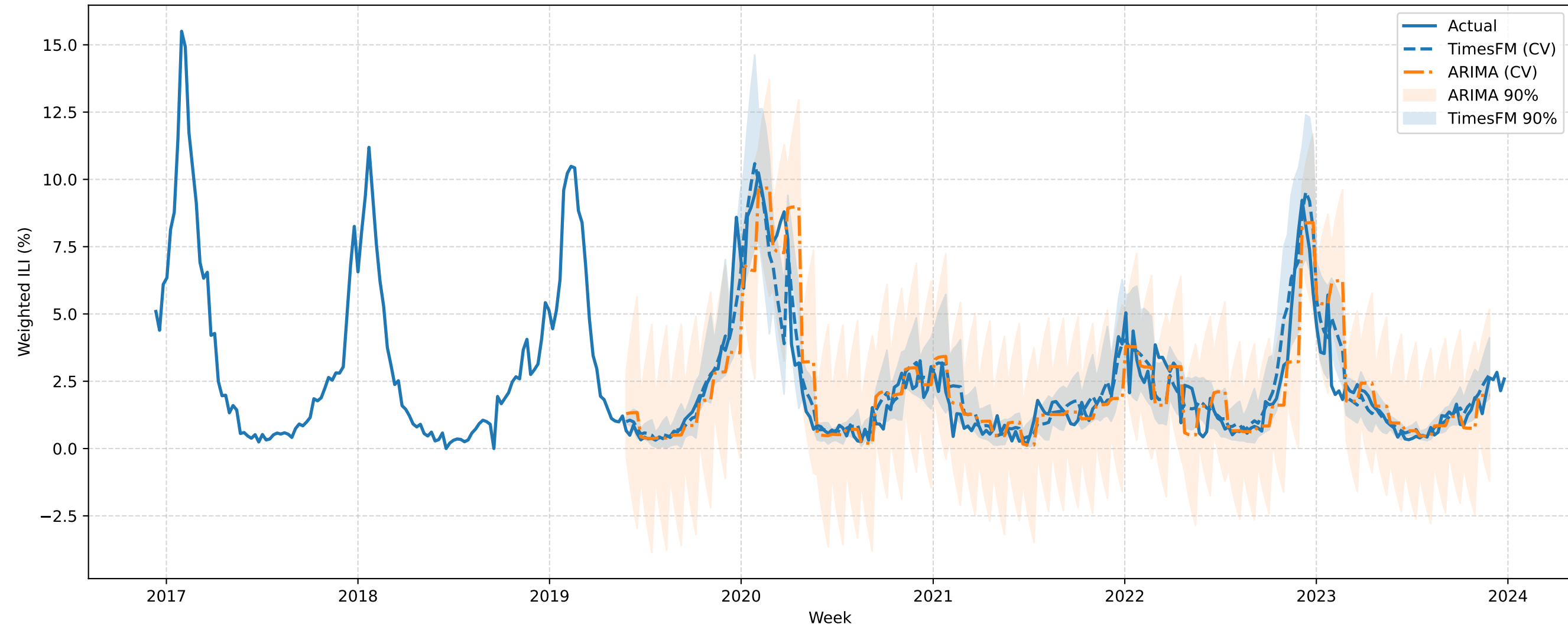
FINALIZED OK Expanding-Window CV (h=4): TimesFM vs ARIMA (best order)
