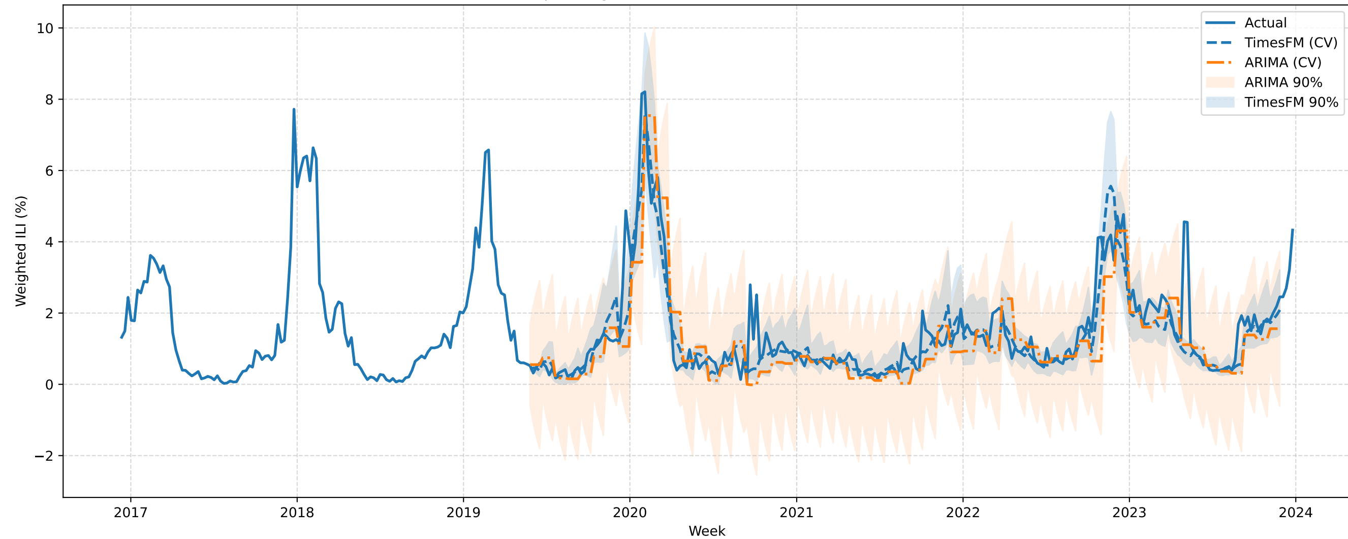
VERSIONED WV Expanding-Window CV (h=4): TimesFM vs ARIMA (best order)
