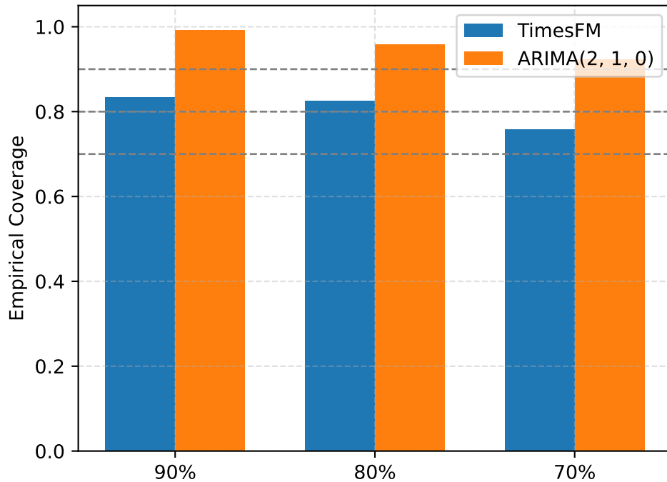
VERSIONED MS Coverage
