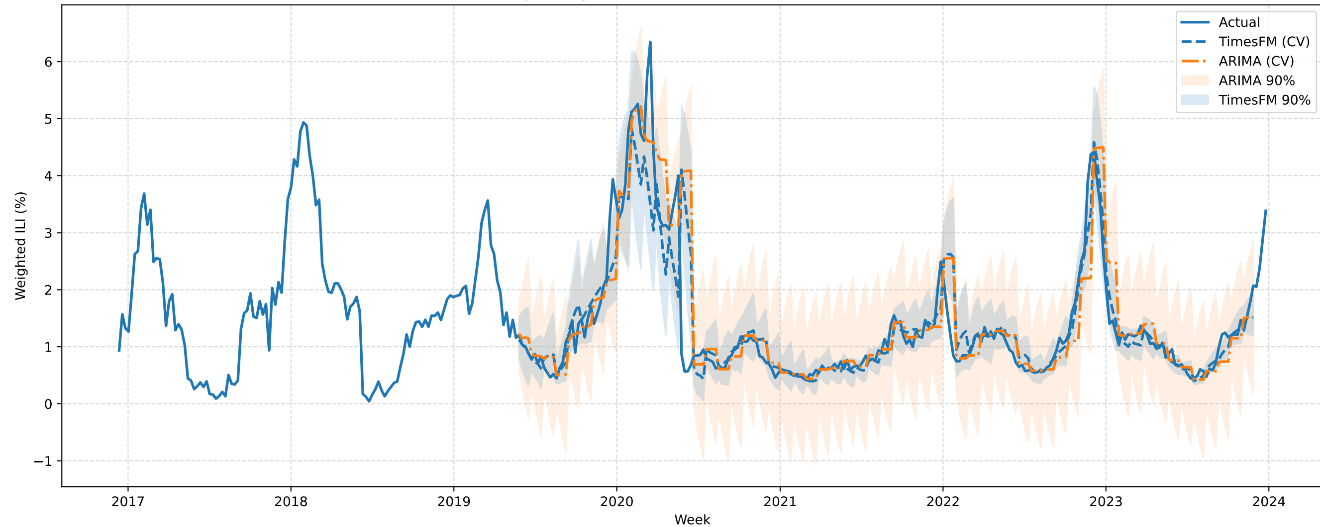
FINALIZED WI Expanding-Window CV (h=4): TimesFM vs ARIMA (best order)
