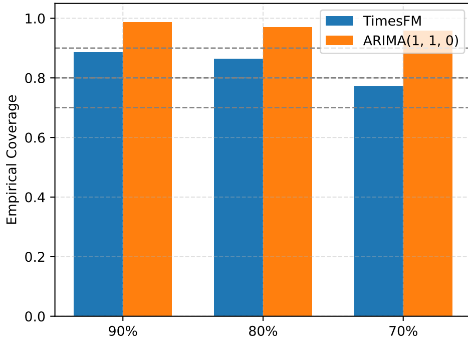
VERSIONED AR Coverage
