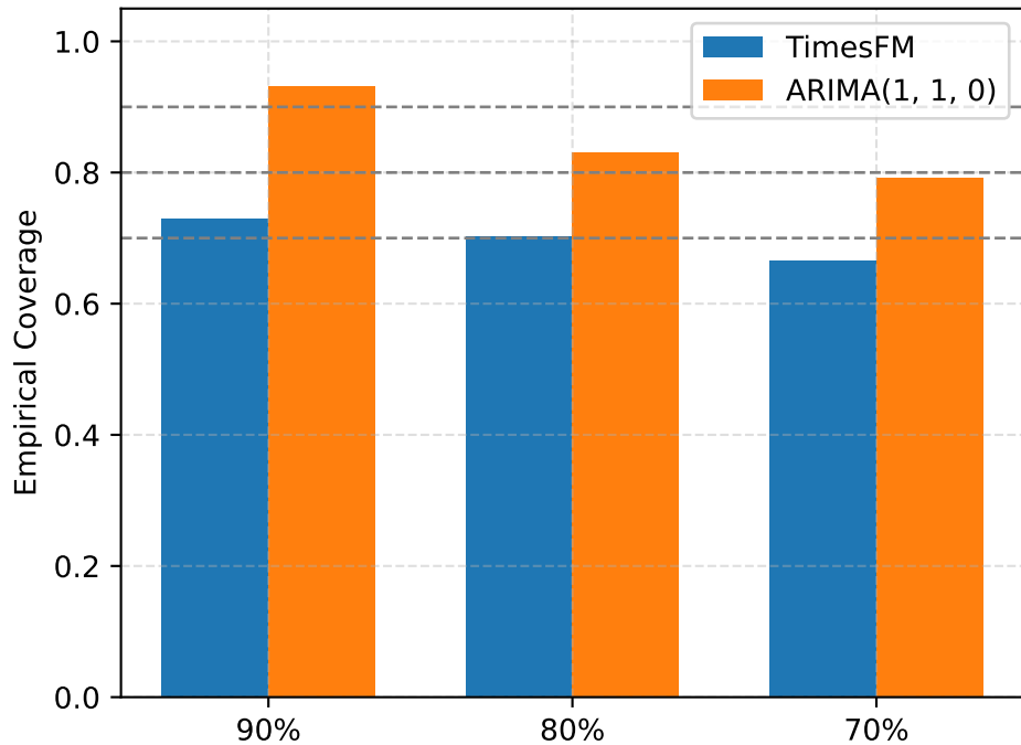
VERSIONED IL Coverage
