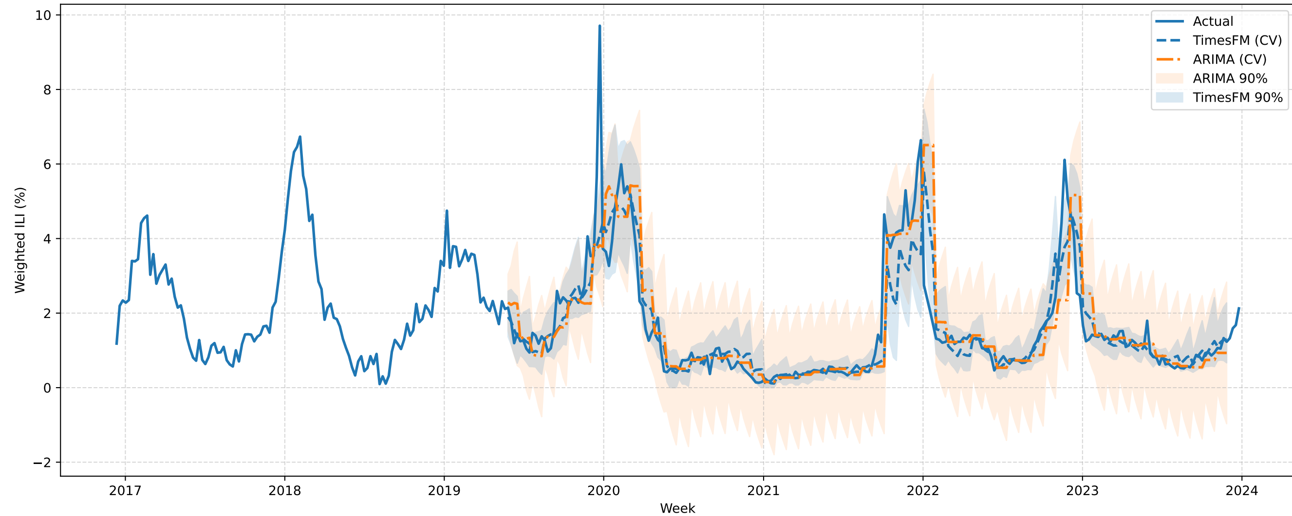
FINALIZED MN Expanding-Window CV (h=4): TimesFM vs ARIMA (best order)
