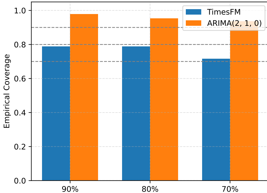
VERSIONED GA Coverage
