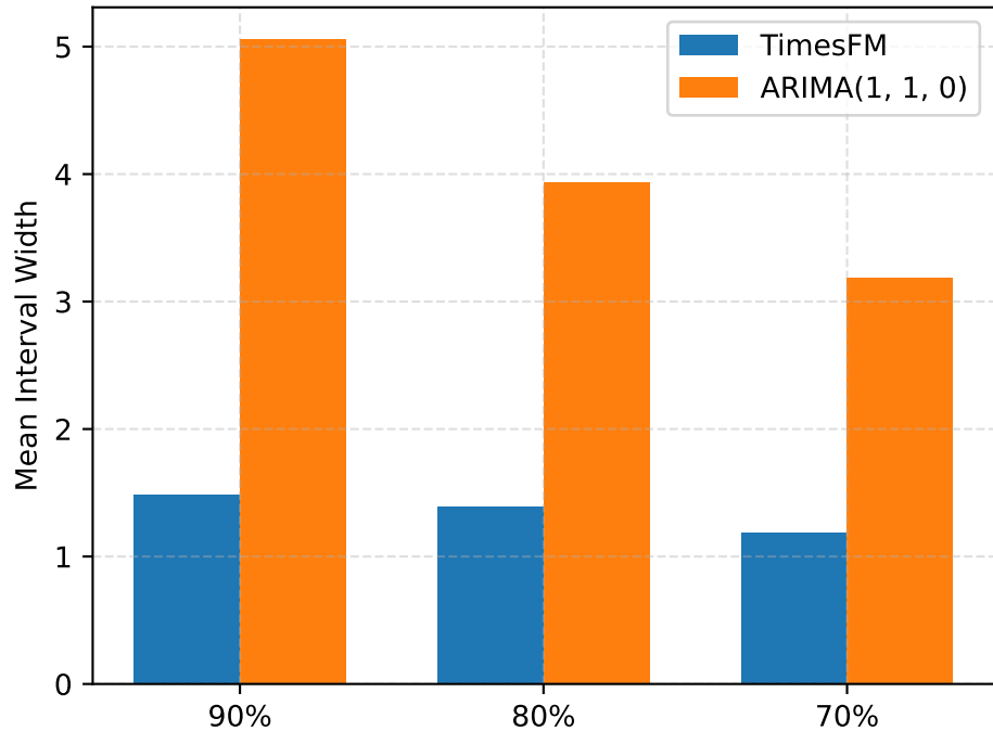
VERSIONED AR Width
