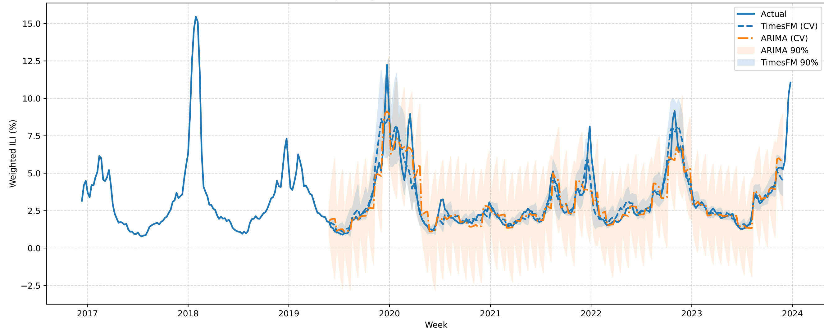
VERSIONED GA Expanding-Window CV (h=4): TimesFM vs ARIMA (best order)
