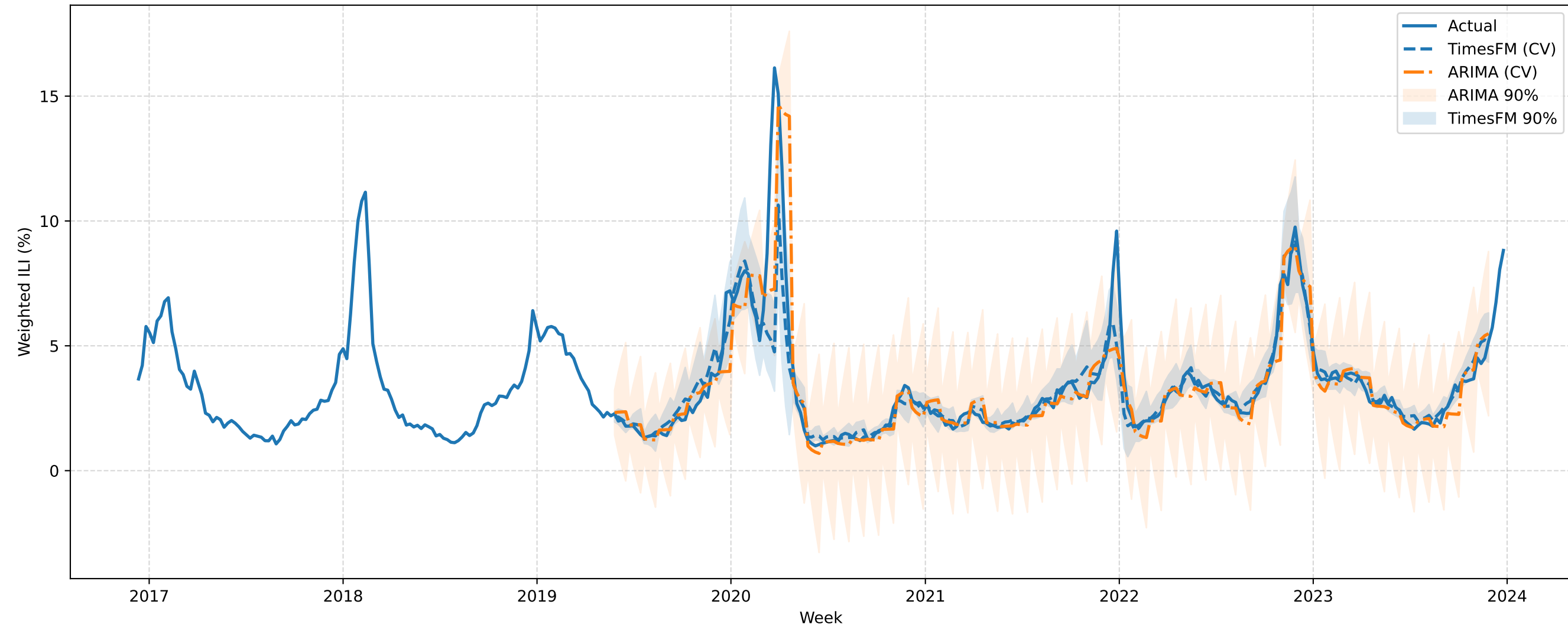
VERSIONED NJ Expanding-Window CV (h=4): TimesFM vs ARIMA (best order)
