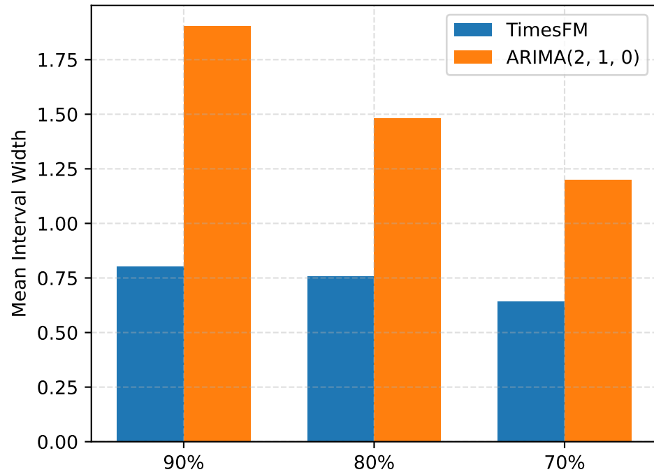
FINALIZED ME Width
