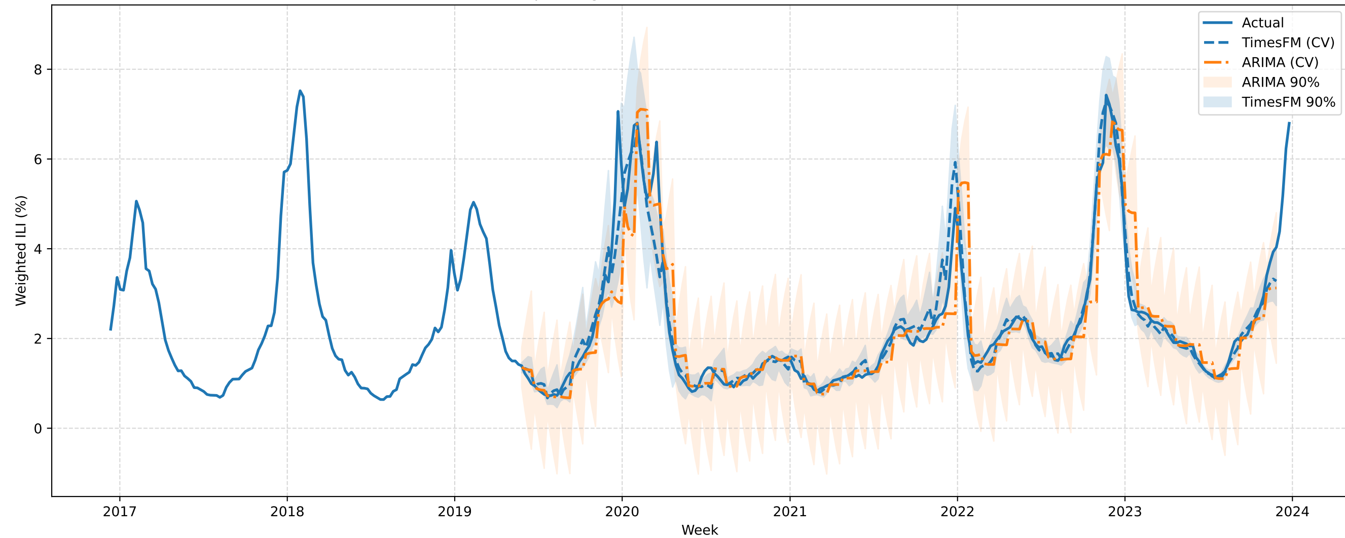
FINALIZED NAT Expanding-Window CV (h=4): TimesFM vs ARIMA (best order)
