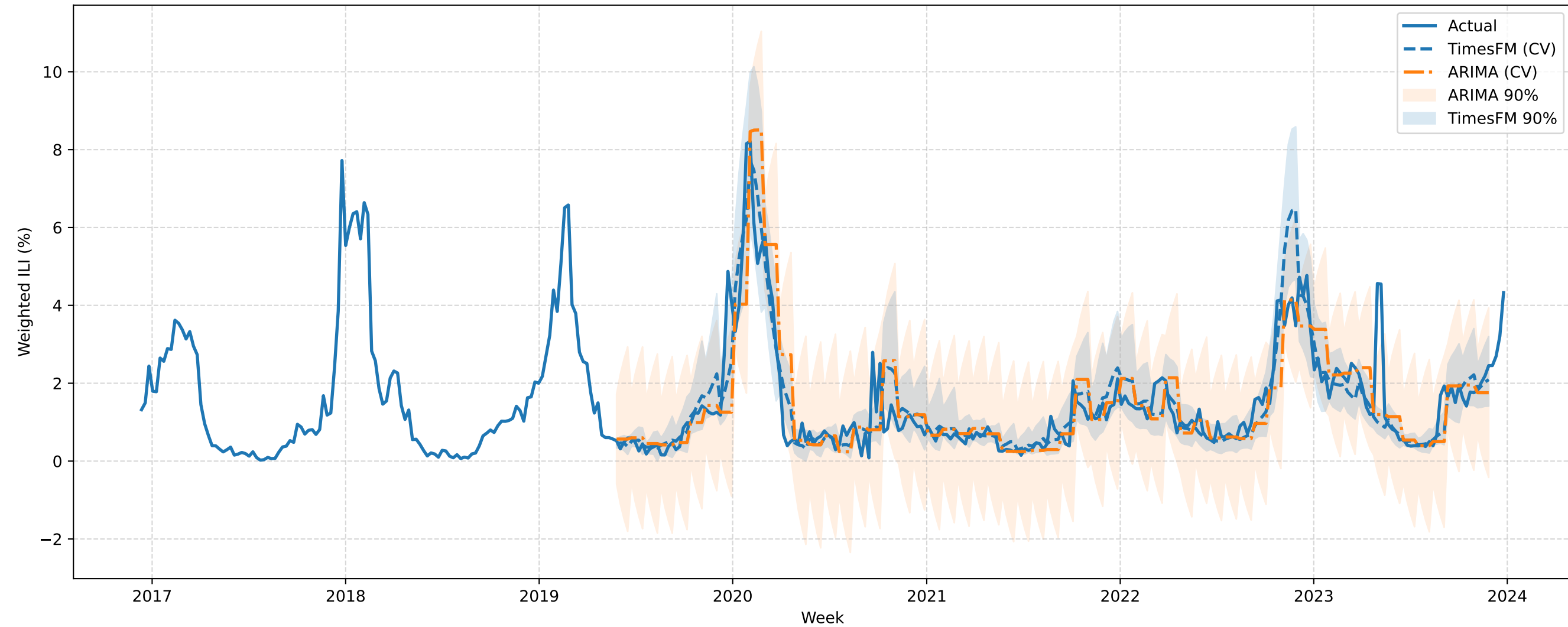
FINALIZED WV Expanding-Window CV (h=4): TimesFM vs ARIMA (best order)
