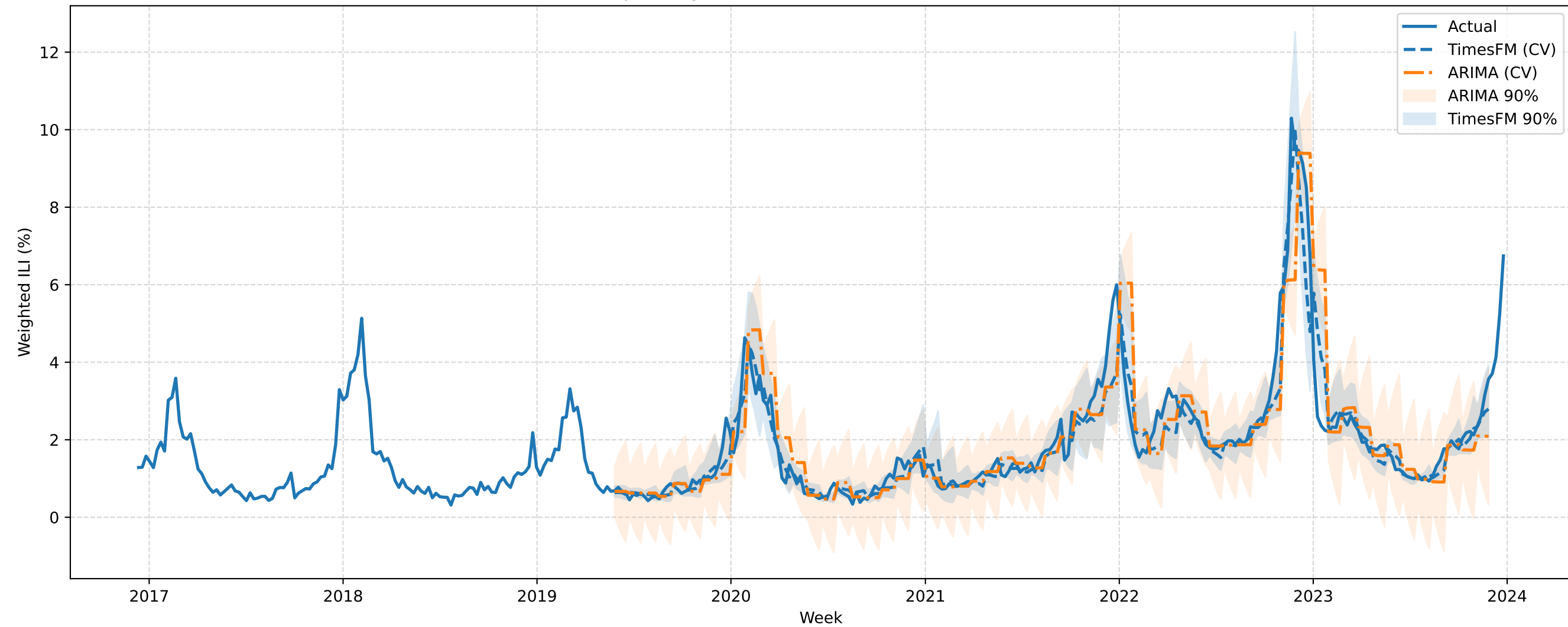
FINALIZED OH Expanding-Window CV (h=4): TimesFM vs ARIMA (best order)
