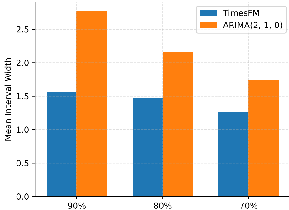
FINALIZED HI Width
