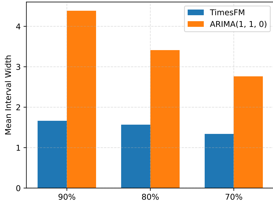
FINALIZED MS Width
