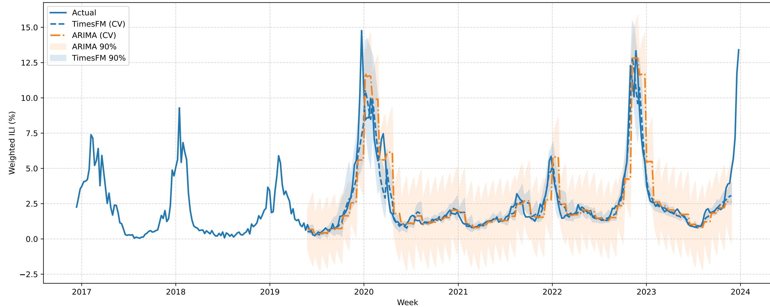
FINALIZED TN Expanding-Window CV (h=4): TimesFM vs ARIMA (best order)
