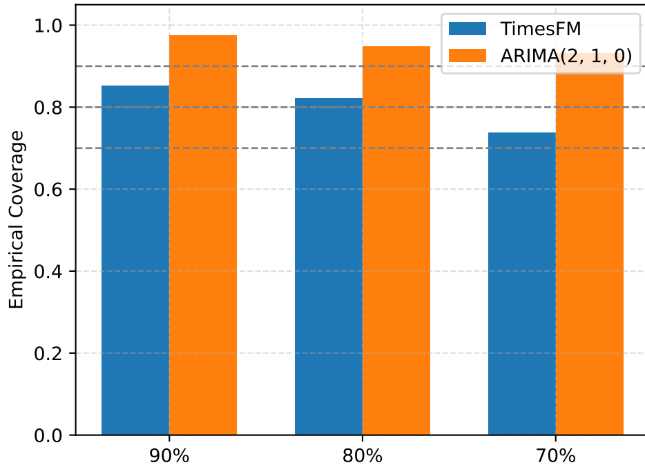
VERSIONED SC Coverage
