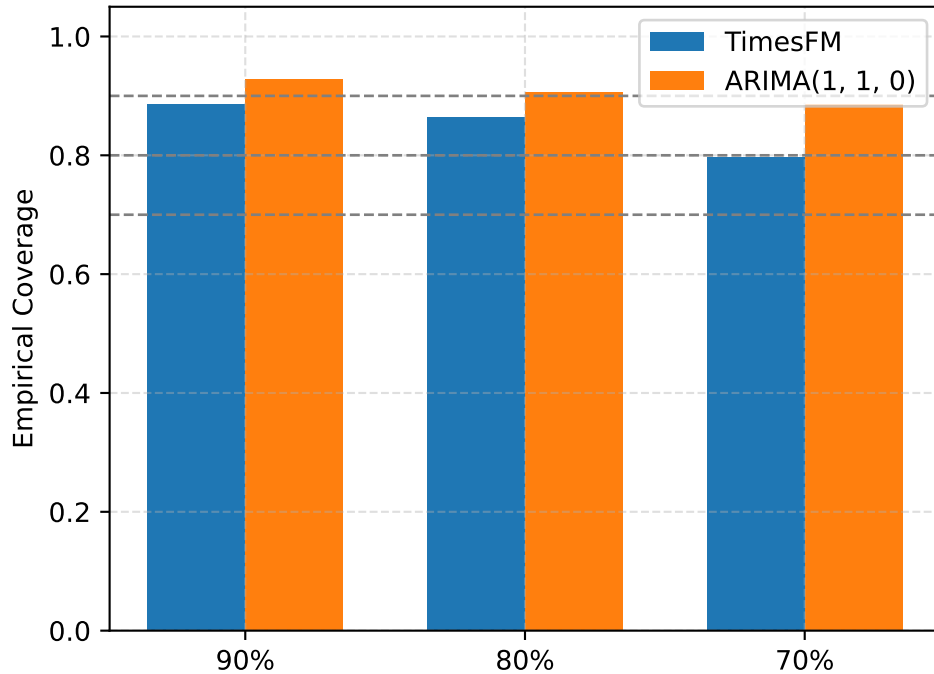
VERSIONED OK Coverage
