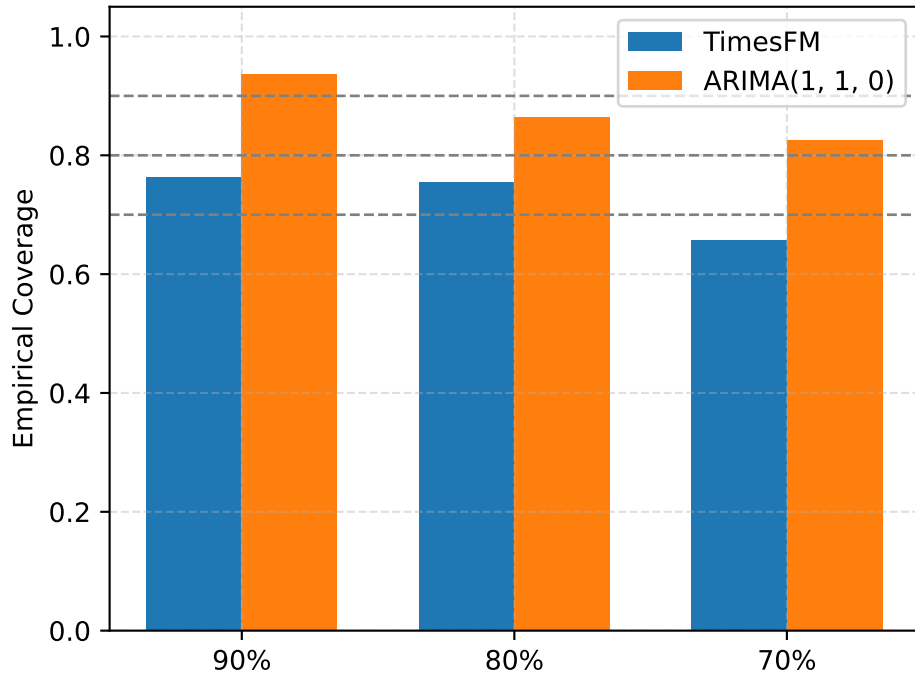
VERSIONED CA Coverage
