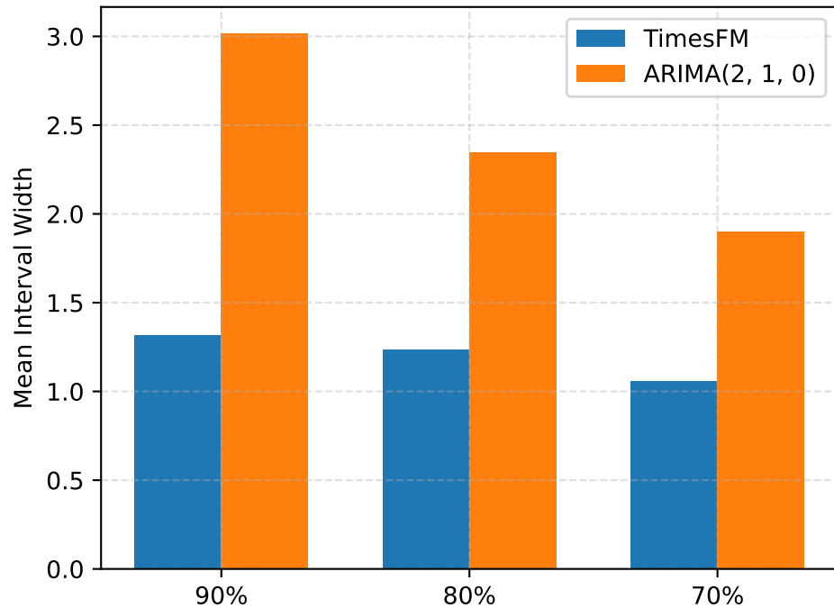
FINALIZED MN Width
