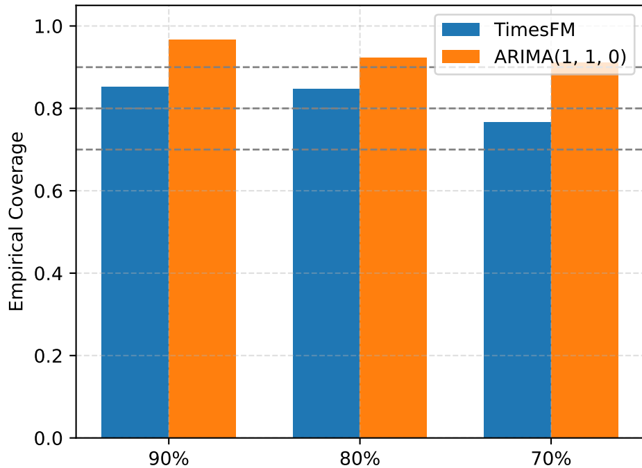
VERSIONED PA Coverage
