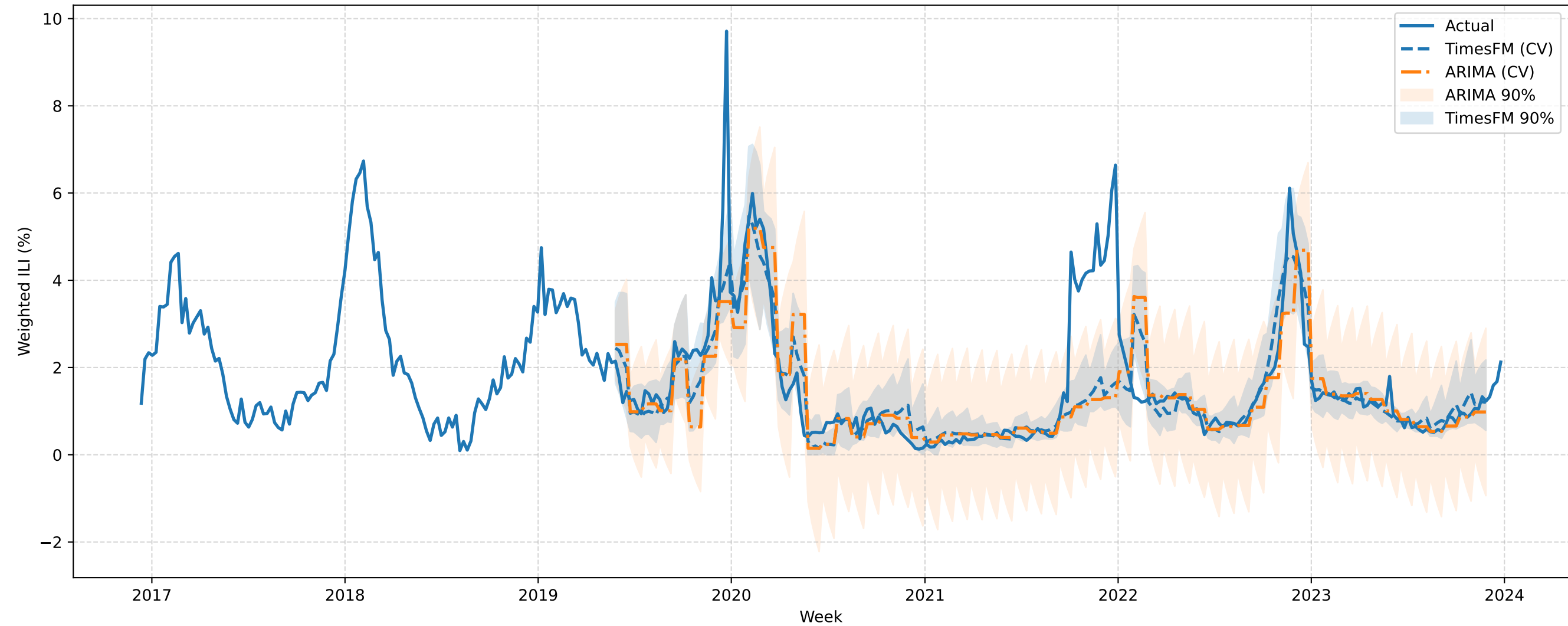
VERSIONED MN Expanding-Window CV (h=4): TimesFM vs ARIMA (best order)
