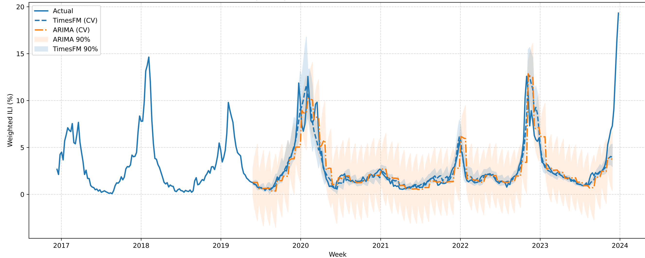
FINALIZED SC Expanding-Window CV (h=4): TimesFM vs ARIMA (best order)
