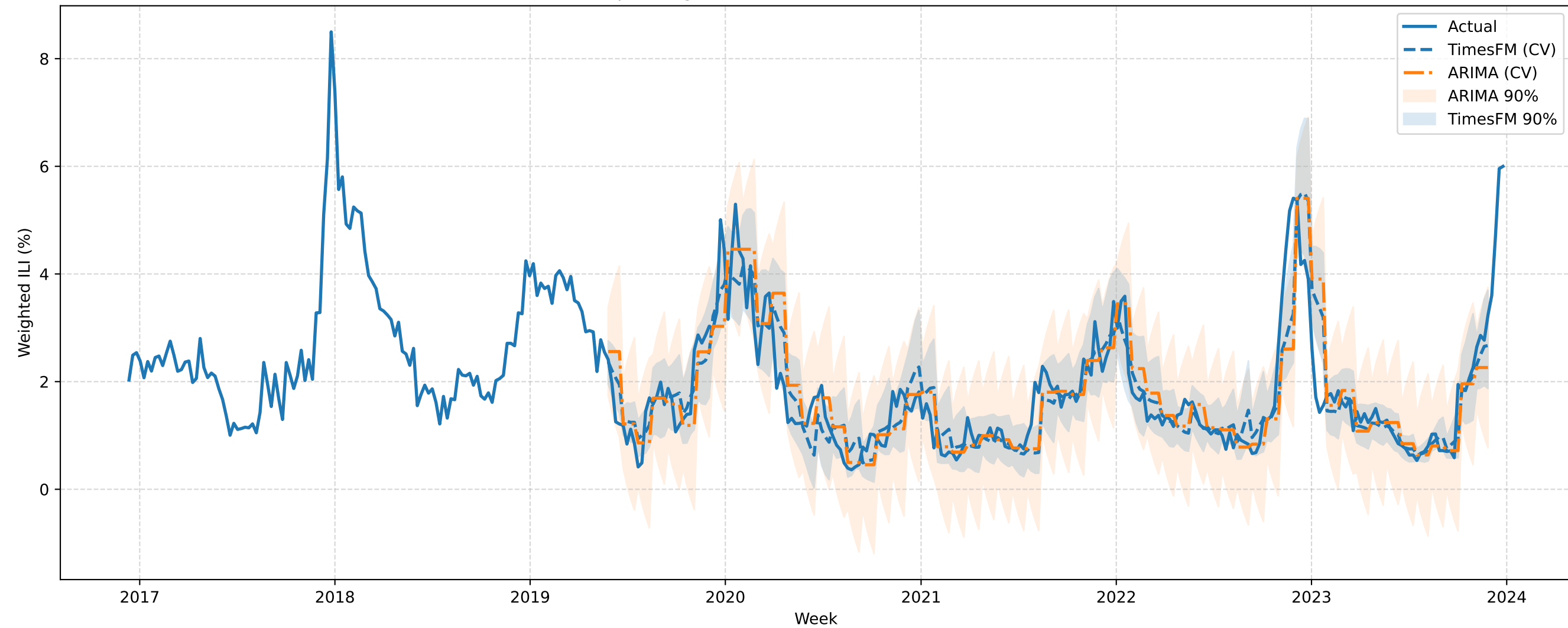
FINALIZED AZ Expanding-Window CV (h=4): TimesFM vs ARIMA (best order)
