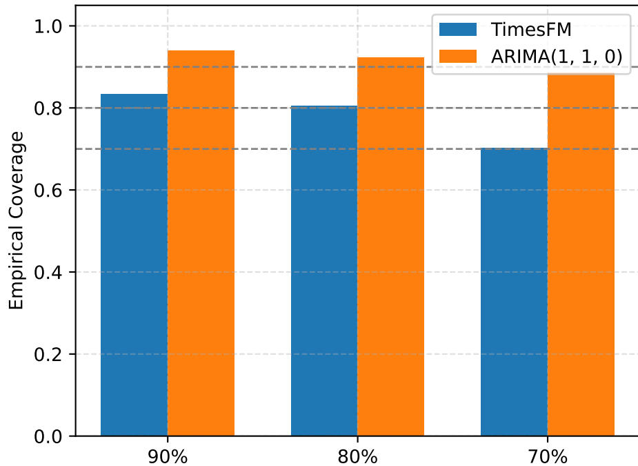
FINALIZED NC Coverage
