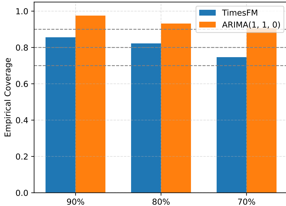
VERSIONED TX Coverage
