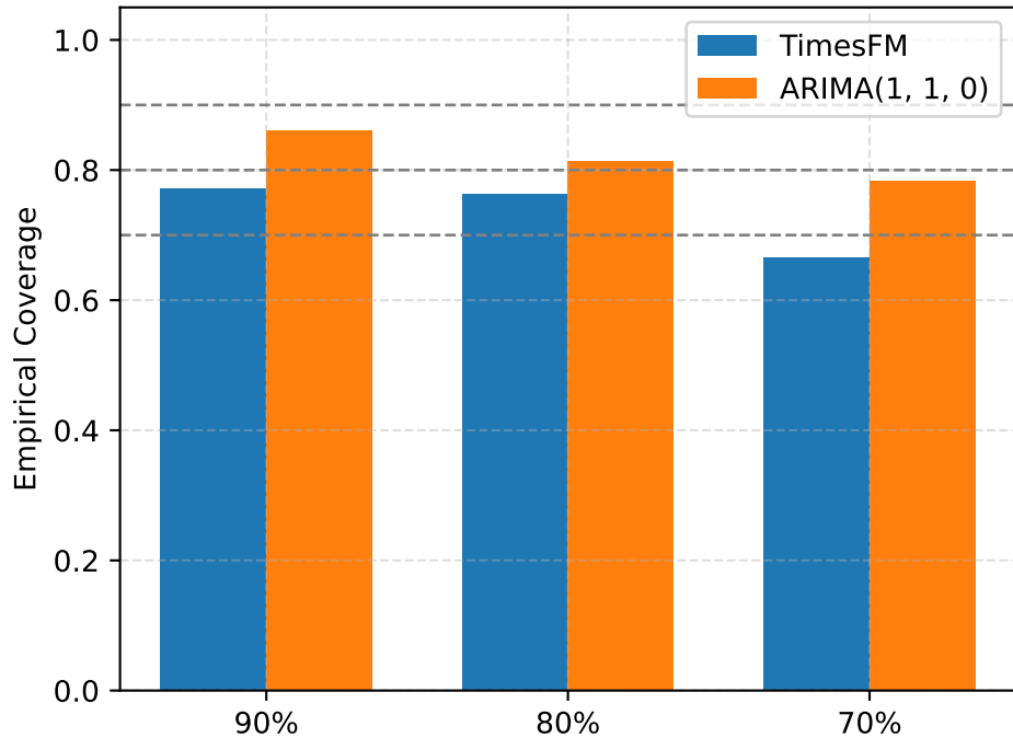
FINALIZED WY Coverage
