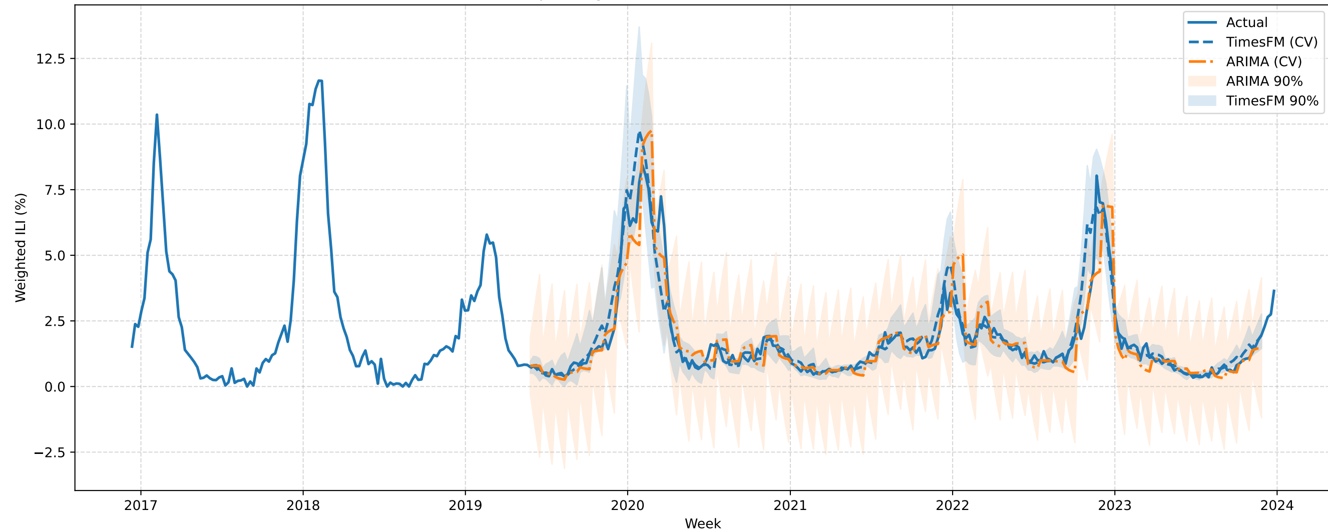
VERSIONED KS Expanding-Window CV (h=4): TimesFM vs ARIMA (best order)
