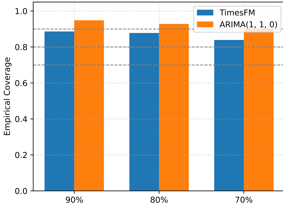
VERSIONED TN Coverage
