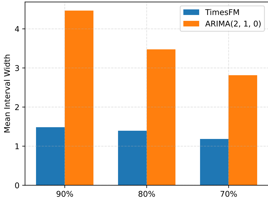
FINALIZED NJ Width
