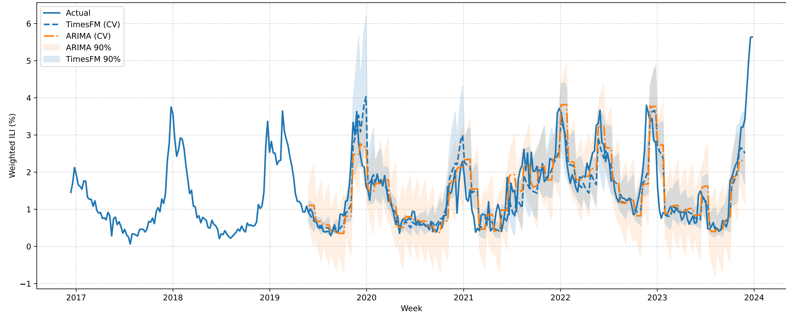
FINALIZED NV Expanding-Window CV (h=4): TimesFM vs ARIMA (best order)
