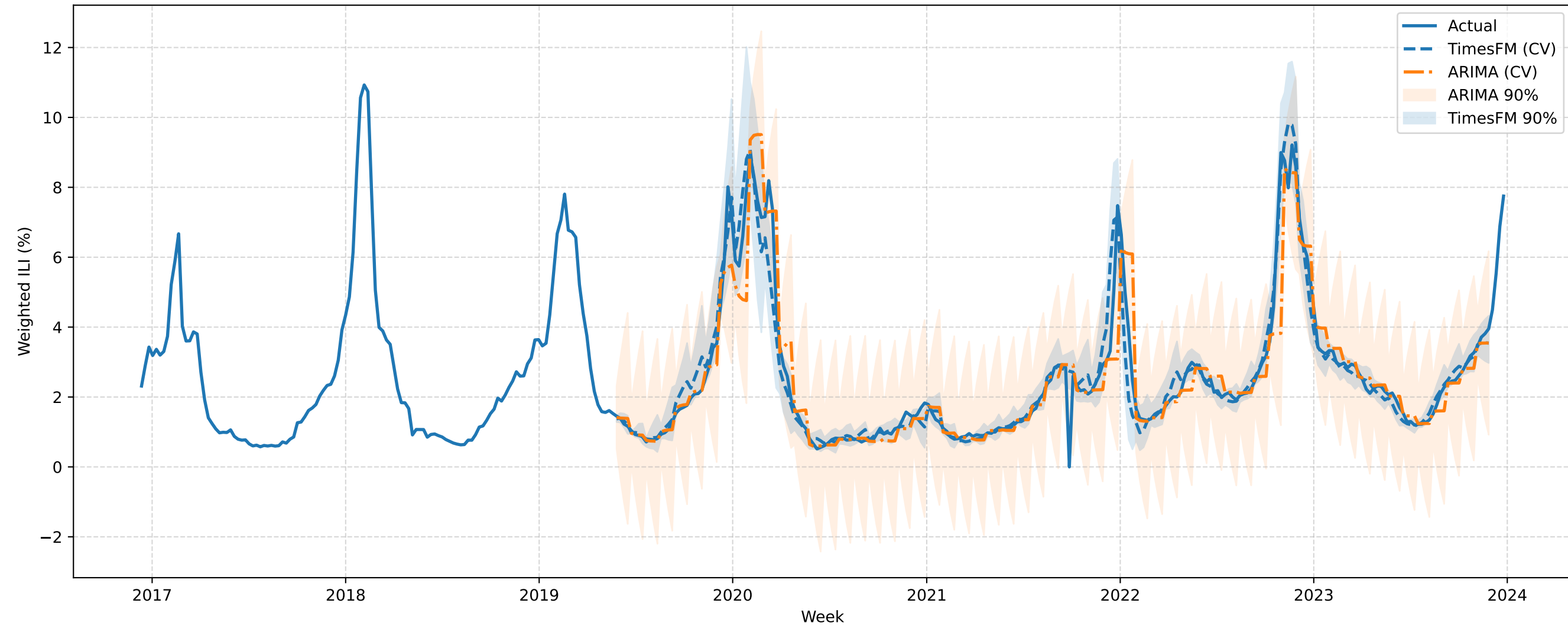
VERSIONED VA Expanding-Window CV (h=4): TimesFM vs ARIMA (best order)
