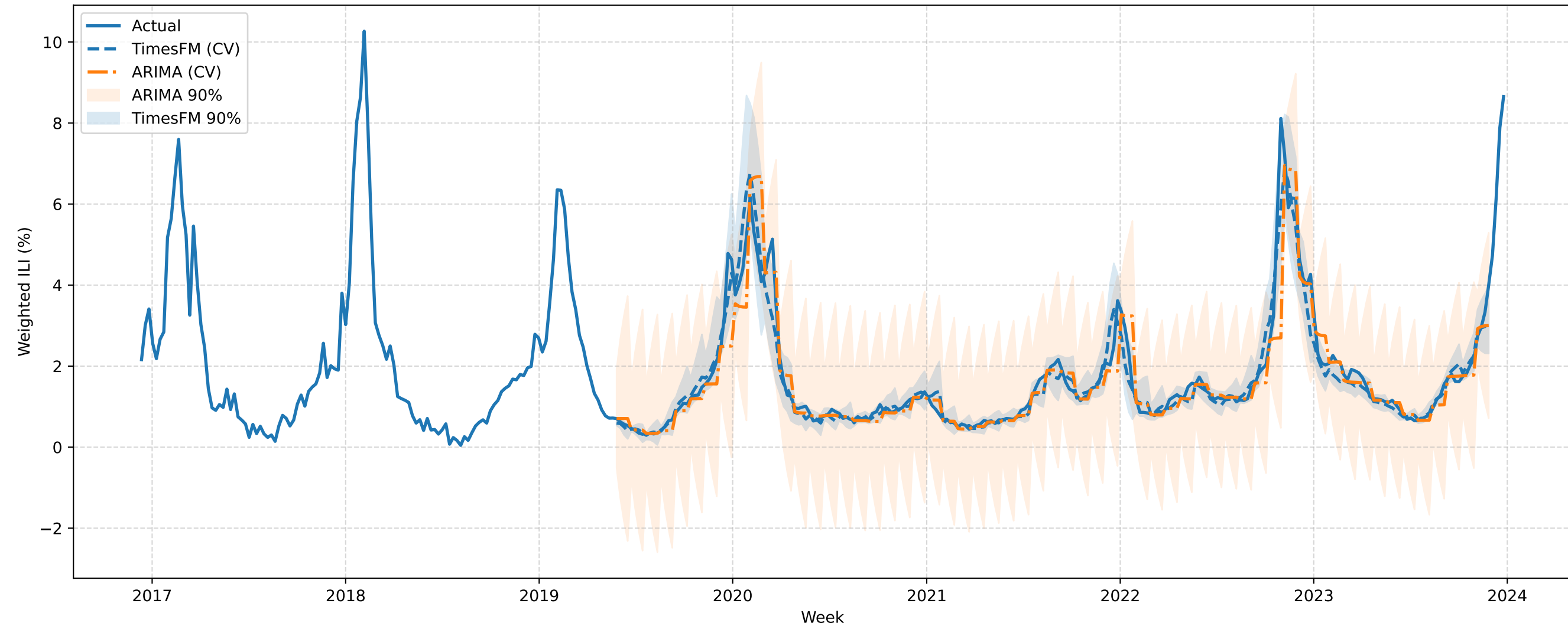
VERSIONED NC Expanding-Window CV (h=4): TimesFM vs ARIMA (best order)
