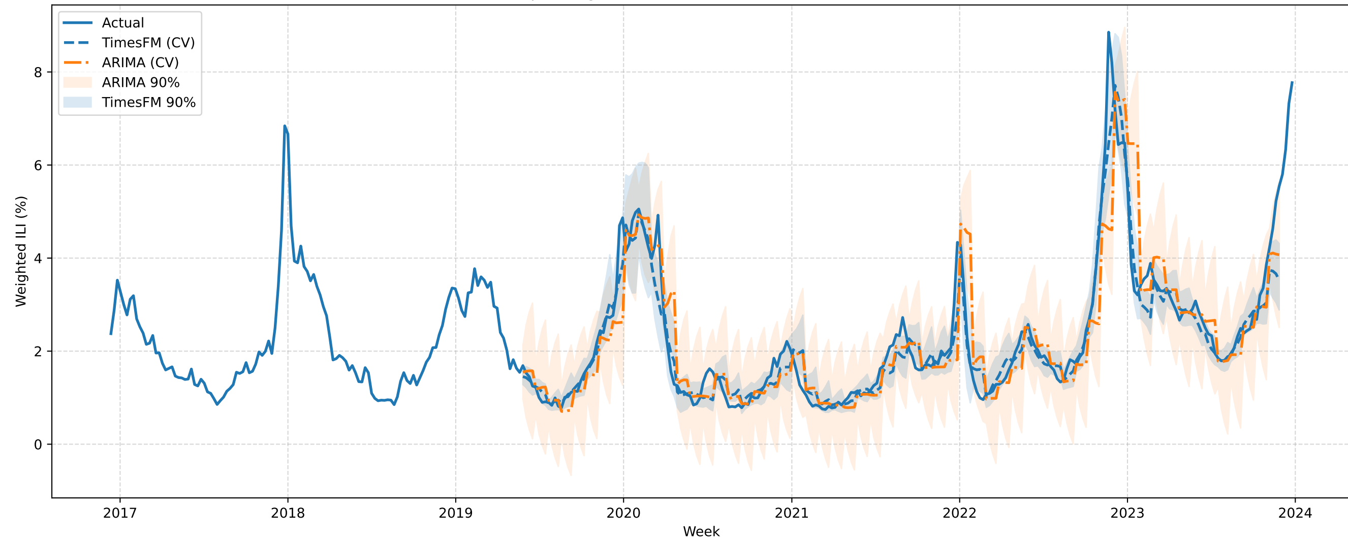
FINALIZED CA Expanding-Window CV (h=4): TimesFM vs ARIMA (best order)
