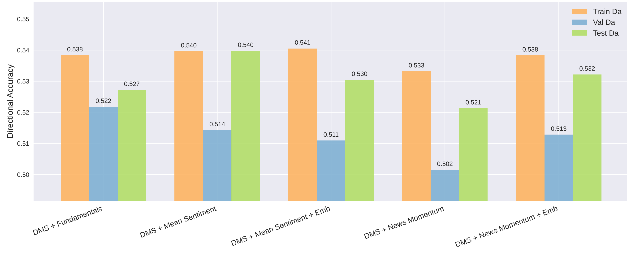
Model Performance Comparison (Train / Validation / Test)
