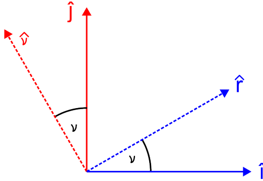
Figure 5.1: Position and unit vectors in plane polar coordinates
