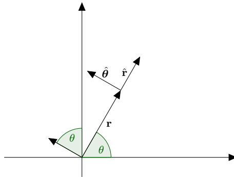
Figure 2.1: Position and unit vectors in plane polar coordinates
