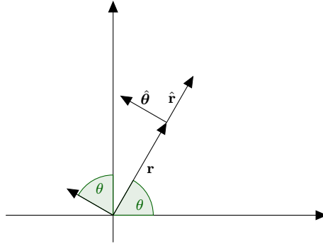
Figure 5.1: Position and unit vectors in plane polar coordinates
