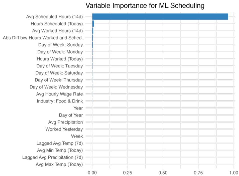
Figure 14: Feature Importance: ML model
