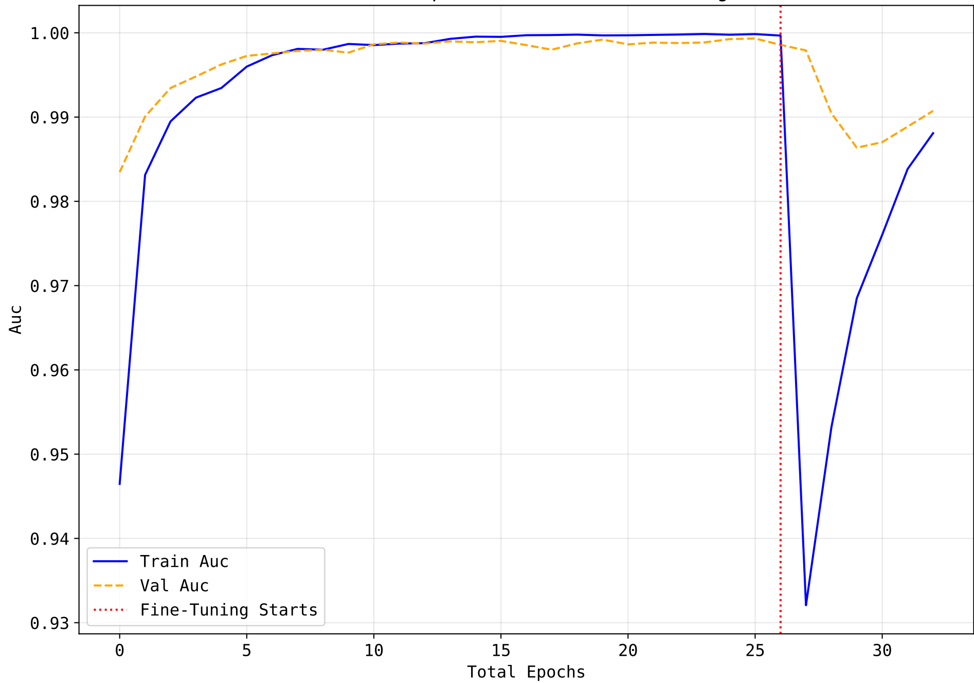
Auc Over Epochs (Two-Phase Training)
