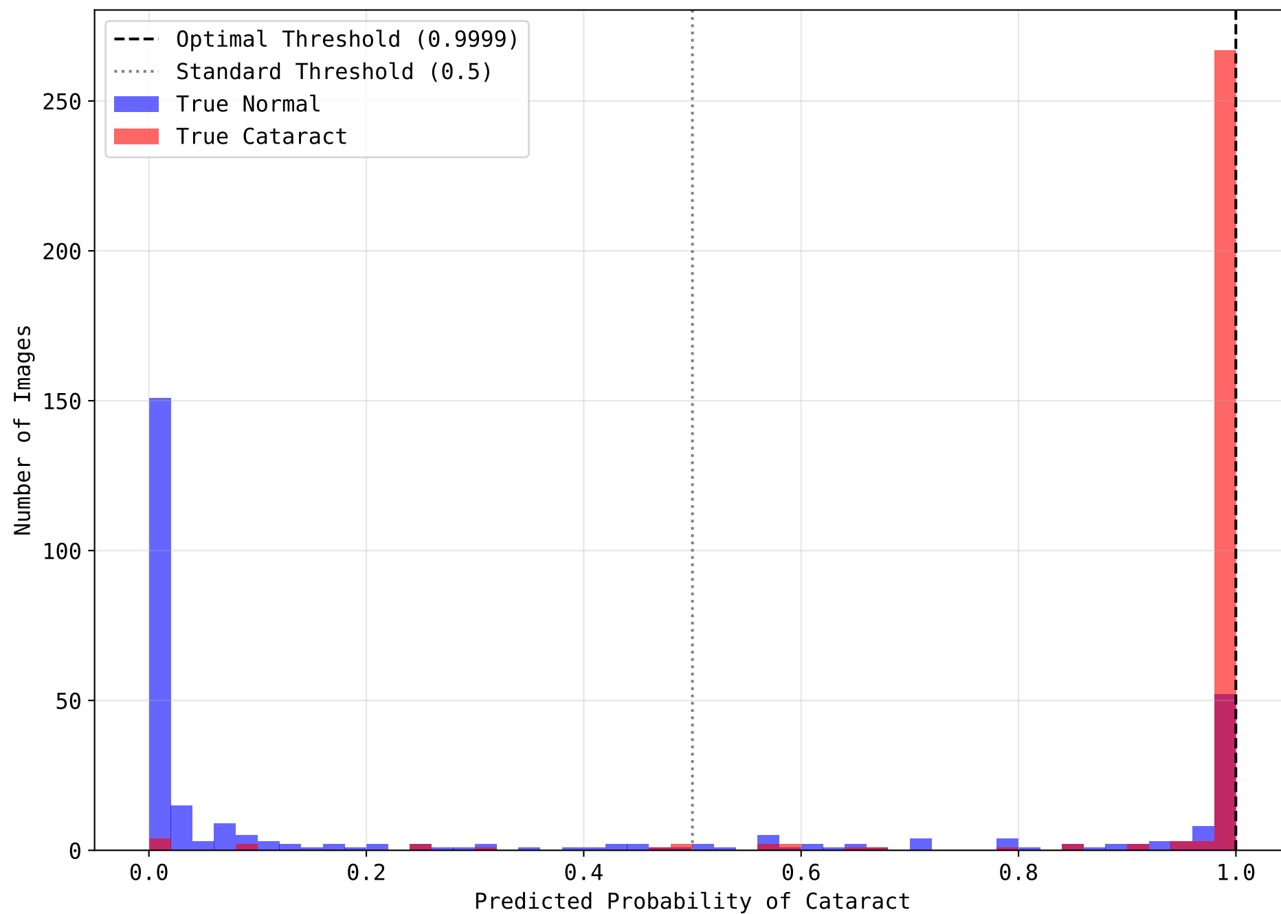
DenseNet121 - Distribution of Predicted Probabilities
