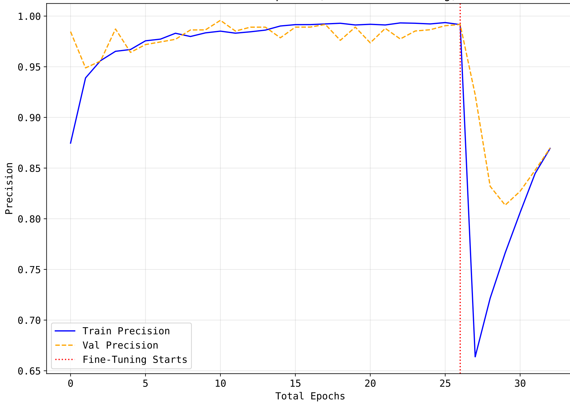
Precision Over Epochs (Two-Phase Training)
