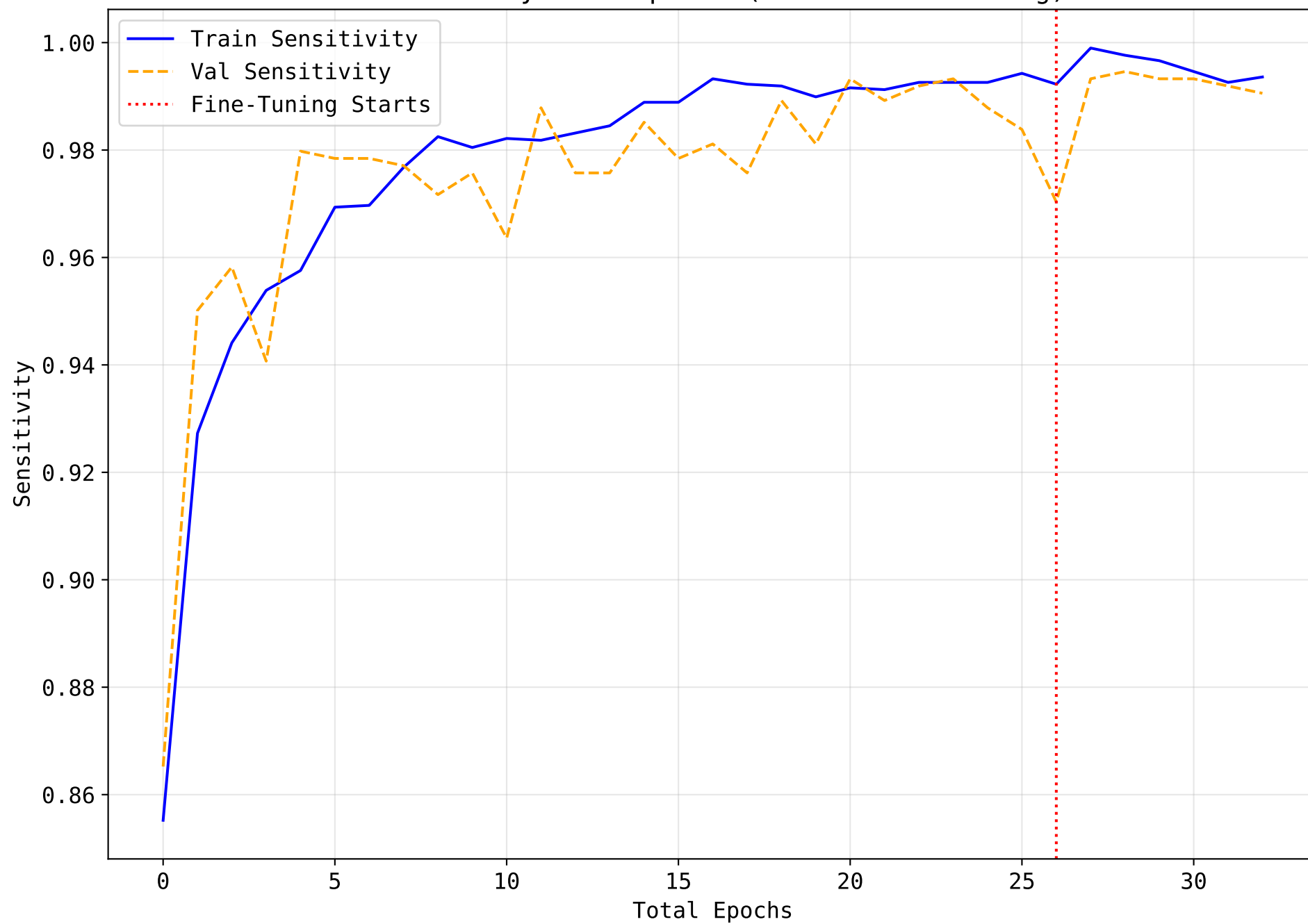
Sensitivity Over Epochs (Two-Phase Training)
