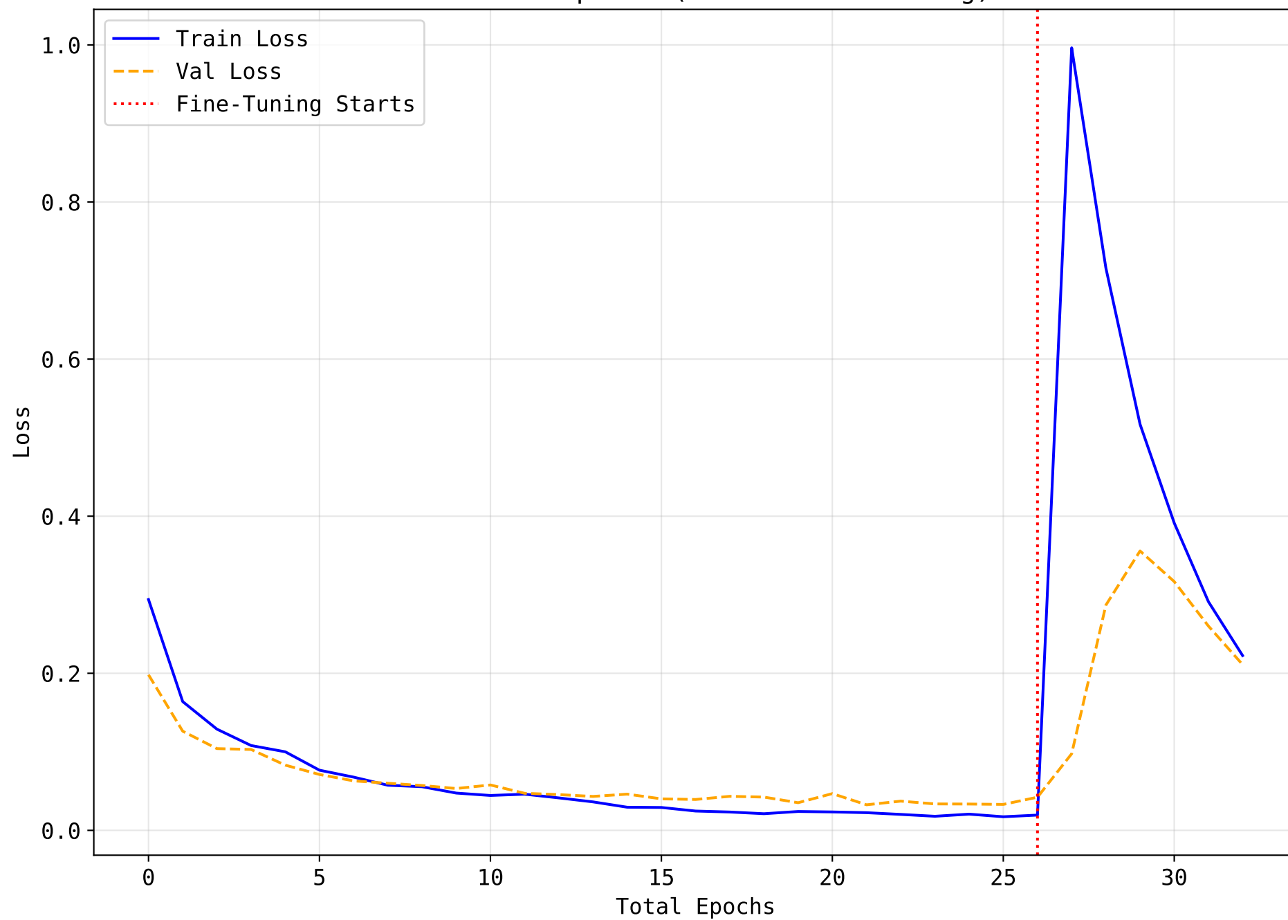
Loss Over Epochs (Two-Phase Training)
