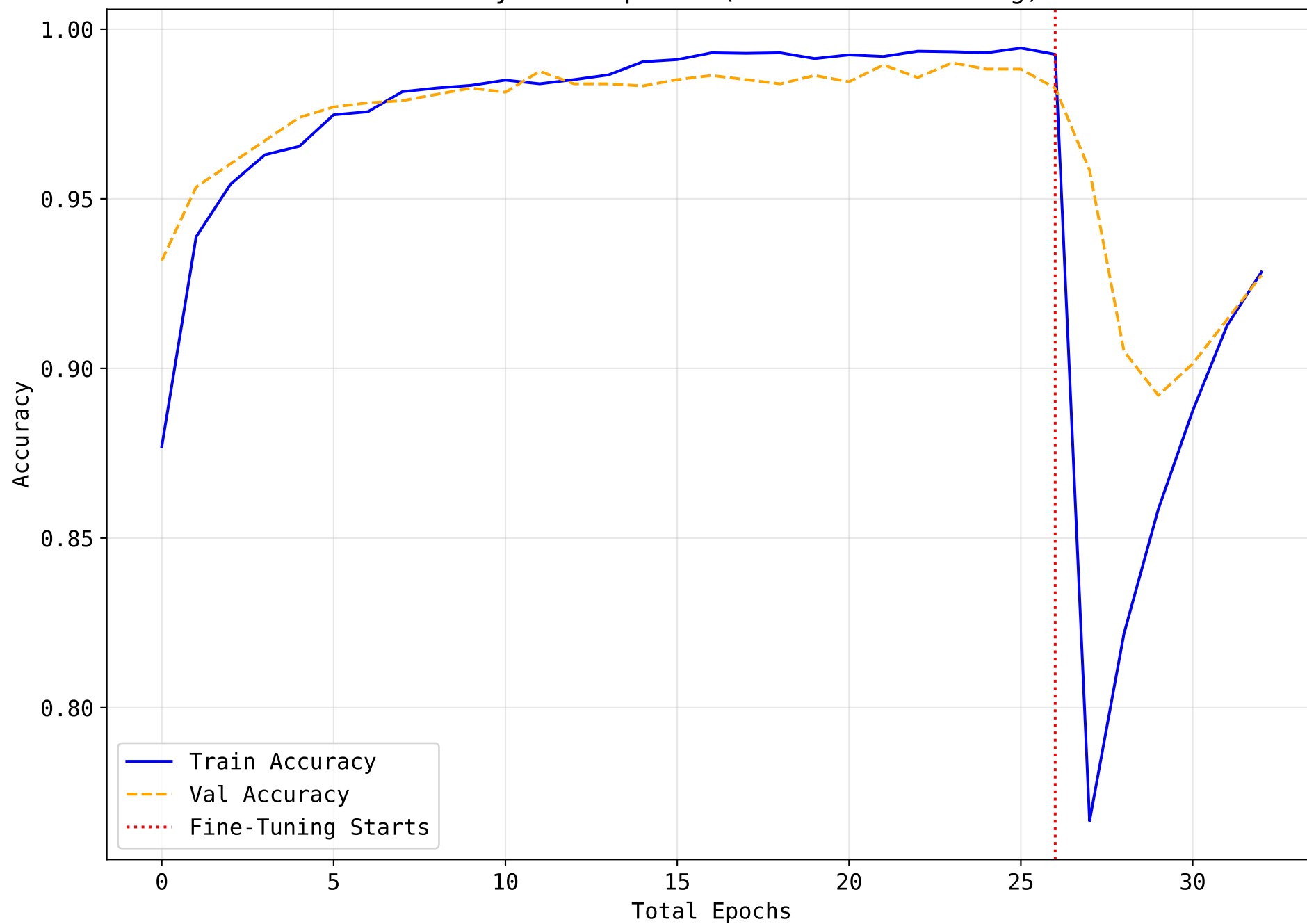
Accuracy Over Epochs (Two-Phase Training)
