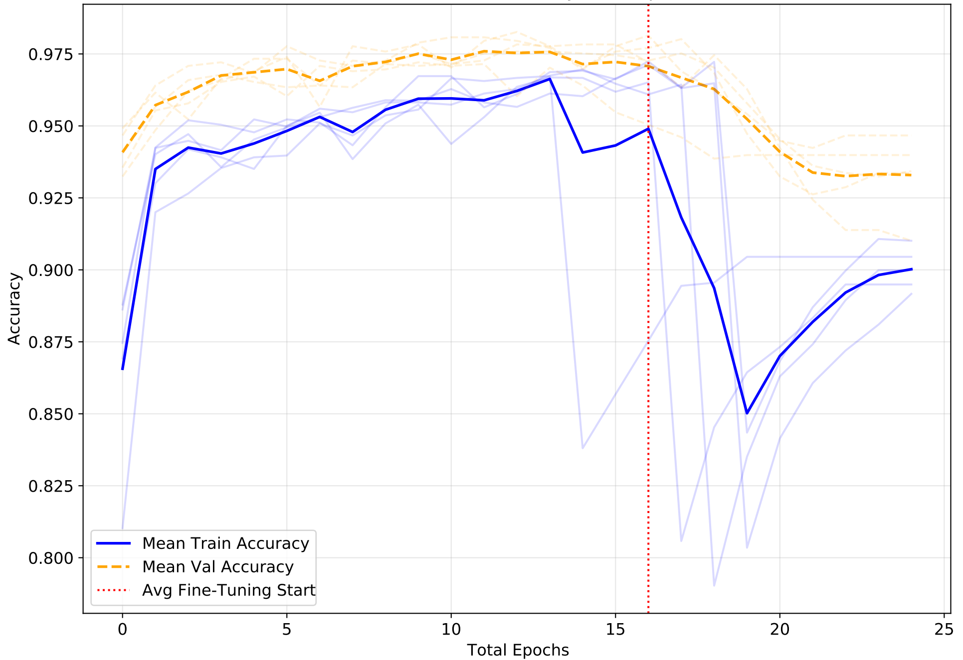
Cross-Validated Accuracy Over Epochs
