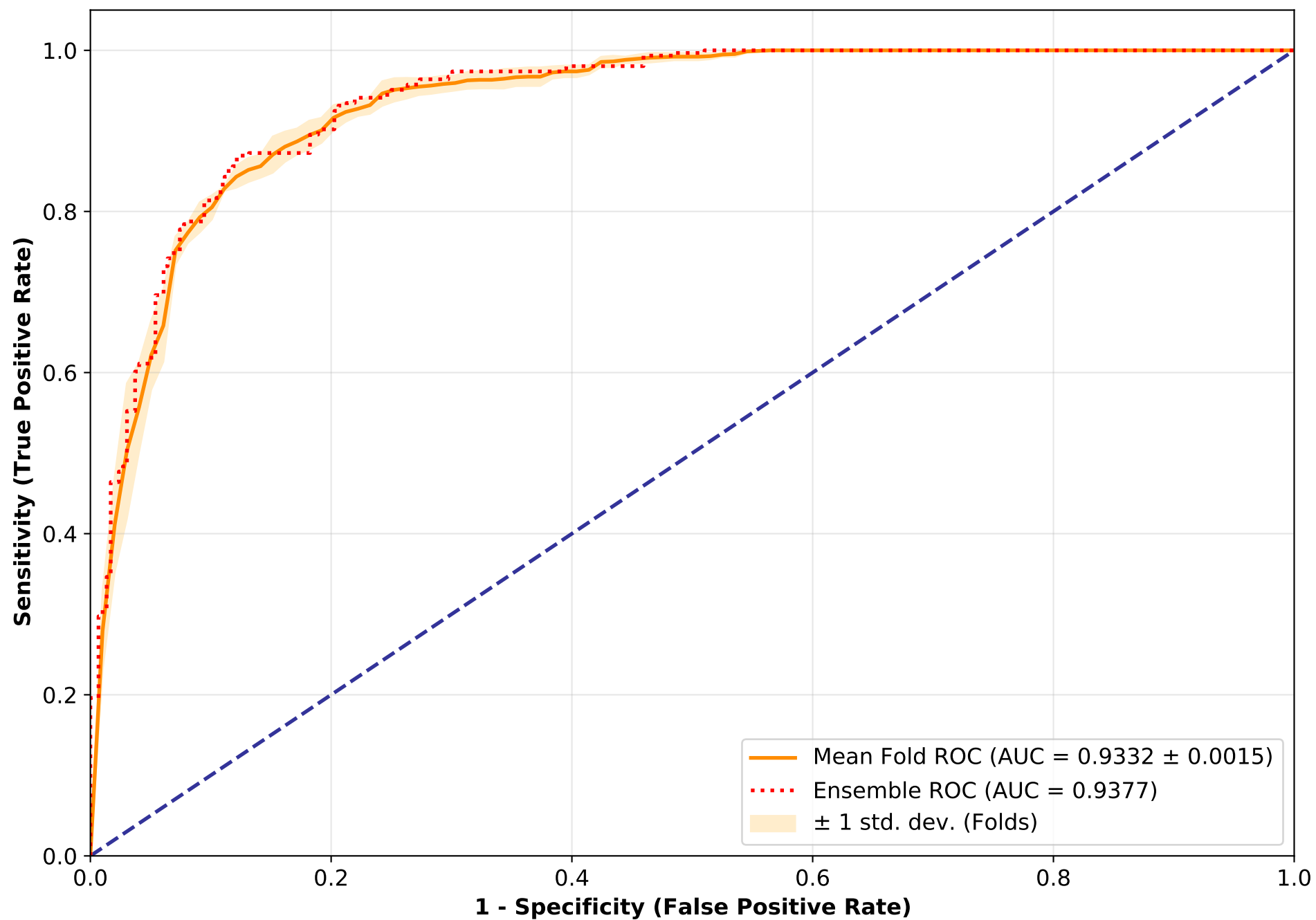
Cross-Validated ROC Curve - MobileNetV2
