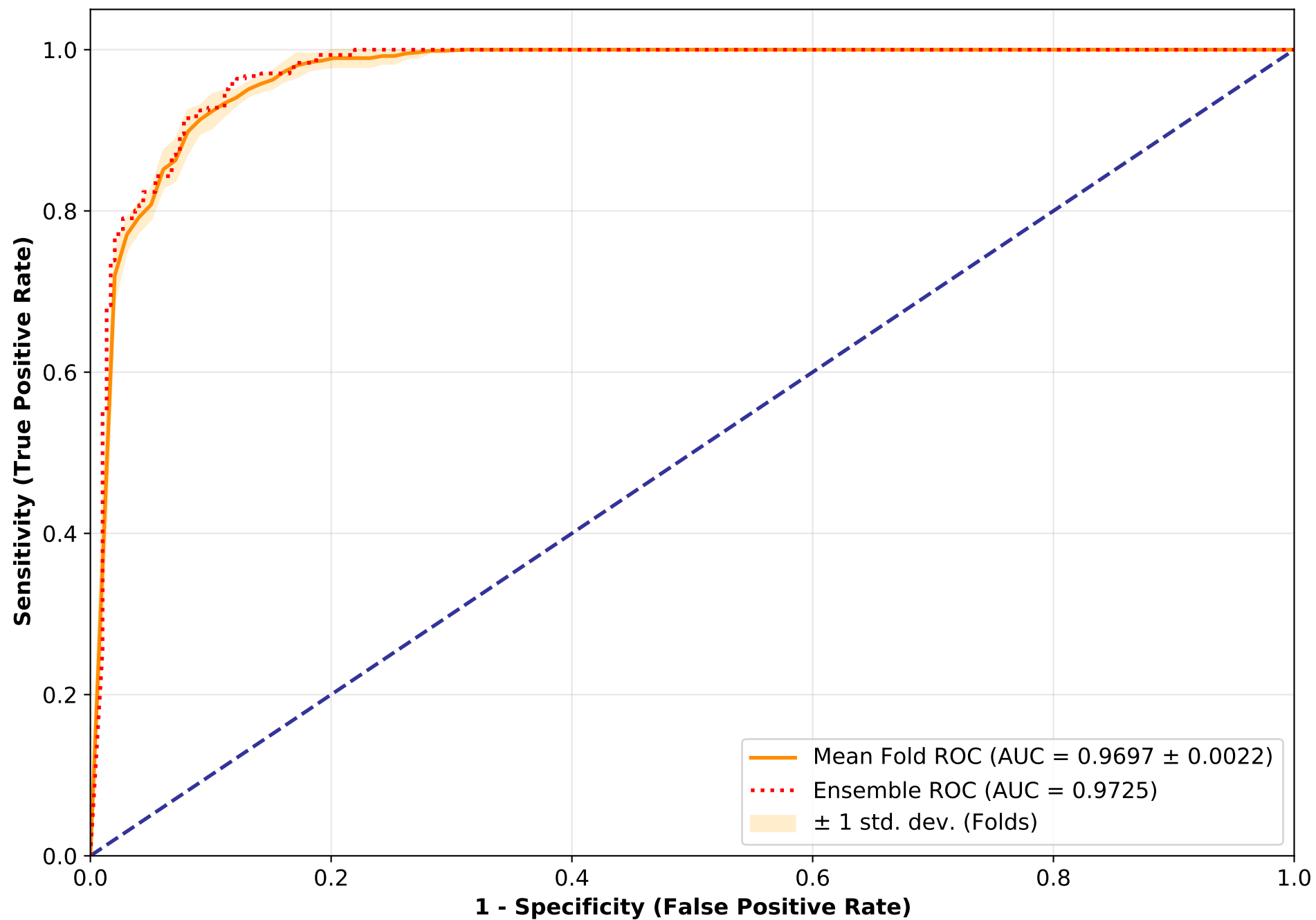
Cross-Validated ROC Curve - ResNet50
