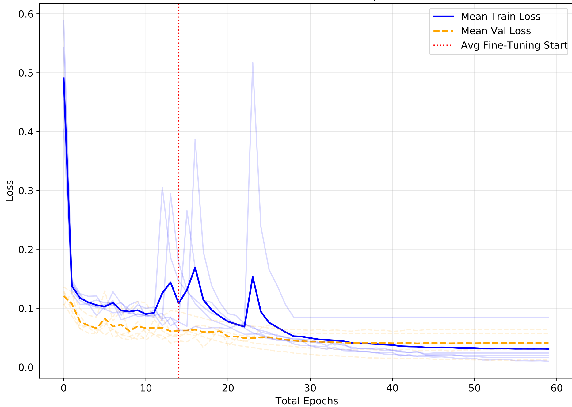
Cross-Validated Loss Over Epochs
