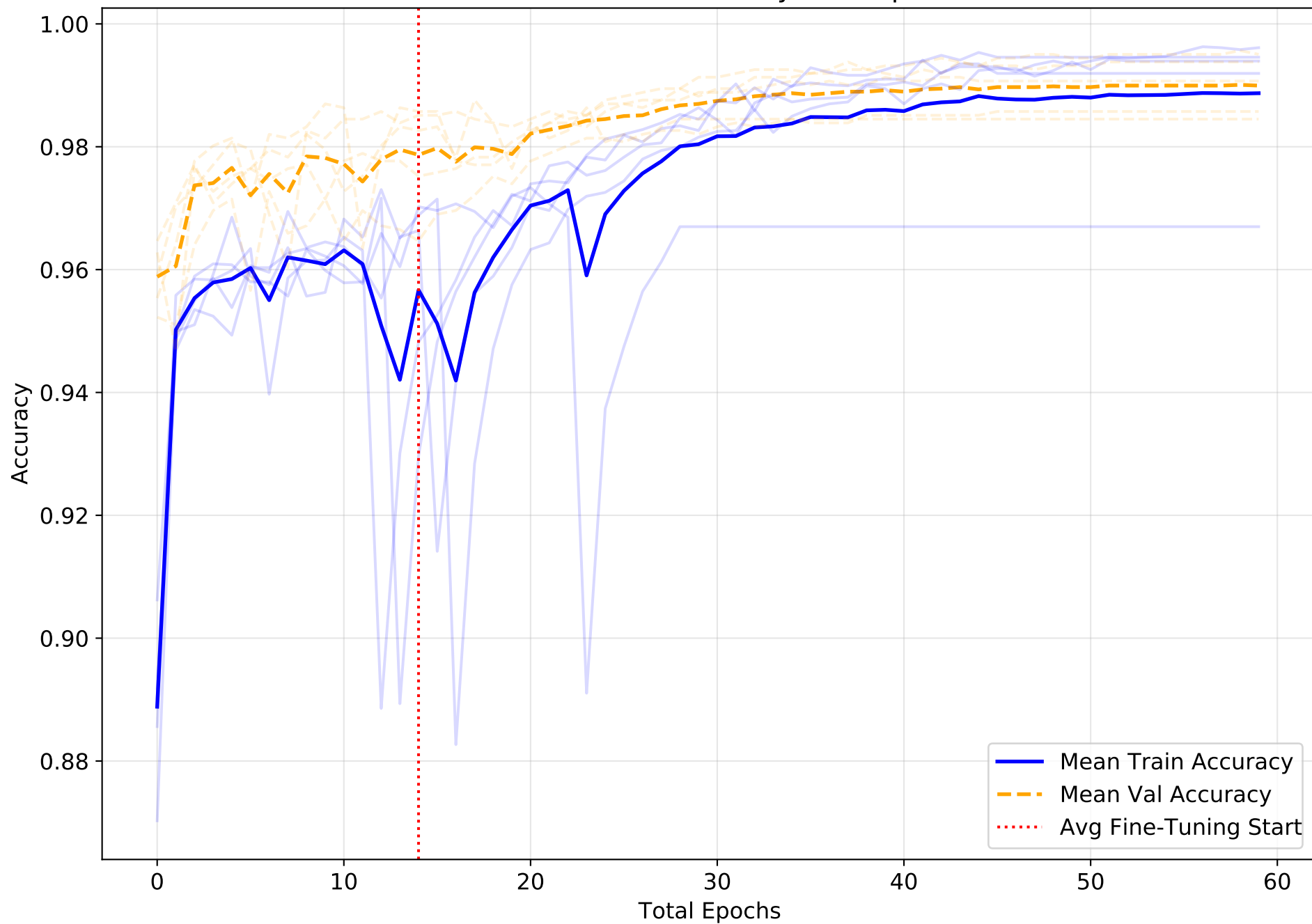
Cross-Validated Accuracy Over Epochs
