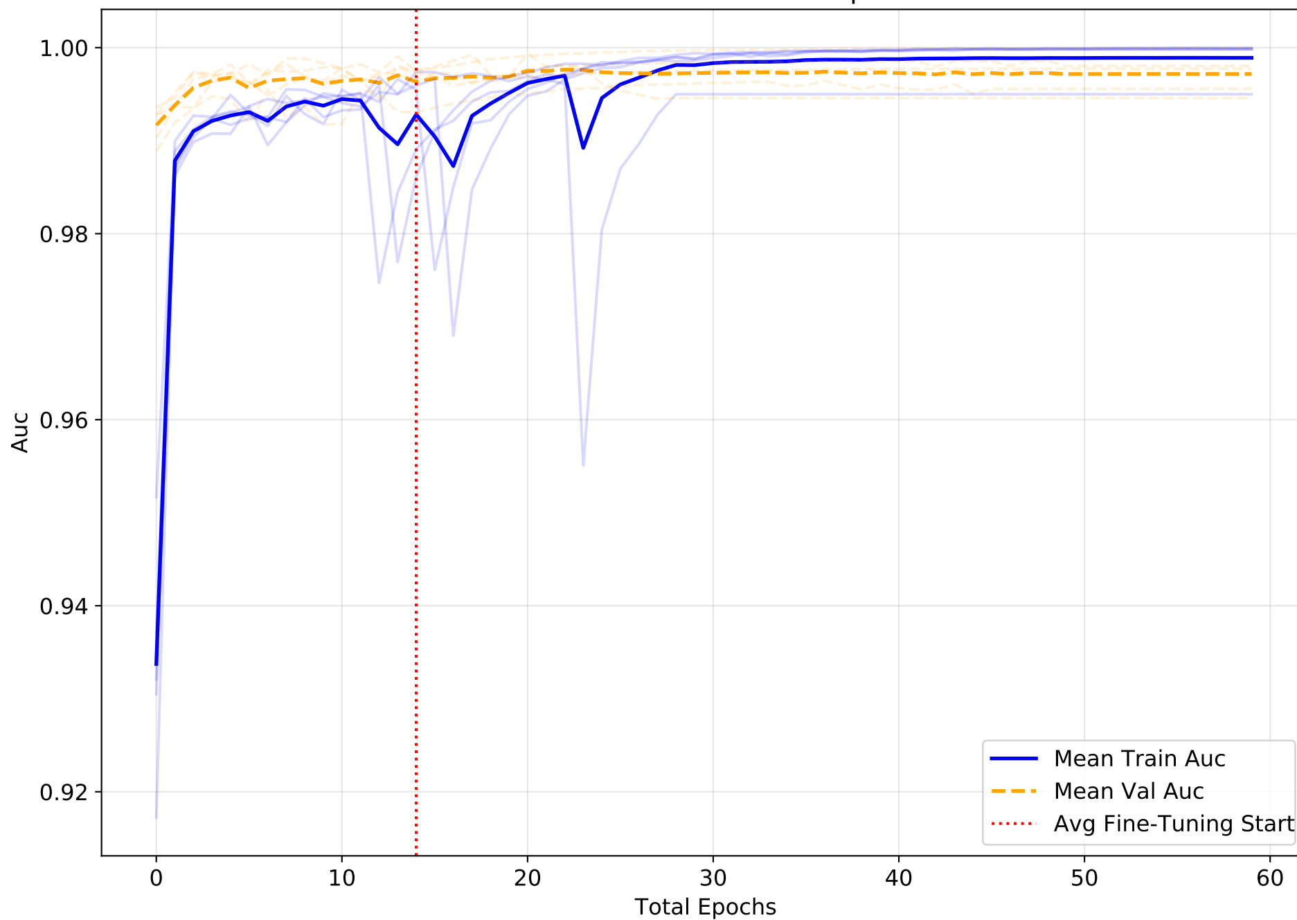
Cross-Validated Auc Over Epochs
