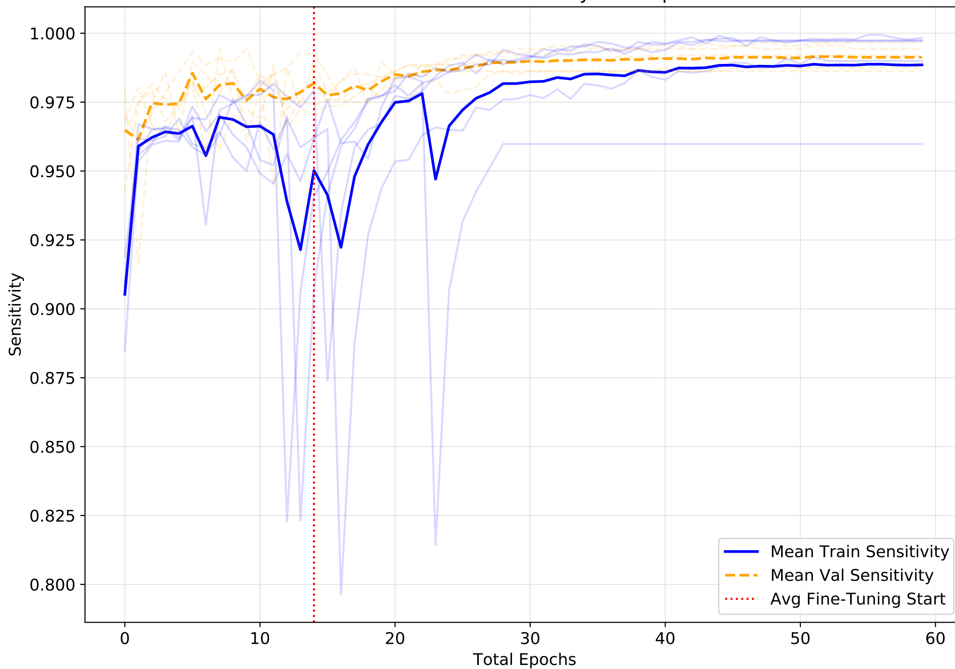
Cross-Validated Sensitivity Over Epochs
