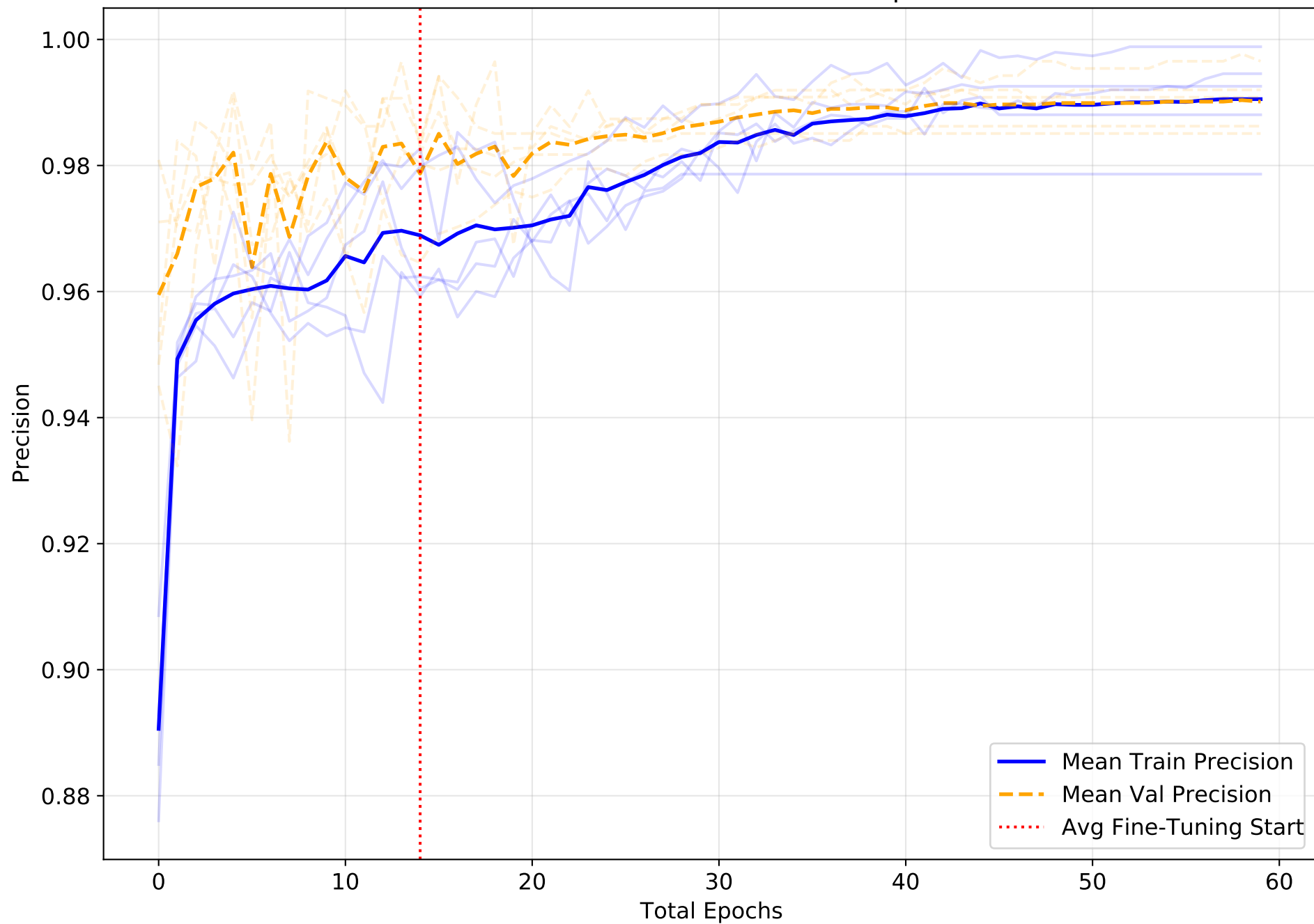
Cross-Validated Precision Over Epochs
