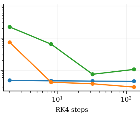
Rosenbrock — RK4
